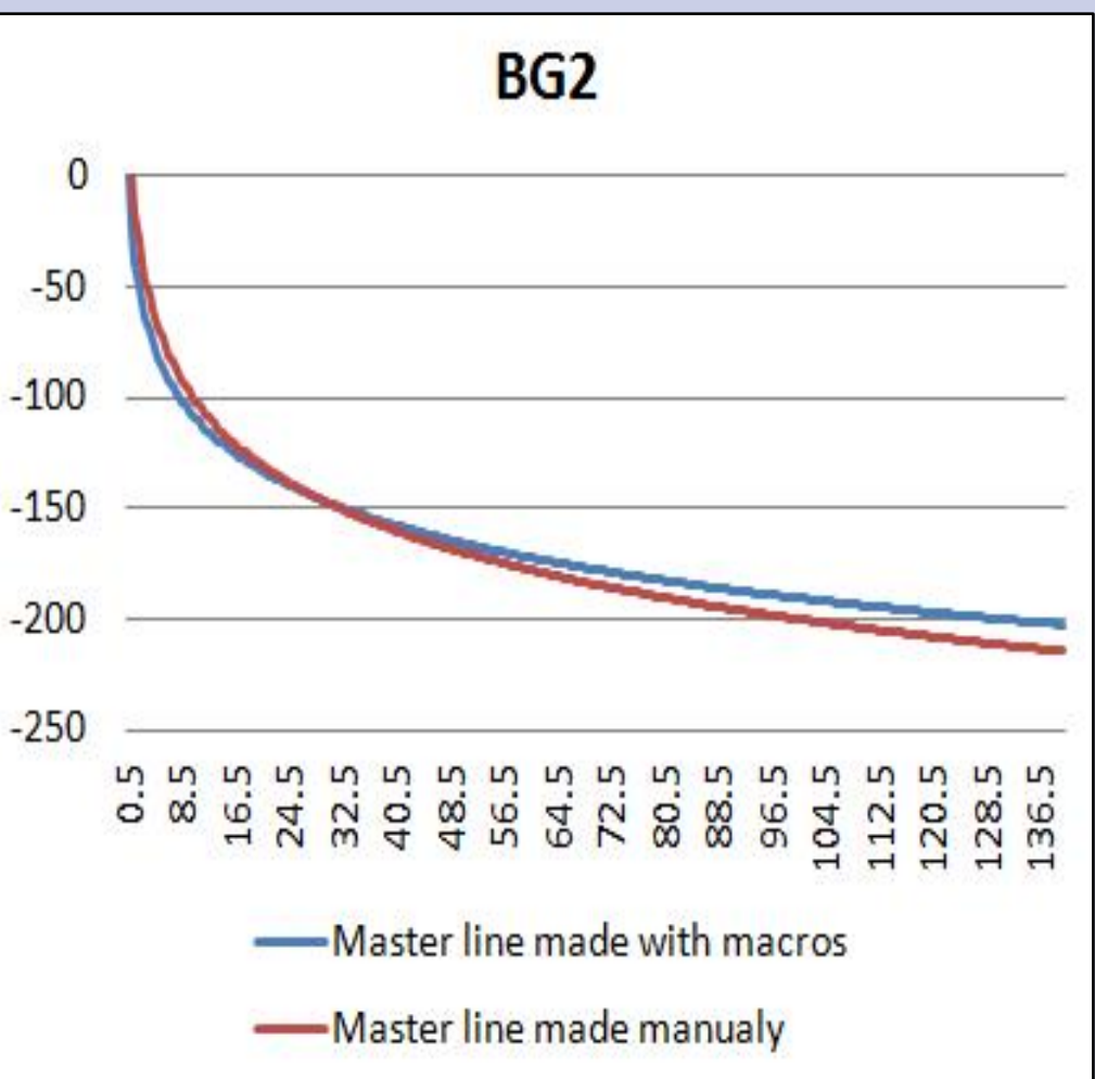
Figure 7. Master recession curves for groundwater levels
