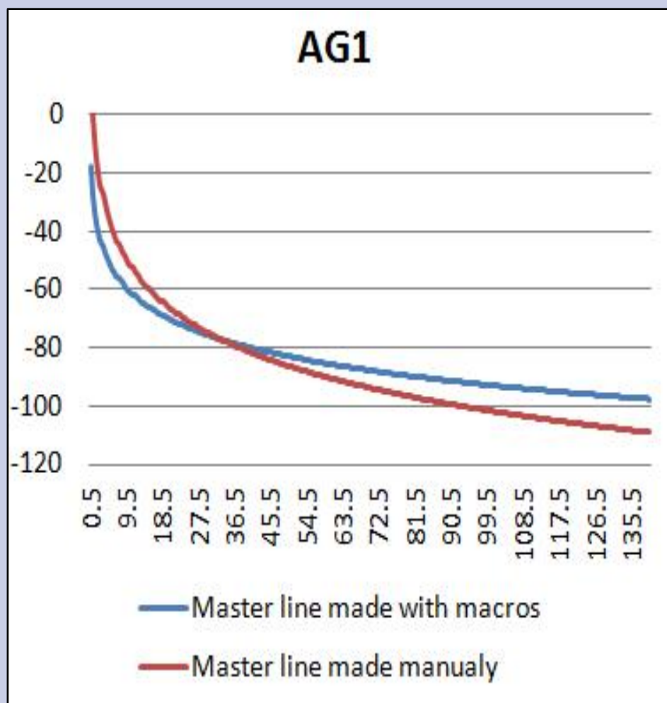
Figure 7. Master recession curves for groundwater levels
