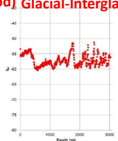
Ice core 3,000 m, 0-720 kyr
