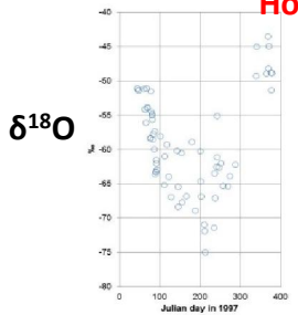
Precipitation 1 year
