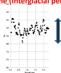
Surface snow (Pit) 2.3 m, 0-30 year
