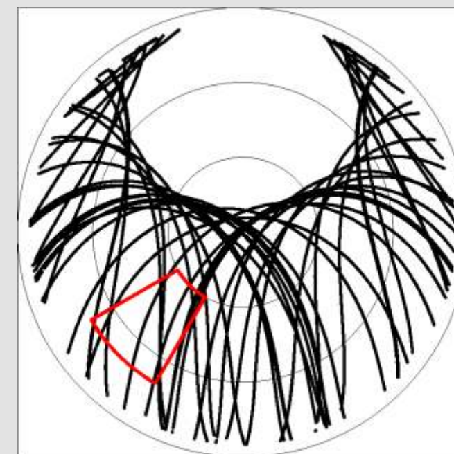
Figure 7: Skyplot for the GPS satellites of site 0384 for DoY2013: 200 with modified PCV sector in red.
