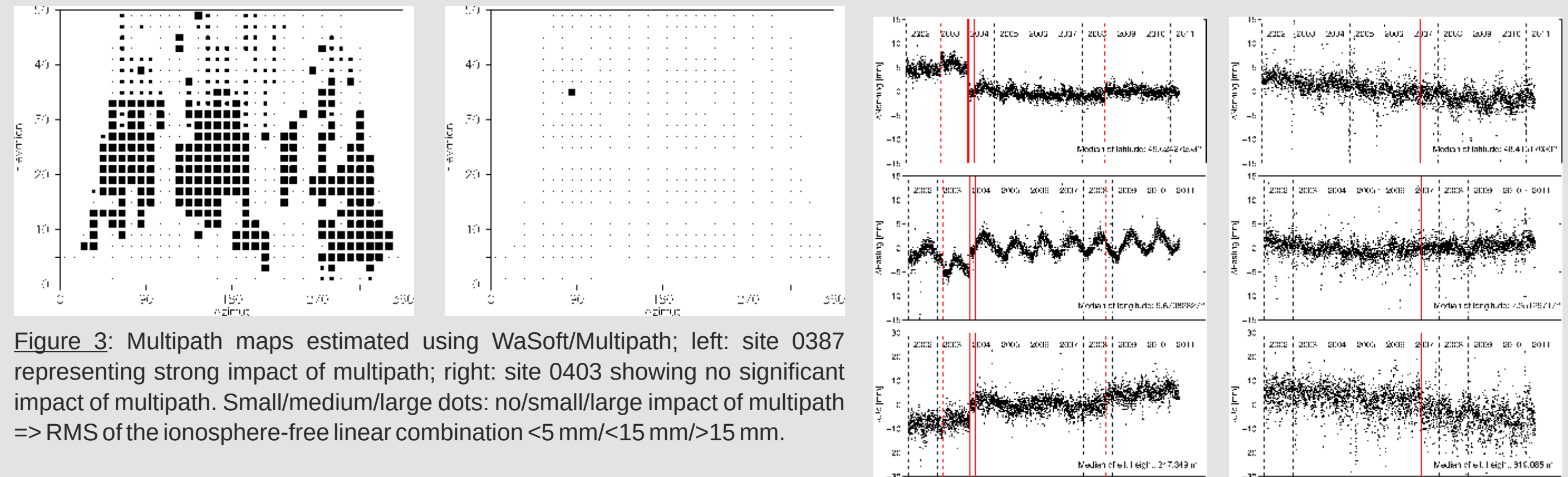
Figure 3: Multipath maps estimated using WaSoM/Multipath; left: site 0387 representing strong impact of multipath; right: site 0403 showing no significant impact of multipath. Small/medium/large dots: no/small/large impact of multipath => RMS of the ionosphere-free linear combination <5 mm/<15 mm/>15 mm.
