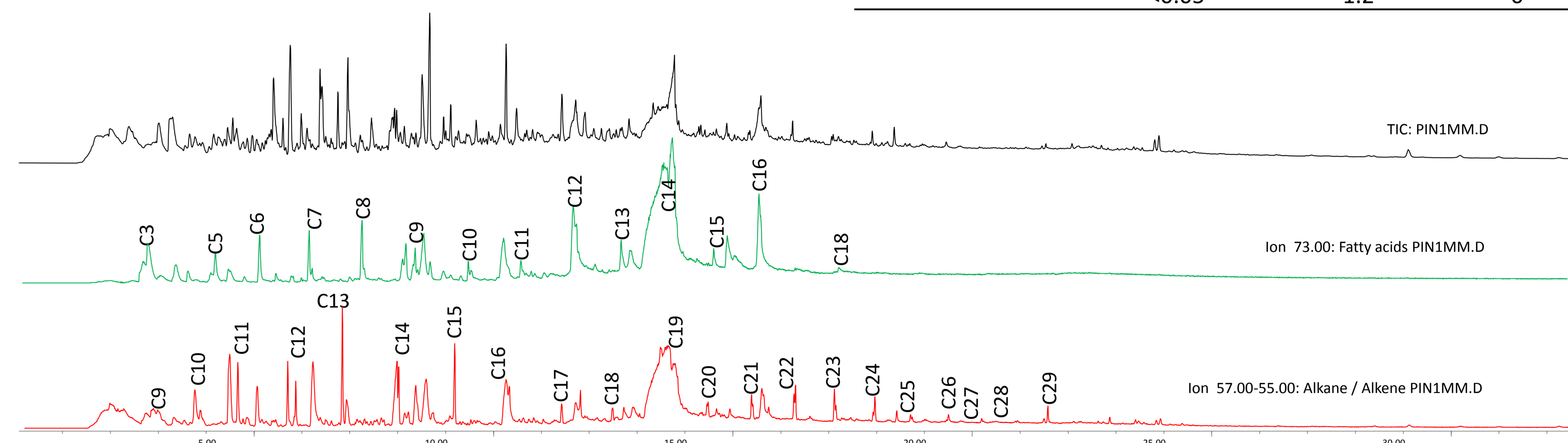
Figure 3. Total ion chromatogram (TIC) chromatogram of fatty acids (ion 73.00) and alkane/alkene (ion 57.00-55.00) of the 1-2 mm aggregate sieve fraction collected under Pinus pinea .
