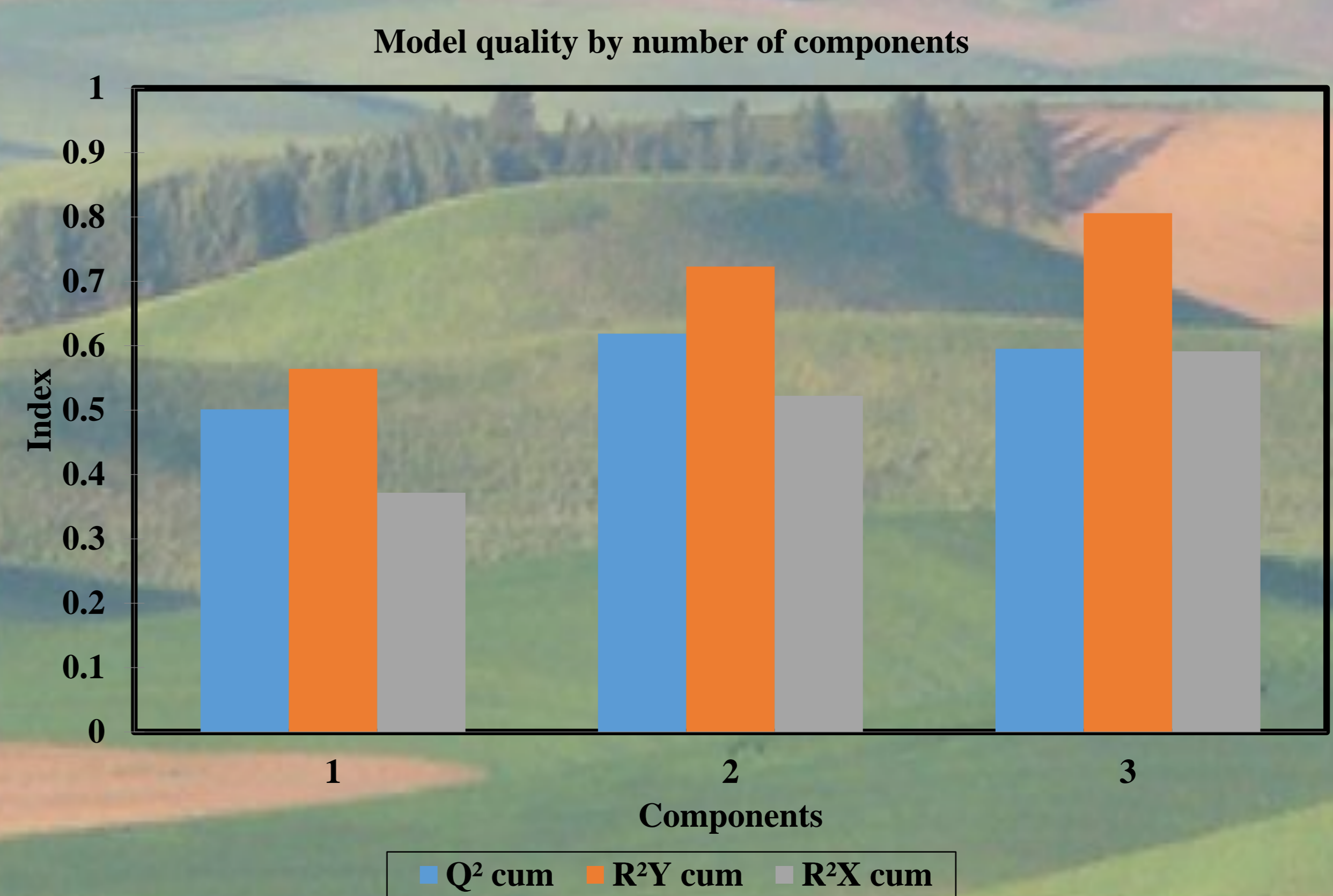
Figure 2. The number of components in the PLS model
