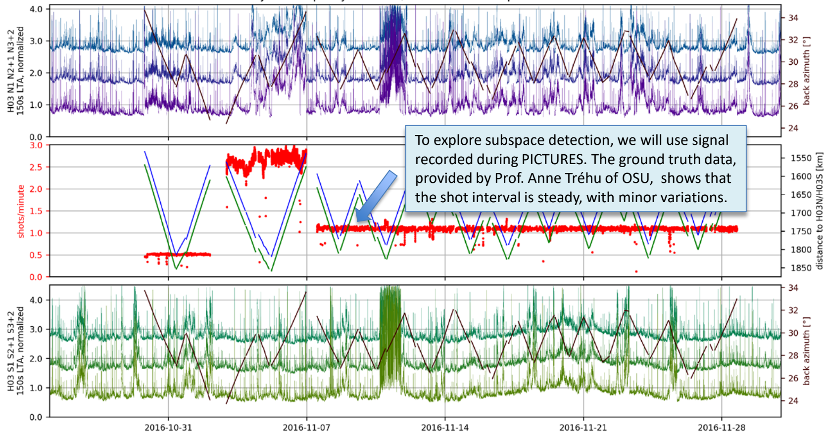
PICTURES survey shot frequency and H03N/H03S 150 s LTA for pass band 16.0-32.0 Hz
