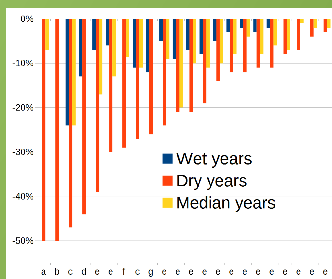
Figure 3 : Stream discharge decrease for wet, median and dry years. Every bar corresponds to a catchment for which the stream discharge decrease was estimated.
