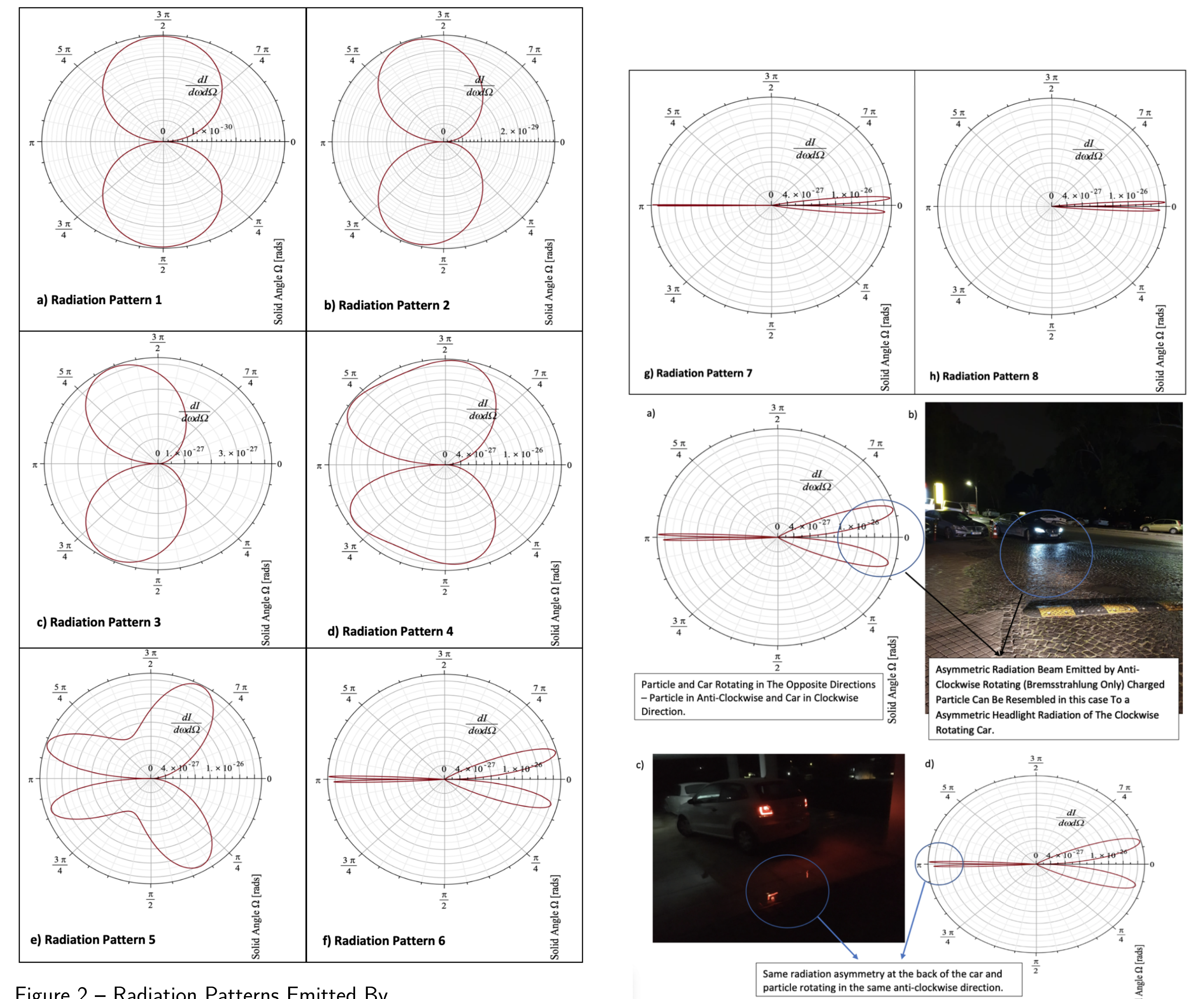
Figure 2 – Radiation Patterns Emitted By Anti-Clockwise Rotating Charged Particle. Particle's forward direction is to the right - towards 0 rads in 8 radiation plot.
