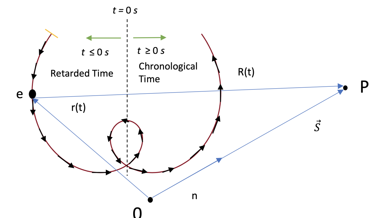
Figure 6 – Radiation Emission By change in Velocity over Time by A Coulomb Force of Other Charges and External Leader Tip Electric Field. O represents the target particle that defines the spiral trajectory of electron due to Coulomb force. Particle (electron) acceleration and velocity vectors are displayed with black arrows and are tangential to the spiral trajectory (red line). Hence, perpendicular to the position vector r(t)[m] . R(t)[s] gives the distance between accelerated single particle (source) and the observer all the time. P is the position of observer. \vec{S}[W/m^2] is a Poynting vector of emitted electromagnetic wave and it gives the direction of energy flow rate per area. n (Dimensionless) unit vector in the direction of power flow.
