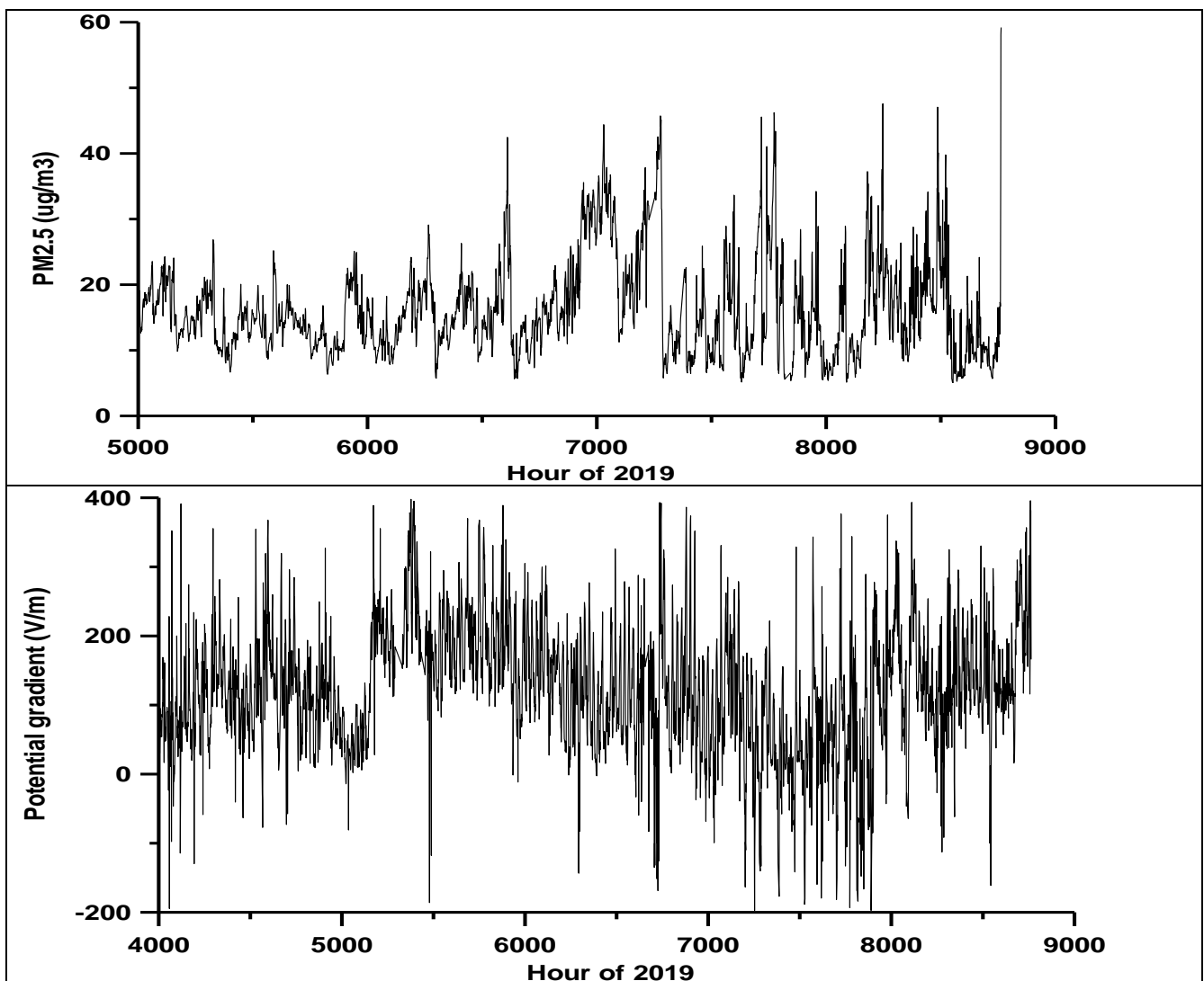
Fig. 2: Mean hourly values of PM2.5 (top) and mean hourly values of Potential Gradient (middle). As values of PG below -200 V/m or above 400 V/m are associated with very disturbed conditions (i.e. thunderstorms, nearby lightning or passage of electrified clouds), we show in the figure only the PG timeseries for PG values between -200 V/m and 400 V/m, although there were instances where PG went above 4000 V/m or below -8000 V/m.
