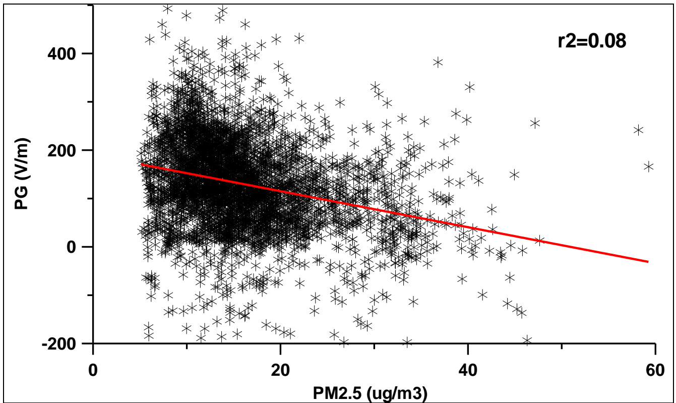
Fig. 3: Scatter plot of hourly values of PM2.5 versus PG (only for PG values between -200 and 400 V/m). R^2=0.08 . There is some influence of the aerosol concentration, as determined by the in-situ measurements, on near-ground PG. An increase of PM2.5 by 10 \mu\text{g}/\text{m}^3 decreases the field by around 37 V/m.
