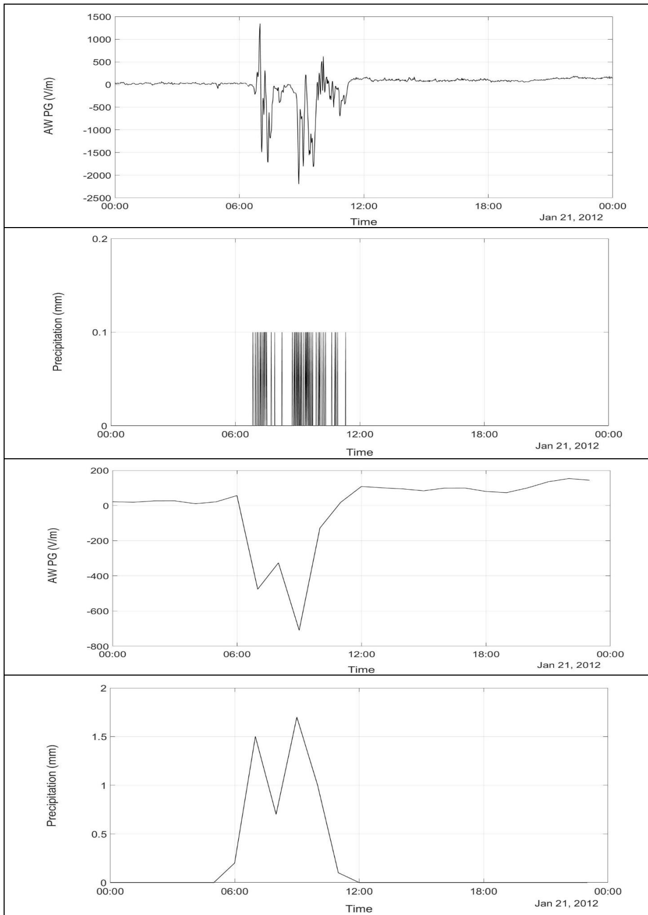
Figure 1: Rain and PG during the 21/01/2012. 1-min values in the upper panels, hourly values on the two lower panels. There has been no rain for the last 15 days.
