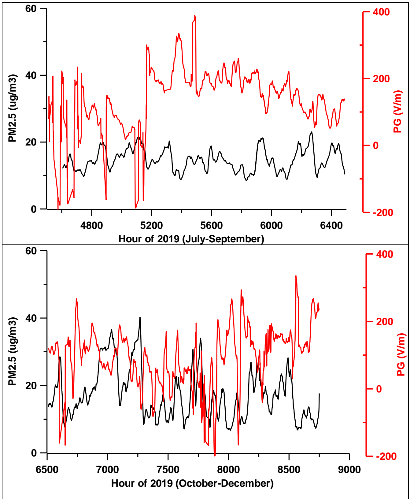
Fig. 4: Running average (window=23 hrs) of hourly PG and PM2.5 timeseries for summer and winter. Anticorrelation is evident, especially for summer (upper panel).
