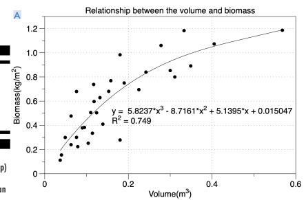
Figure 7-Biomass Model A) Relationship between the volume and biomass(F) B) Relationship between the actual and predicted biomass
