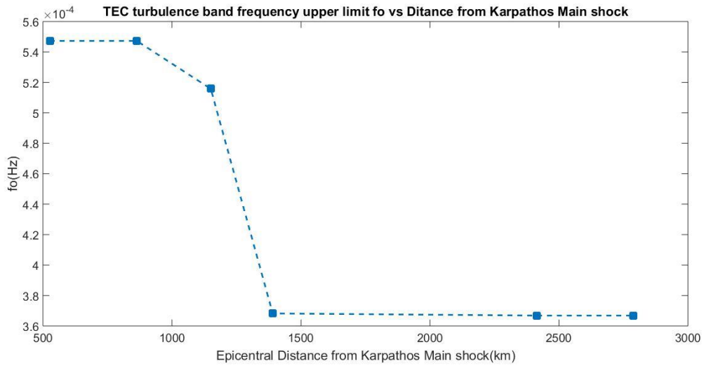
Figure 6. Variation of TEC turbulence frequency upper limit f_o over the GPS stations with the epicentral distance, at 10/12/2019 i.e. the day of Karpathos earthquake.
