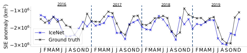
Fig. 4: IceNet's predicted sea ice extent (SIE), plotted as an anomaly from the 1979-2015 climatological sea ice extent.
