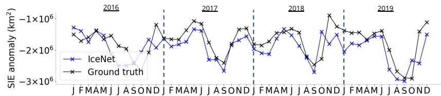
Fig. 4: IceNet's monthly predicted sea ice extent (SIE), plotted as an anomaly from the 1979-2015 climatological sea ice extent.
