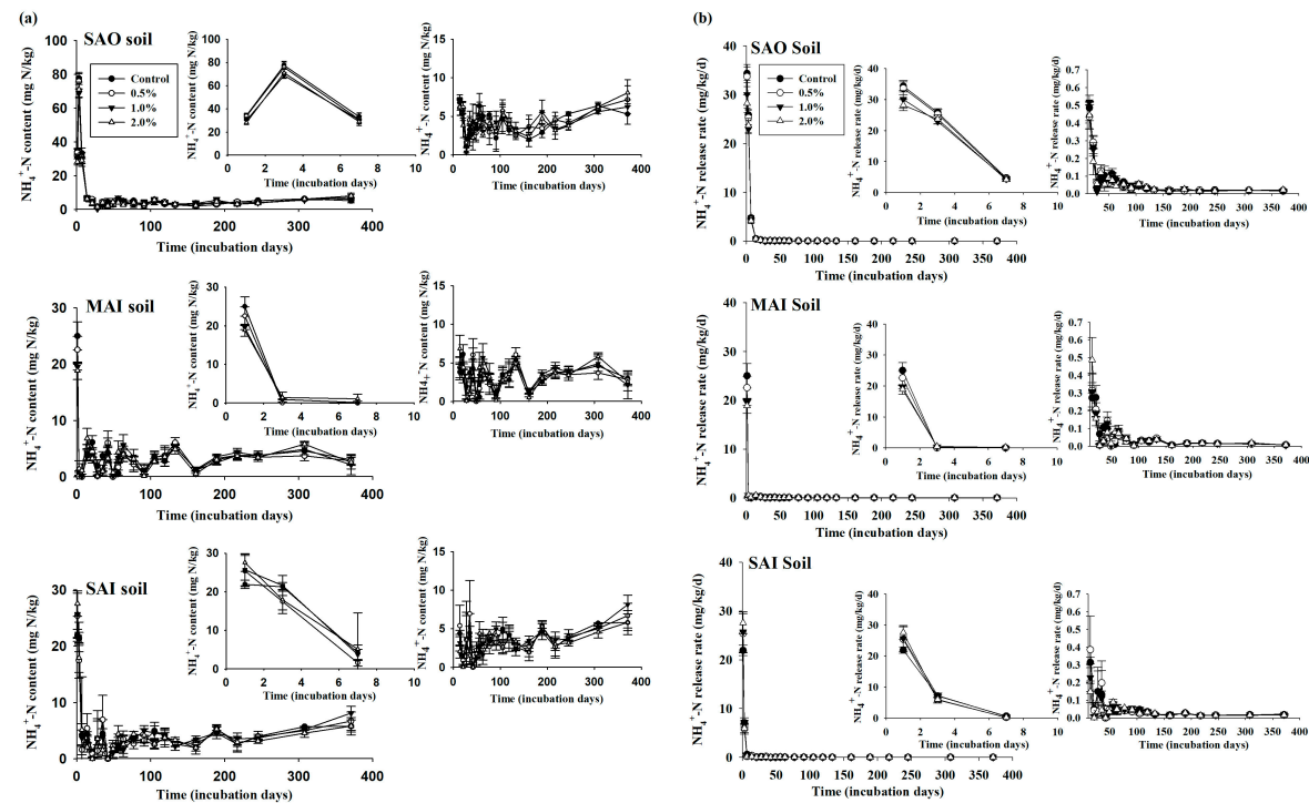
Figure 1. Effects of biochar additions on (a) \text{NH}_4^+ -N content and (b) \text{NH}_4^+ -N release rate. For each incubation time, release rate was calculated as the amount of release divided by the incubation time. The data are mean value ( n = 5 ), and vertical bars represent standard deviations (SDs) of the means.
