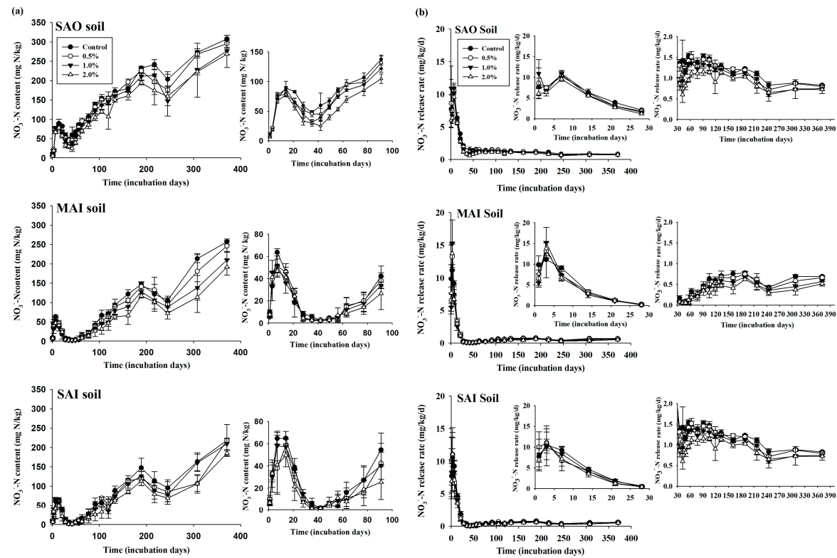
Figure 2. Effects of biochar additions on (a) \text{NO}_3^- -N content and (b) \text{NO}_3^- -N release rate. For each incubation time, release rate was calculated as the amount of release divided by the incubation time. The data are mean value ( n = 5 ), and vertical bars represent standard deviations (SDs) of the means.
