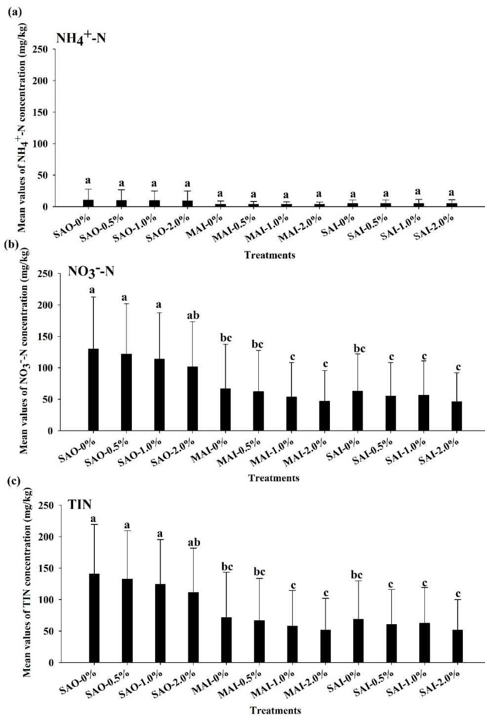
Figure 3. Mean values (mg/kg) of (a) \text{NH}_4^+\text{-N} , (b) \text{NO}_3^-\text{-N} , and (c) total inorganic N (TIN) in three studied soils during a 371-day incubation. The different lowercase letters indicate the significantly difference at p < 0.05 between treatments. The data are mean value ( n = 110 ), and vertical bars represent standard deviations (SDs) of the means).
