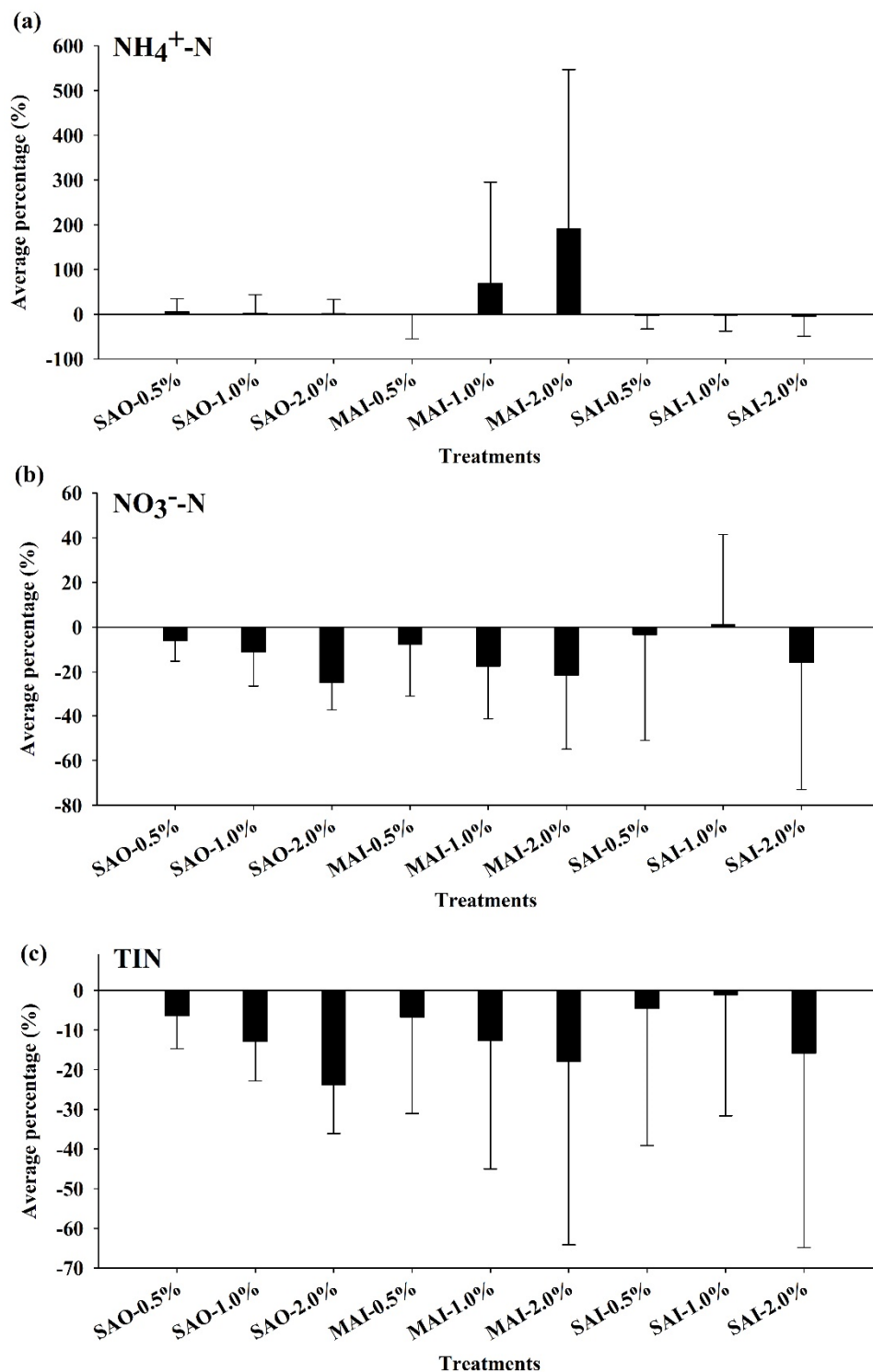
Figure 4. Average percentage (%) (22 times) of mean relative value of (a) \text{NH}_4^+\text{-N} , (b) \text{NO}_3^-\text{-N} , and (c) total inorganic N (TIN) in three studied soils during a 371-day incubation. Percentage expressed as the difference between biochar amended treatments and un-amended control treatment. The data are mean value, and vertical bars represent standard deviations (SDs) of the means.
