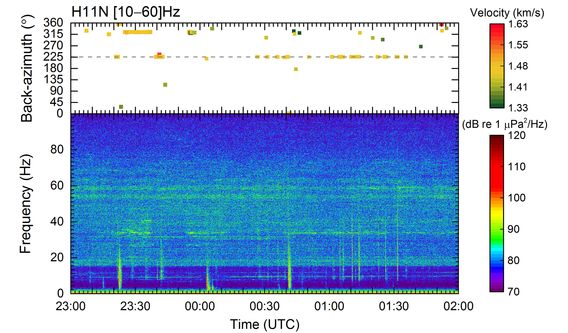
Figure 7. Back-azimuth evaluated by the cross-correlation analysis of H11N and the corresponding spectrogram on 09 February 2018.
