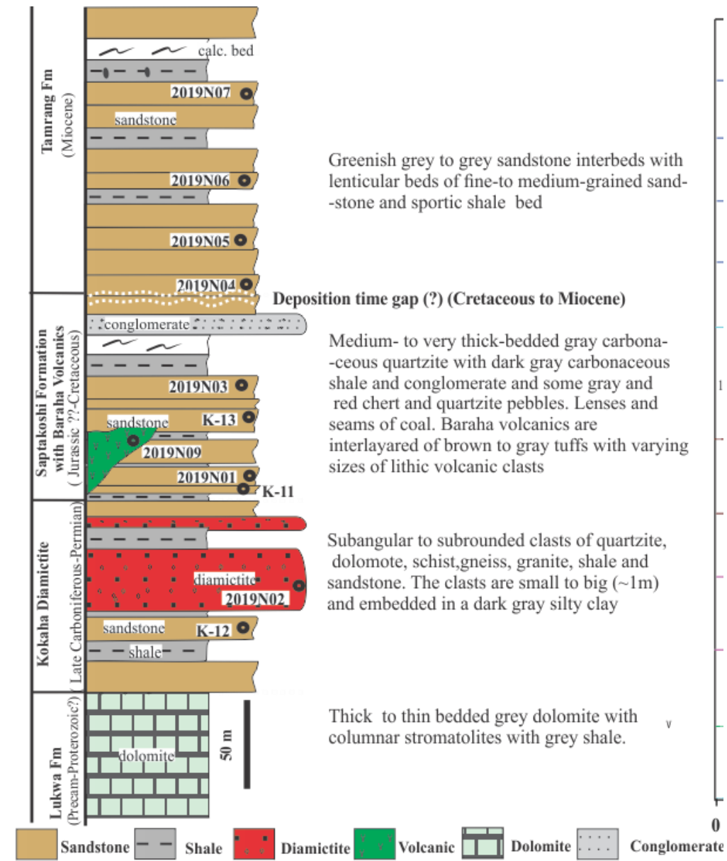
Columnar section of Gondwana sequence presented along the Barakshetra area, eastern Nepal
