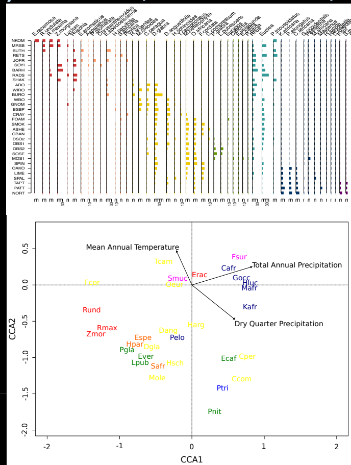
Figure 2: Pollen diagram adapted from Parkinson et al, 2000 with corresponding CCA
