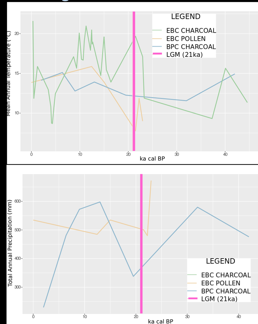
Figure 3: Reconstructed Mean Annual Temperature and Total Annual Precipitation
