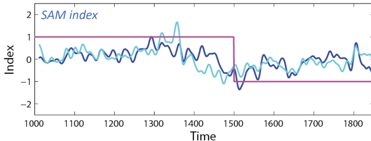
SAM index used as forcing
