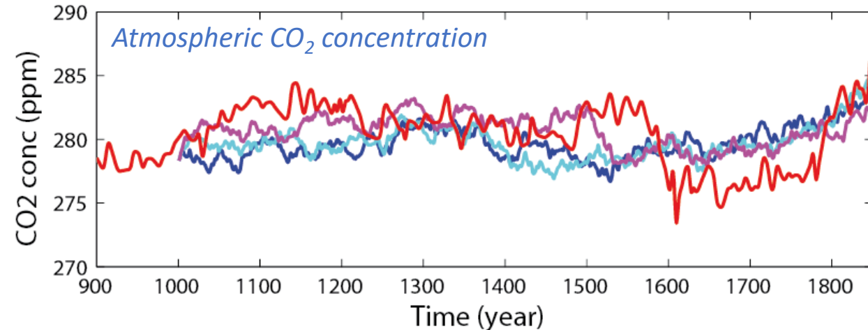
Response in the coupled model of intermediate complexity LOVECLIM
