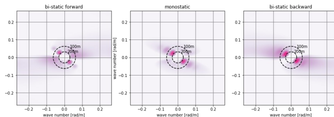
Bistatic SAR spectra
