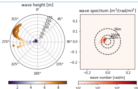
Inflow angle affects radiating wave pattern
