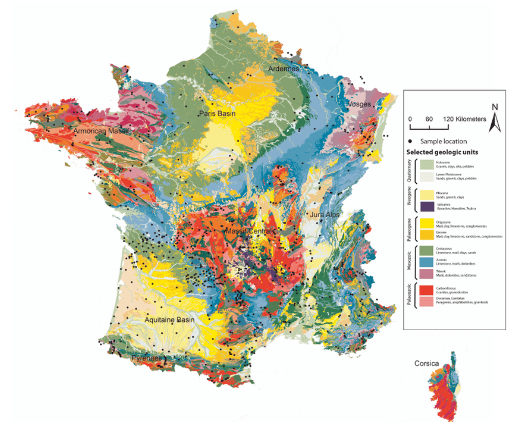
Geology
