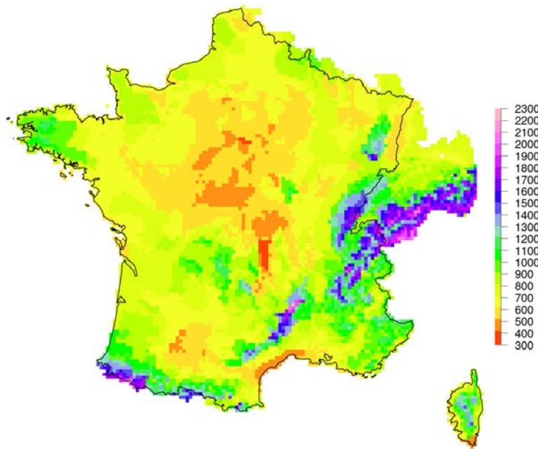
Precipitation (mm/yr)
