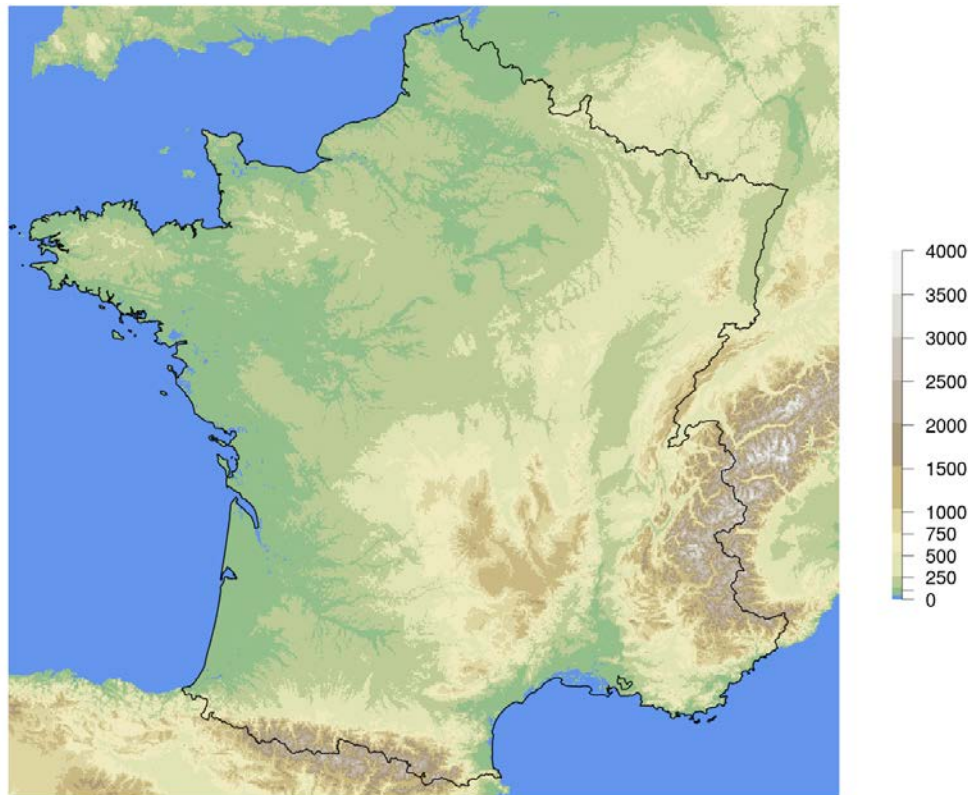
Elevation (m)
