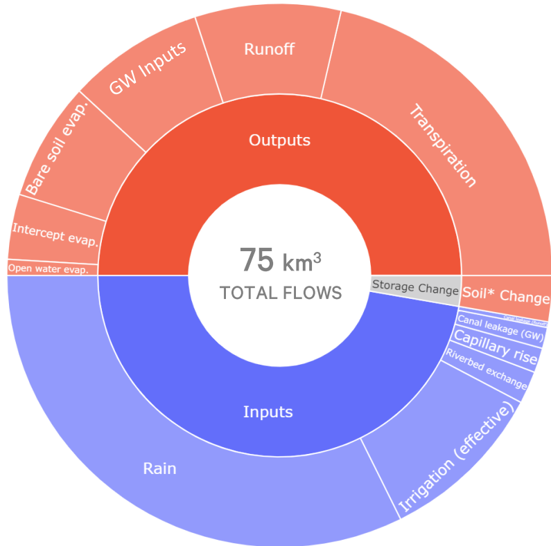
Soil moisture flows
