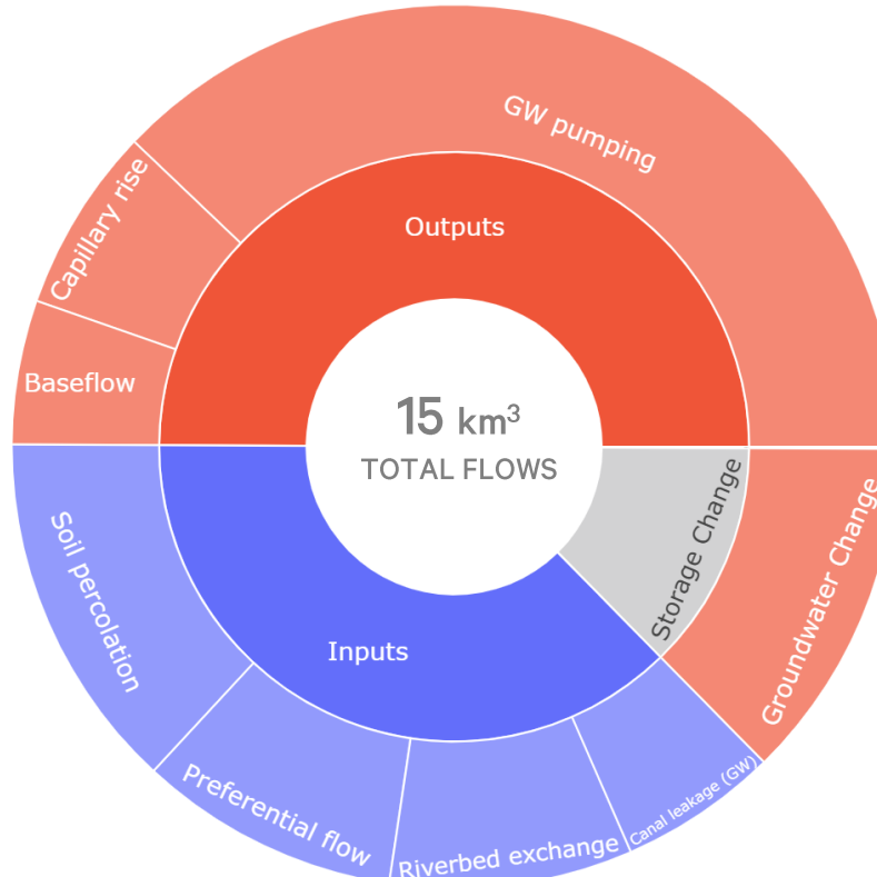
Groundwater (GW) flows
