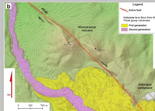
Khonarasar volcano, split by PSS fault
