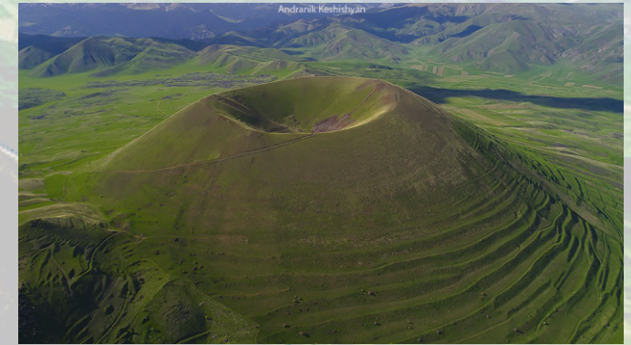
Vayotssar upper Pleistocene volcano
