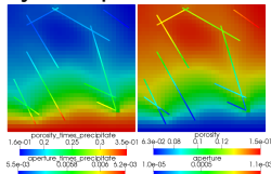
occluding fractures
