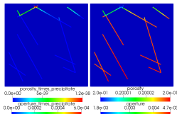
opening fractures
