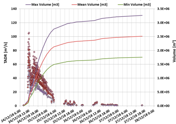
TADR and volume retrieved by HOTSAT using SEVIRI
