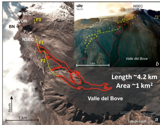
Lava flow (red) on GE (from Calvari et al., 2020 – doi:10.3390/rs12060905)
