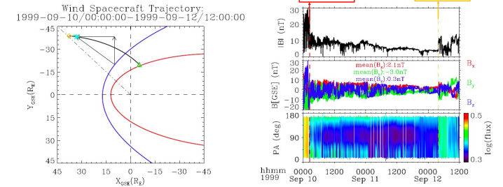
Fig 1: (Left) Wind Satellite orbit (green) with empirical model bow shock (blue, see Peredo et al., 1995) and magnetopause (red, see Roelof & Sibeck, 1993) plotted for reference. The triangle and diamond respectively represent the start and end of Wind trajectory. The asterisk denotes the position where an IP shock was detected by Wind. (Right) The Wind observations which corresponds to the trajectory shown in the left. From top to bottom, the panels show the magnetic field magnitude, GSE components of the magnetic field, pitch-angle distribution of 340 eV electrons.
