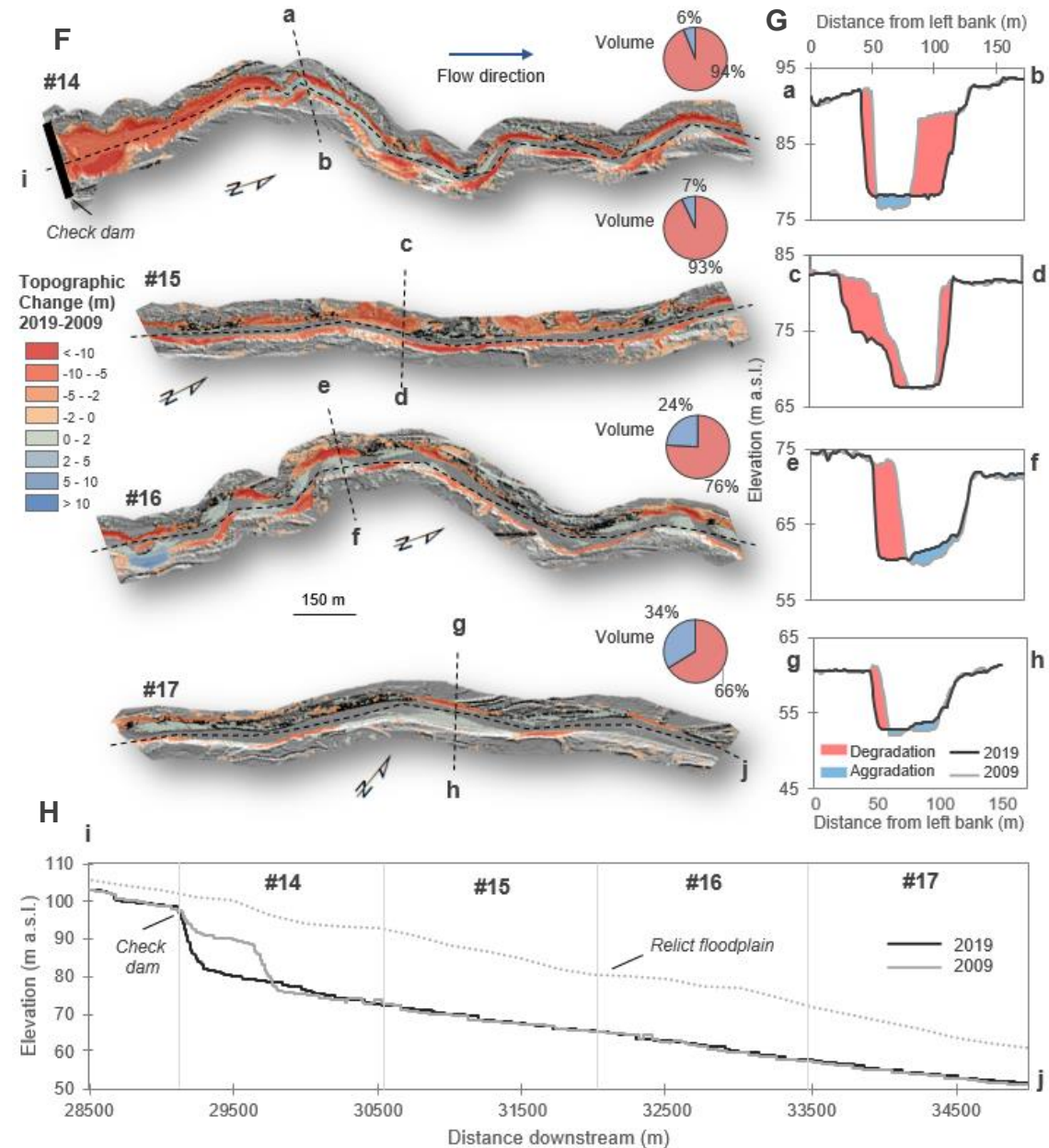
A. Study area location. B. Study reaches segmentation sketch map. C. Mean active channel width and local slope. D. Active width change and confinement. E. Volumetric changes. F. DoD maps of Canyon study reaches. G. Representative cross sections of canyon reaches. H. Longitudinal profile evolution of canyon reaches.
