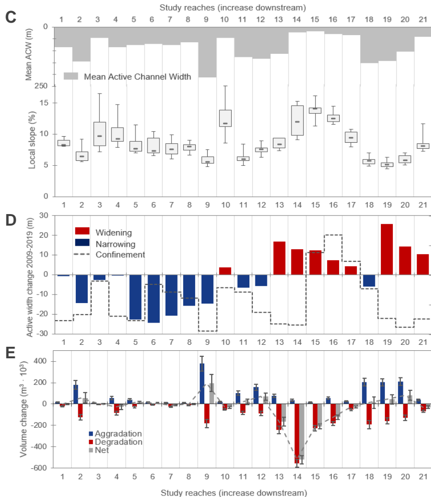
A. Study area location. B. Study reaches segmentation sketch map. C. Mean active channel width and local slope. D. Active width change and confinement. E. Volumetric changes. F. DoD maps of Canyon study reaches. G. Representative cross sections of canyon reaches. H. Longitudinal profile evolution of canyon reaches.
