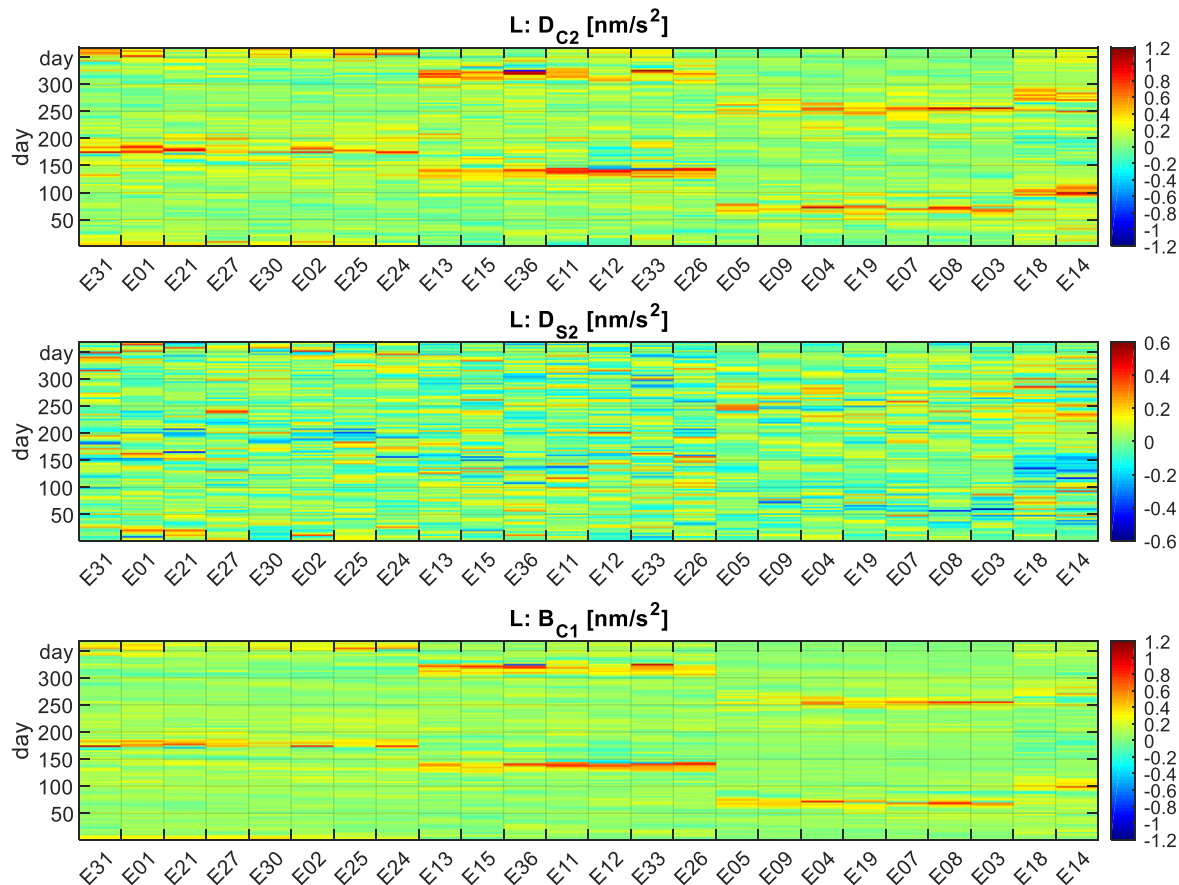
epoch-wise clocks
