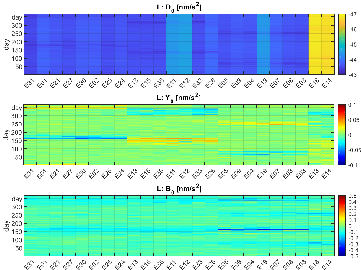
epoch-wise clocks
