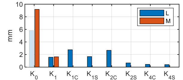
satellite clocks
