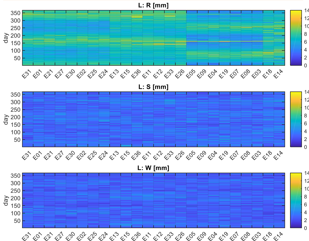
epoch-wise clocks
