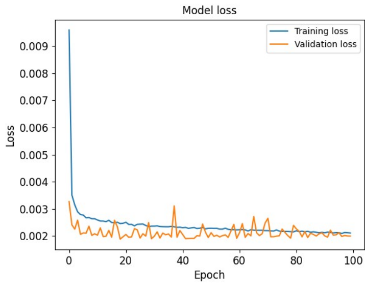
Figure 6. Mean squared error training loss for LSTM to predict divergence
