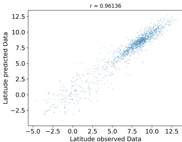
Figure 5. Correlation between the observed and predicted data for the latitude of maximum precipitation.
