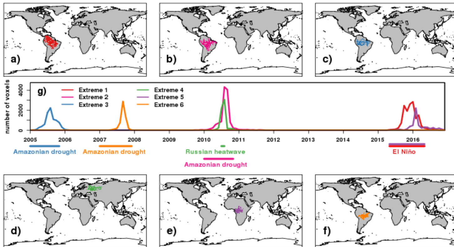
HCHO 95 percentile extremes
