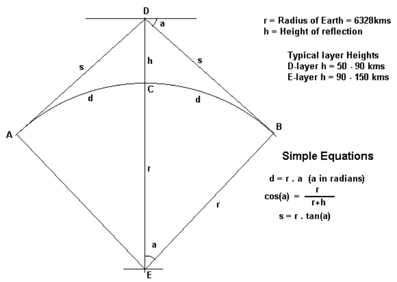
Simple Geometry of Ionospheric Reflection
