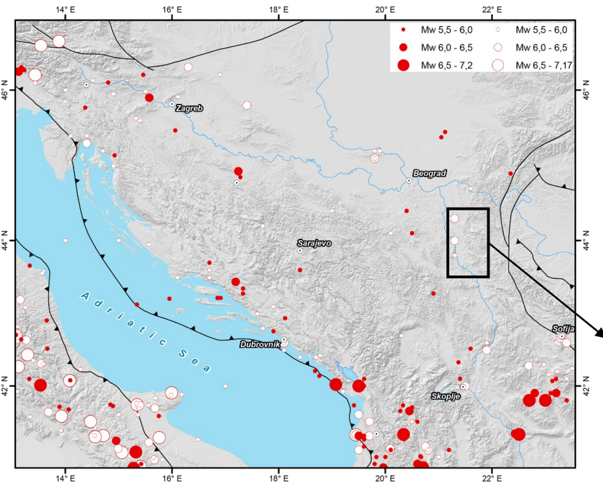
SHARE catalogue of historical and instrumentally located earthquakes
