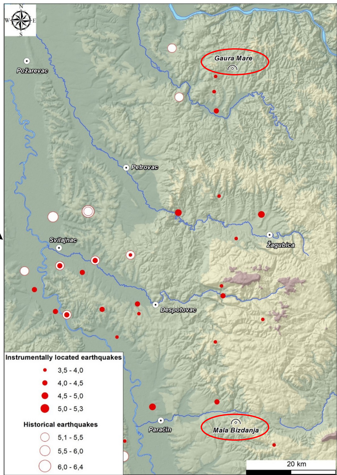
SHARE catalogue of historical and instrumentally located earthquakes
