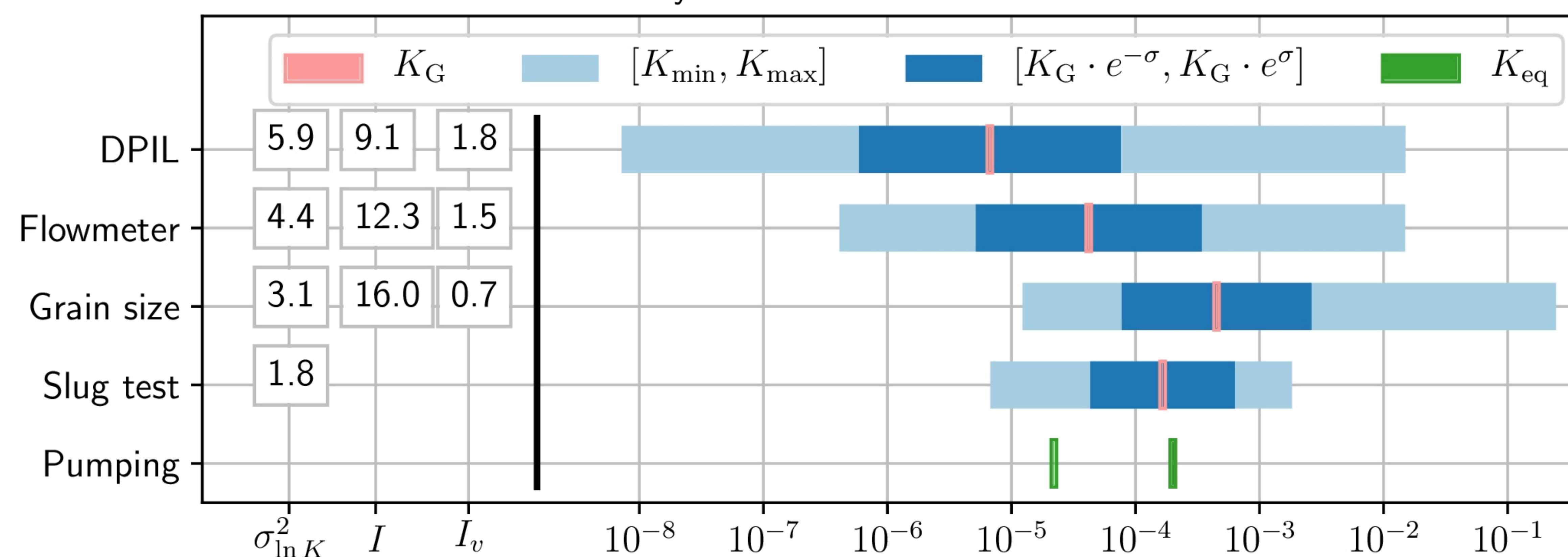
Geostatistics of hydraulic data at MADE with various methods
