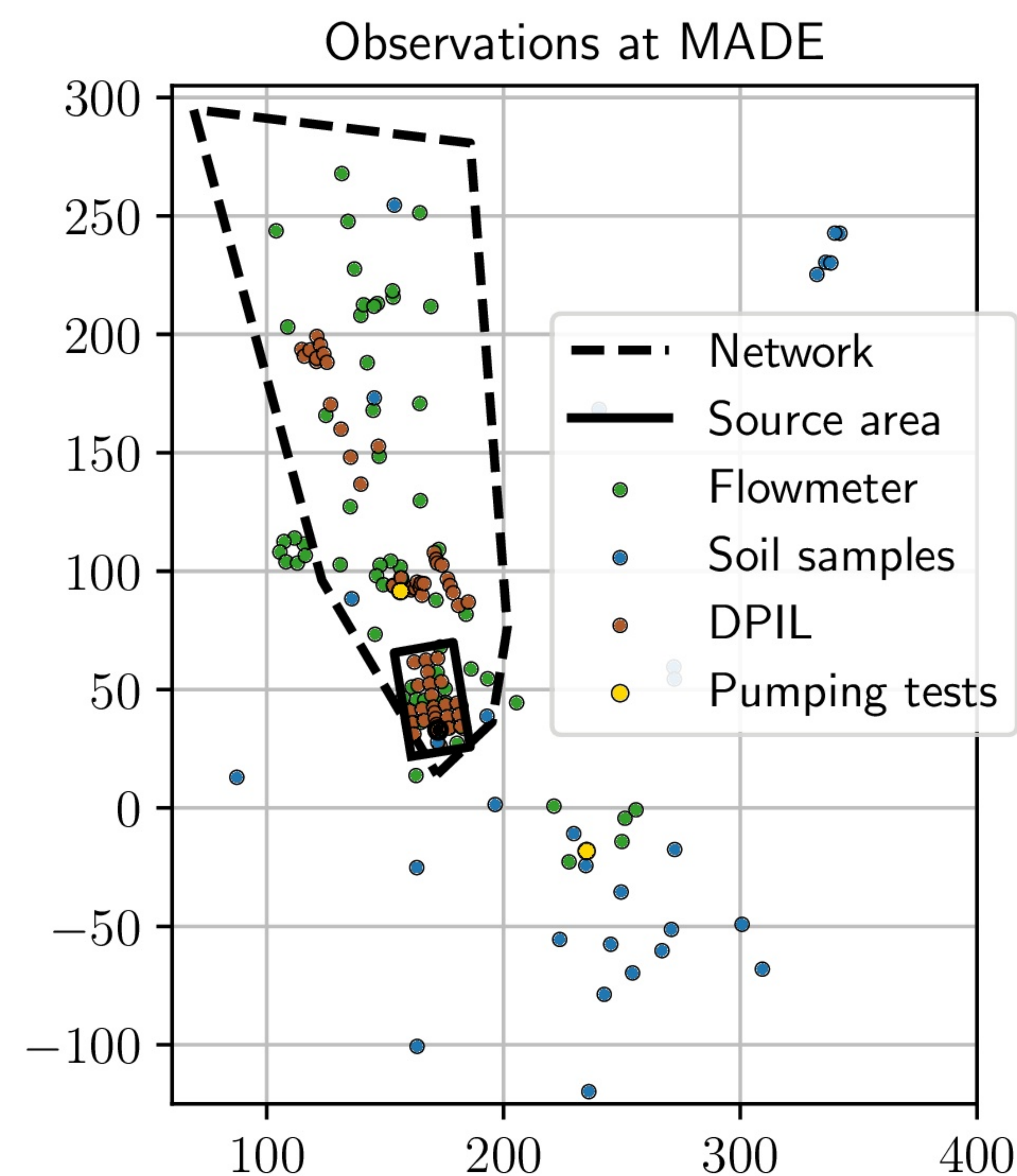
Geostatistics of hydraulic data at MADE with various methods
