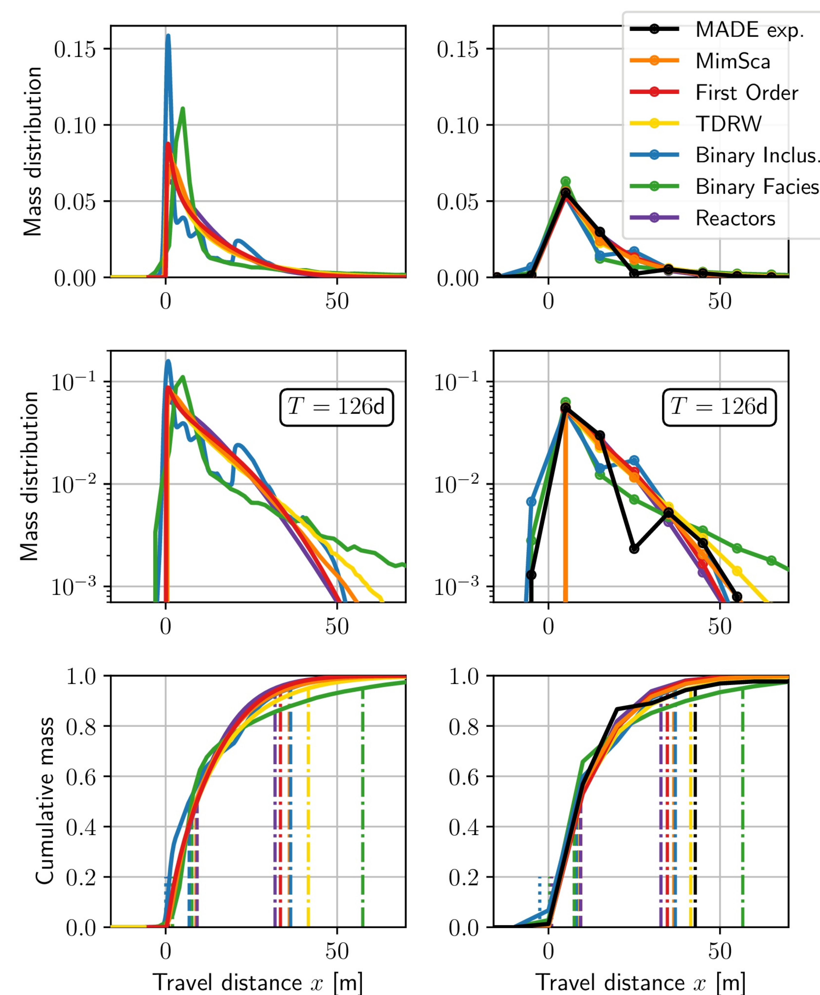
Longitudinal mass distribution for models and MADE observations for various display modes.
