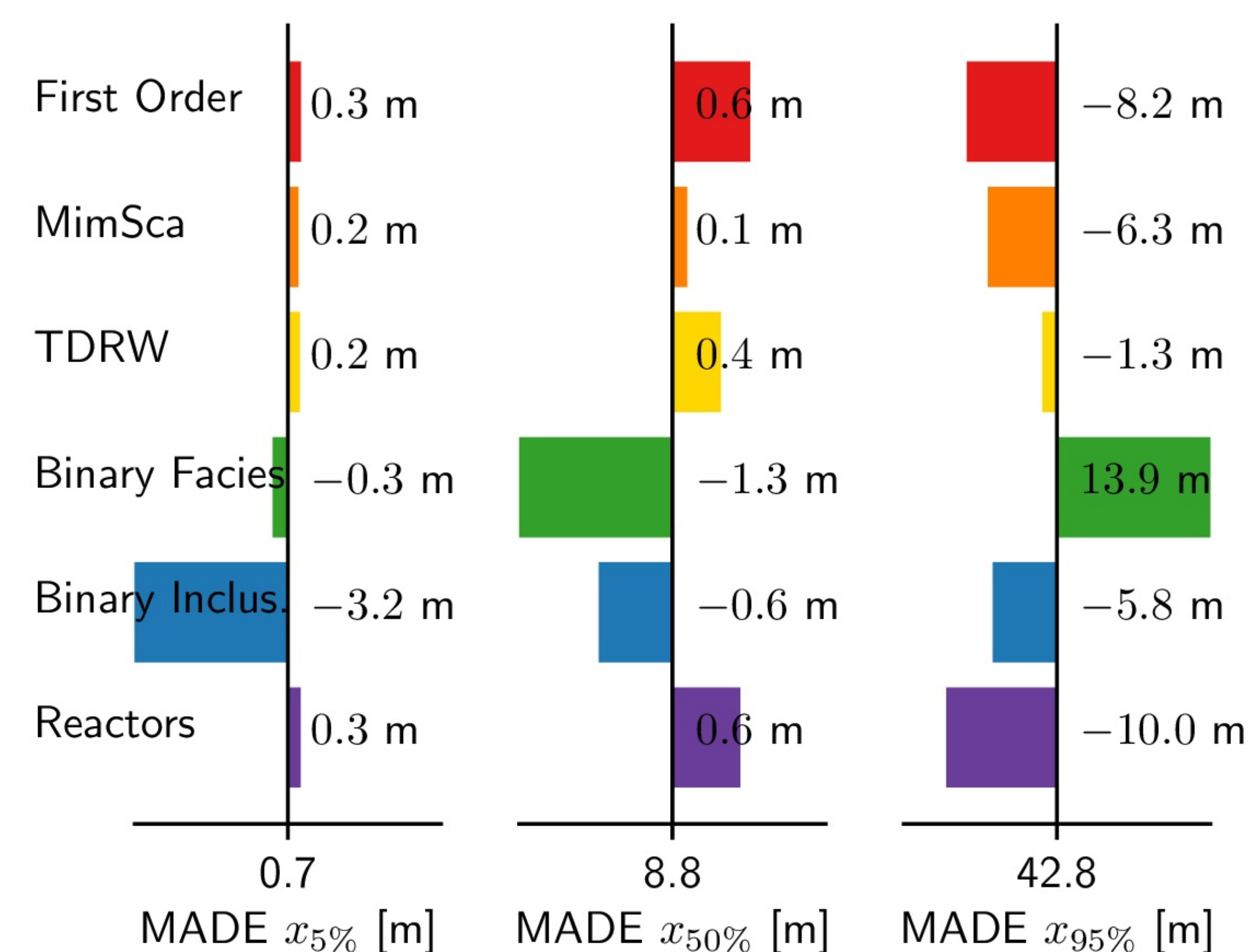
Model deviations recovery locations at 126 days from MADE observations.
