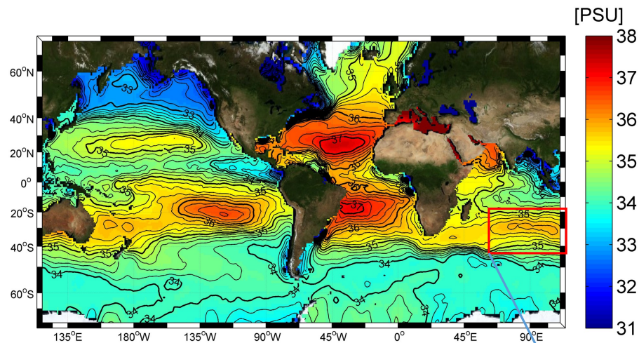
Annual mean SSS from the World Ocean Atlas
