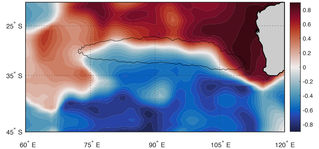
SSS correlation with yearly isohaline area
