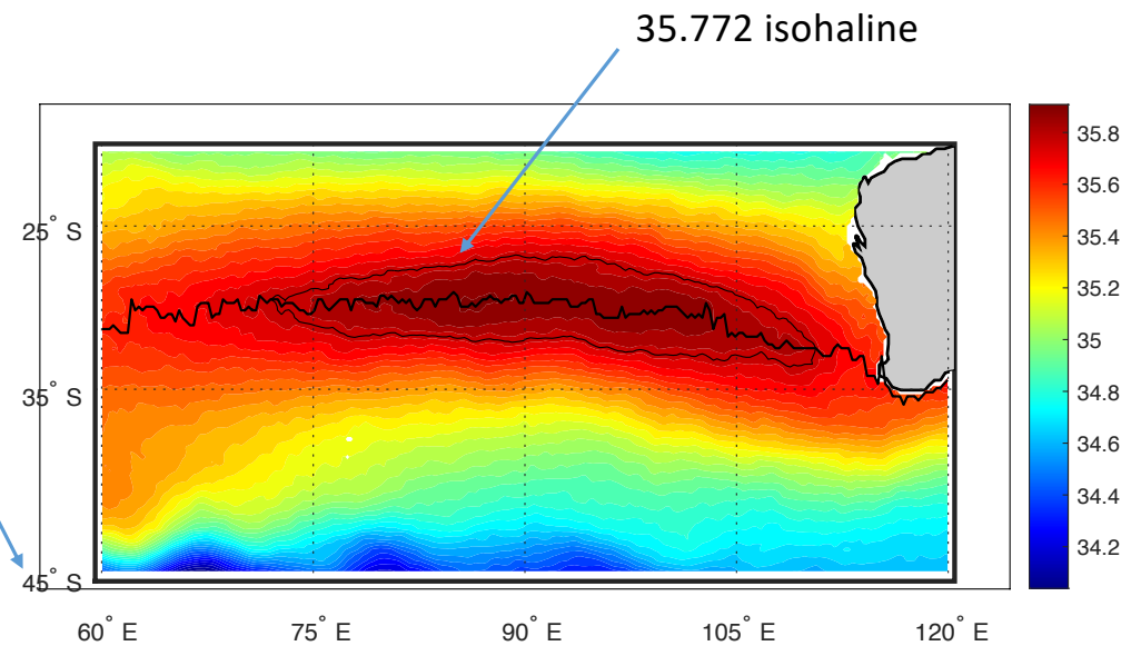
South Indian Ocean 2010-2020 mean
