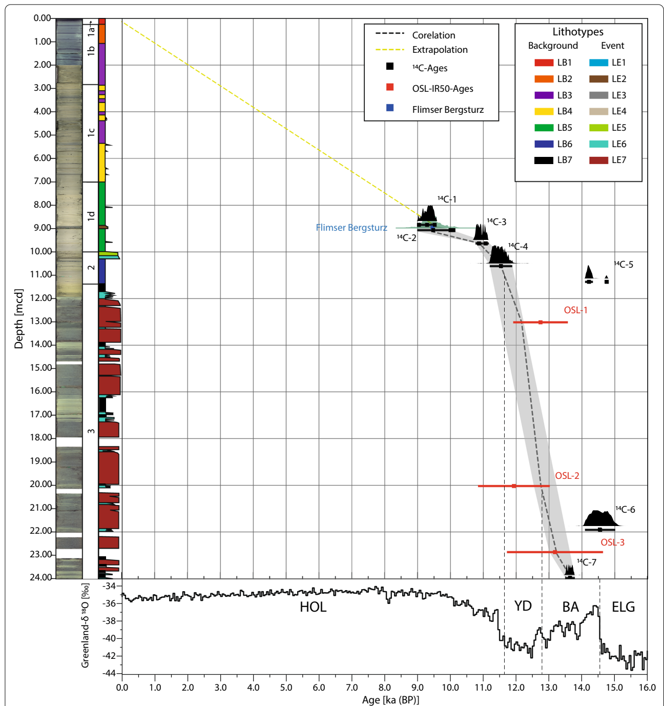
Fig. 6 Age-depth model of HIBO19 composite section. The ages are given in ka BP and marked with squares. Uncertainties are indicated by x-axis error-bars: ^{14}\text{C} (black, 2 \sigma -range); OSL-IR50 (red, gaussian approach); Flimser Bergsturz correlating (blue, given uncertainty). Depth scale in meter composite depth, the marker-size exceeds the depth-interval of the samples. The probability histograms for the ^{14}\text{C} -ages are given above the corresponding calibrated ages in black and for ^{14}\text{C} -2 in semi-transparent green. The age-depth correlation below 8.83 mcd is indicated by a black dashed line, above, the model was just extrapolated with a straight line (yellow dashed line). The probability envelope is indicated in grey. The \delta^{18}\text{O} data in [‰] (National Centers for Environmental Information (NCEI), 2020) from 0 to 16 ka BP as a global temperature proxy with the geochronological ages are plotted below: Hol, Holocene; YD, Younger Dryas; BA, Bølling–Allerød; ELG, Early late Glacial. The borders are extrapolated with vertical black dashed lines into the age-depth model. The combined composite photo, the stratigraphic units, and the lithotypes with the estimated grain size are given on the left side
