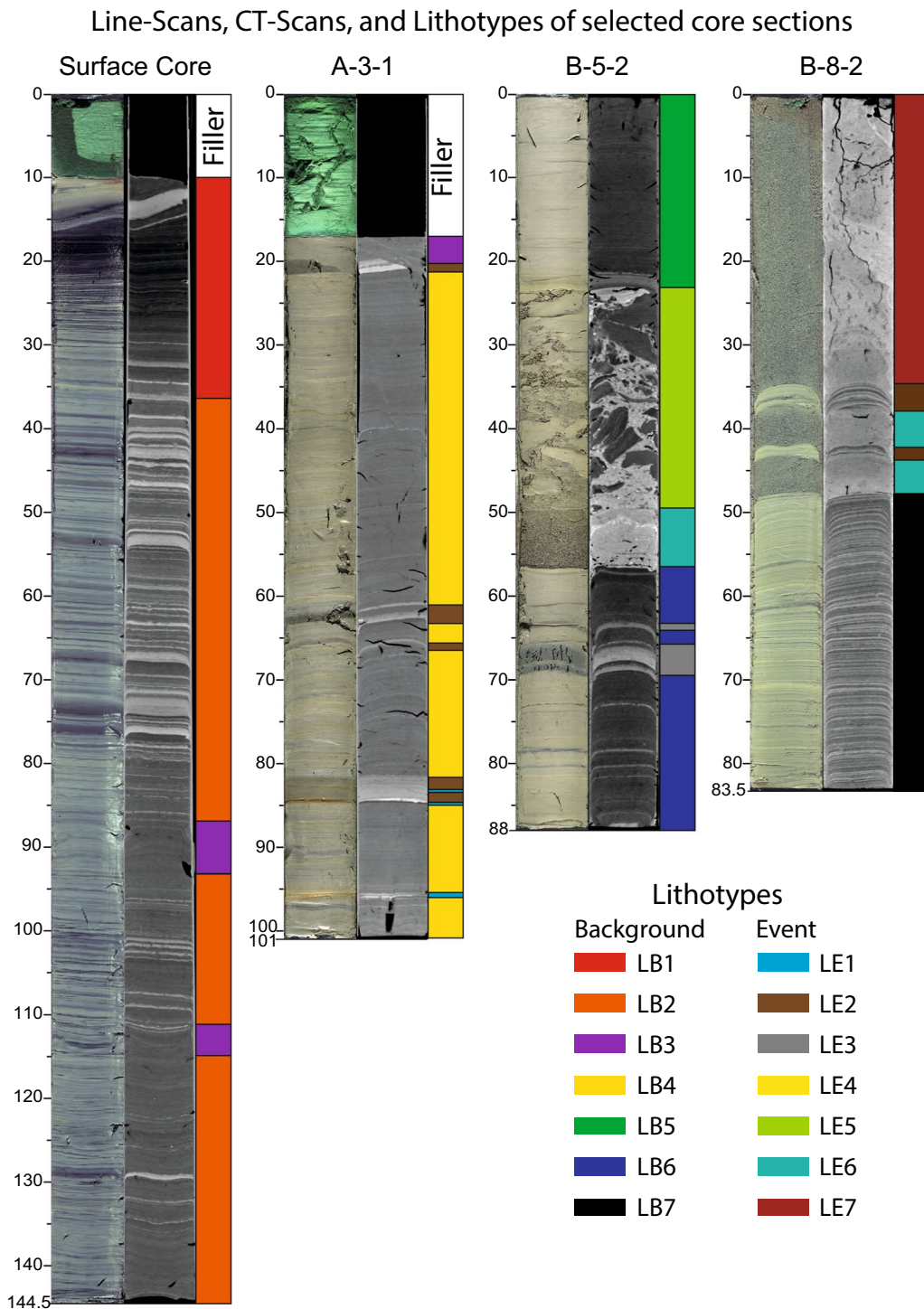
Fig. 5 CT and line scans of selected representative core sections of HIBO19. Each core section is labelled at the top, scale is in cm, each column shows from left to right: line scan, corresponding CT scan, and lithotypes. The color code for the lithotypes is given at the bottom right. Shown core-sections from left to right: Surface core (13–114 cm → 0–1.01 mcd), A-3-1 (61.5–100.5 cm → 6.19–6.58 mcd), B-5-2 (23.5–80.0 cm → 9.96–10.53 mcd), B-8-2 (0.5–75 cm → 15.8–16.545 mcd). A detailed graphical synopsis of the depth conversion of all sections, section parts included in the composite section, and the corresponding composite depth is provided in Additional file 2: Fig. S1
