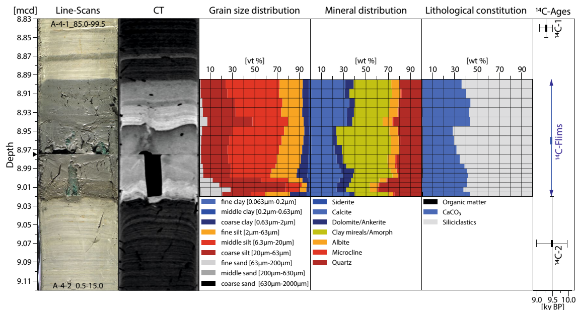
Fig. 9 Core section details of the prominent double event layer related to the Flims Bergsturz event. The corresponding line-scans (colored) and CT scans (black and white) of the event layer are depicted on the left. Bright colors correspond with high density and dark colors the low density. The lower section contains green colored artificial filler-material inserted for an extracted pore-water sample (black in the CT scans). The color-coded grain size distribution [v%], mineral distribution [wt%], and the lithological constituents [wt%] are displayed in the center, with respective sample intervals separated by horizontal black lines. Two of the ^{14}\text{C} -ages (black; with 2\sigma -range, Table 3) are shown in the right column in relation to a previously published Flims Bergsturz age (blue; Deplazes et al., 2007)
