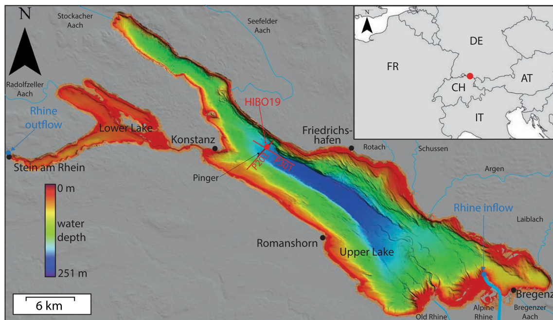
Fig. 1 Bathymetric map of Lake Constance including the location of the coring site (red dot, WGS84: 47.66813°/9.28686°), the traces of the three seismic profiles (airgun in red and pinger in black) crossing the coring site, and the paths of major inflowing streams in blue. The light-orange colored areas at the shore of the lake represent the terrestrial topographic lidar data with elevations >0 m above the reference lake level of 395 m a.s.l. (Wessels et al., 2015). Grey shaded area is the Lidar-based land topography (Swisstopo). The inset in the upper right corner shows the location of the study site (red dot) in Central Europe, with the indicated surrounding countries
