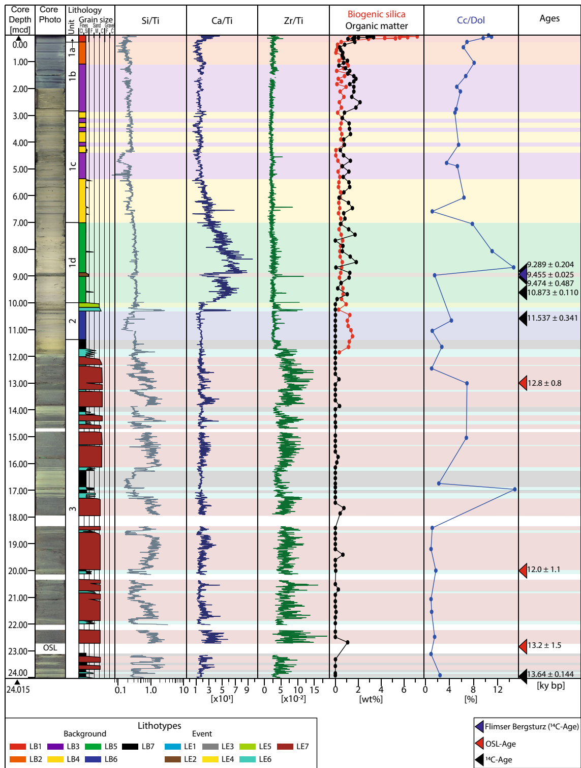
Fig. 4 Summary of key element geochemical ratios and bulk geochemical data over depth for the HIBO19 composite section. Columns from left to right: depth-scale [mcd], combined composite core photo (line scan), stratigraphic units, lithotypes (color code legend in lower left inset) with indicated grain size, XRF-data (Si, Ca, and Zr all plotted in respect to the Ti-data, for elemental curves see Additional file 3: Fig. S2), total organic matter [wt%], biogenic silica concentration [wt%], and the calcite-aragonite/dolomite ratio (Cc/Do) [%]. Relevant ages for the age-model with the corresponding errors are shown at right side. Lithotypes are shown as semi-transparent color codes over the plot's entire width, gaps in the cores are indicated in white
