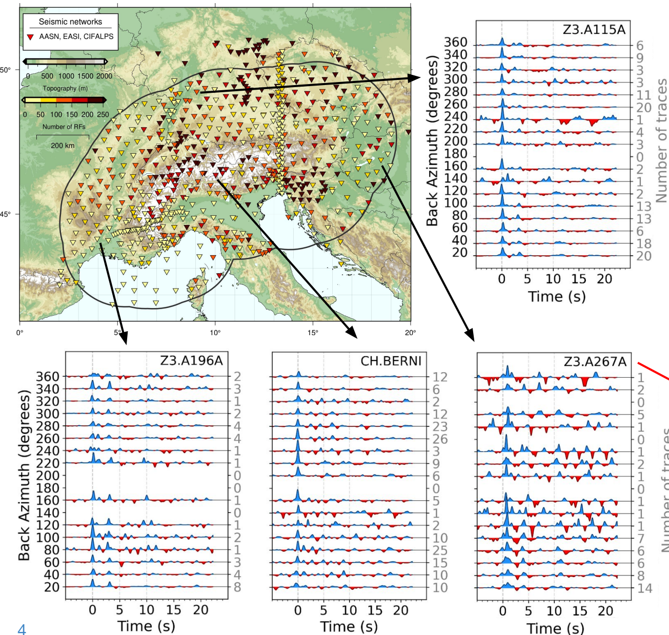
Figure 3. Map shows the number of receiver functions on each seismic sites. Plots show a selected subset of calculated receiver functions versus their back azimuth values from different environments (e.g., European foreland, high alpine region, and Pannonian basin).
