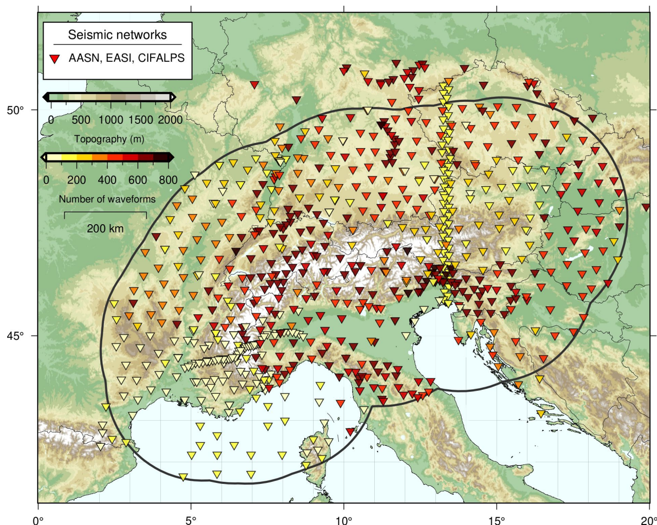
Figure 1. Distribution of three component broadband seismometers of the AlpArray Seismic Network ( AASN ), the Eastern Alpine Seismic Investigation ( EASI ) and the China-Italy-France Alps seismic transect ( CIFALPS ) used in this study. Seismic sites shown as inverted triangles are colored according to their number of waveforms.
