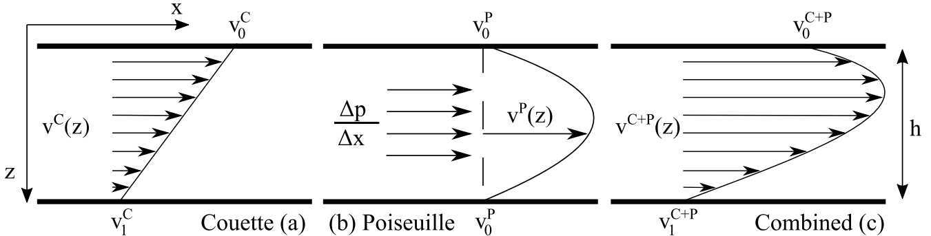
Figure 1: Schematic representation of (a) Couette flow, described a linear profile of shear driven fluid motion between two surfaces where one moves tangentially relative to the other, and seen as proxy for passive asthenosphere flow driven by motion of the overlying plate, (b) Poiseuille flow, described by a parabolic profile, driven by a lateral pressure gradient, and seen as proxy for active asthenosphere flow capable of driving the overlying plate, and (c) superposition of both.
