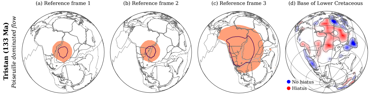
Figure 11: Estimates of Poiseuille flow dominated areas computed for Tristan at 133 Ma using three absolute plate motion models. (a) is the same as figure 10 and assumes a global Mesozoic-Cenozoic plate motion model [27]. (b) uses an Indo-Atlantic moving hotspot reference frame [151] for the past 100 Myrs and a TPW corrected paleomagnetic model [58] for older times. (c) applies a reference frame of Indo-Atlantic moving hotspots [151] for the last 100 Myrs and of fixed African hotspots [155] for prior times. (d) BHS for Base of Lower Cretaceous (see figure 3). Note that the size of hiatus and blank areas throughout Africa and South America in the Base of Lower Cretaceous map compares well to the extent of the Poiseuille-dominated area in Reference Frame 3.
