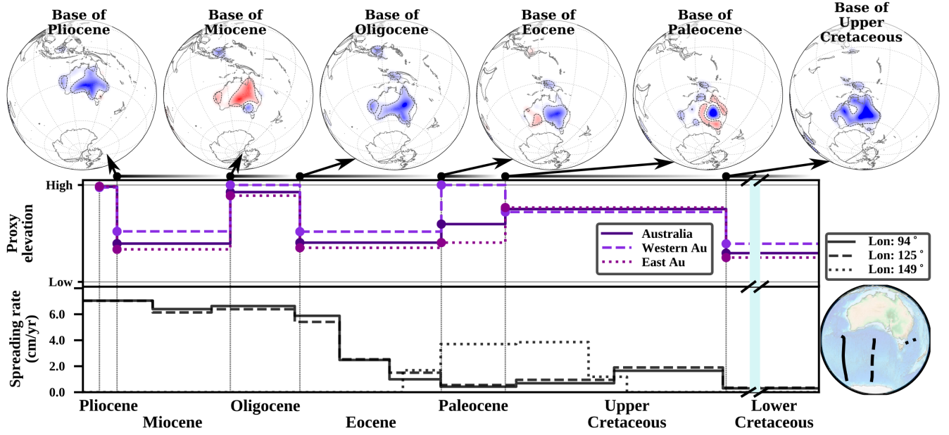
Figure 7: Same as figure 5 with view centred on Australia. Top row shows BHS (see text). Middle row shows proxy elevation curve for the entire continent or separated for eastern and western Australia (see text). Bottom row shows spreading rates for three transects as indicated in bottom right globe. Blue vertical line in the Lower Cretaceous represents a time-lapse omission. Elevated Upper Cretaceous proxy elevation goes along with spreading of Lord Howe Rise (dotted curve), whereas elevated western Australia proxy elevation in the Paleocene precedes rapid Eocene spreading between Antarctica and Australia (see text).
