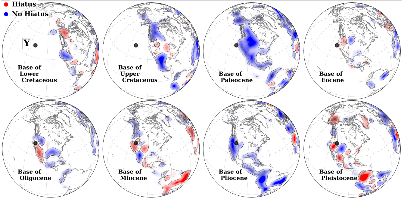
Figure 4: Same as figure 3, but centred on North America. Each BHS map serves as a proxy for paleotopography (red=high, blue=low) in the preceding geological series (see text). Black dot is current Yellowstone (Y) hotspot location [57]. From the Base of Eocene to Base of Miocene hiatus signal surrounds the current location of Yellowstone.
