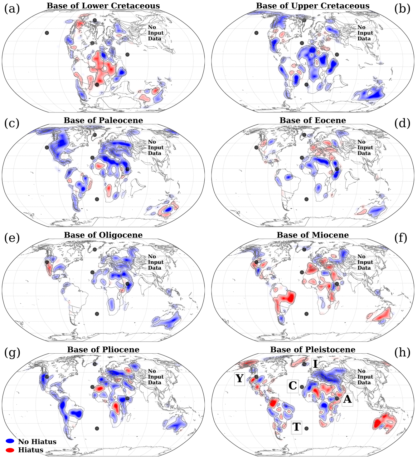
Figure 3: Base Hiatus Surfaces (BHS) from Hayek et al. [45, 46] for eight geological series from Base of Lower Cretaceous to Base of Pleistocene (a)-(h) reconstructed paleogeographically with a global Mesozoic-Cenozoic plate motion model [27] tied to a reference frame of global moving hotspot and a True Polar Wander (TPW) corrected paleomagnetic reconstruction [56], with the latter updated by Seton et al. [55] (see text), and placed into a plate tectonic configuration corresponding to the base of each geological series. Red/blue colours represent the hiatus/no hiatus surfaces. Black dotted lines contour the spherical harmonics signal at the \pm 0.1 amplitude. Each map serves as a proxy for paleotopography (red=high, blue=low) in the preceding series (see text). Black dots are current locations of Yellowstone (Y), Canaries (C), Afar (A), Iceland (I), Tristan (T) hotspot [57].
