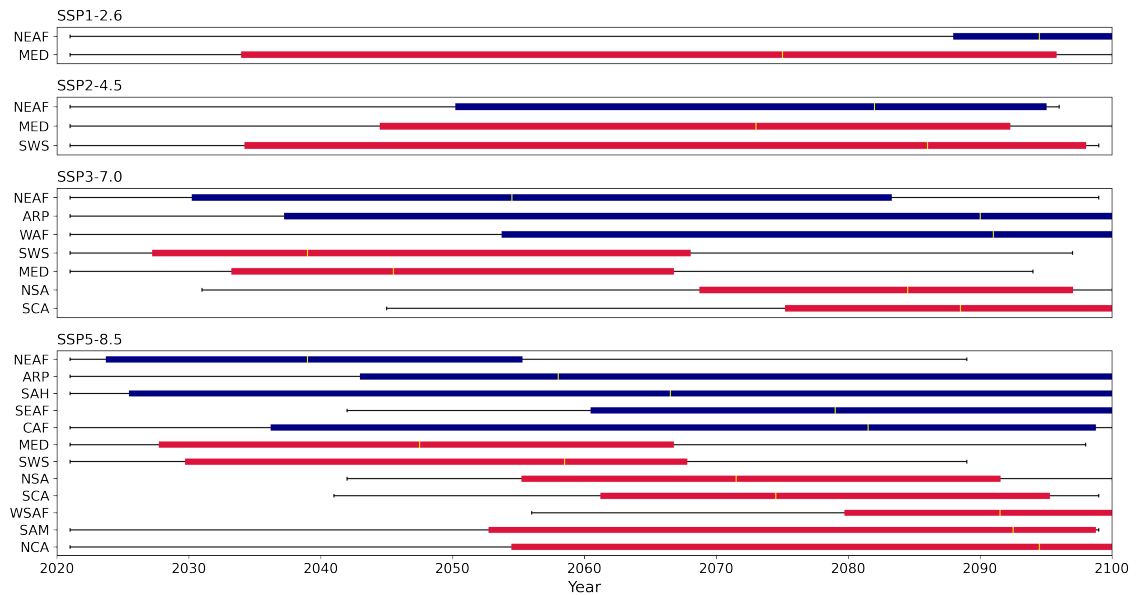
Figure 5. Distribution of the time of emergence of all ESMS for climate regions where more than 50% of the ESMS show a permanent wet (blue) or dry (red) departure in different SSP scenarios within the studied timeframe. The interquartile range is represented by the length of the box, and median by the yellow line within the box.
