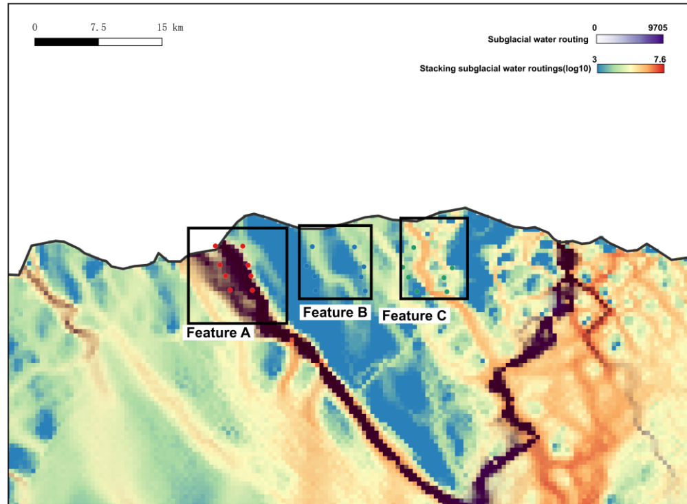
Subglacial water routing results
