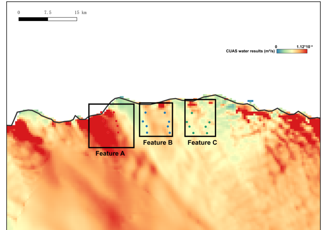
Subglacial water flux results
