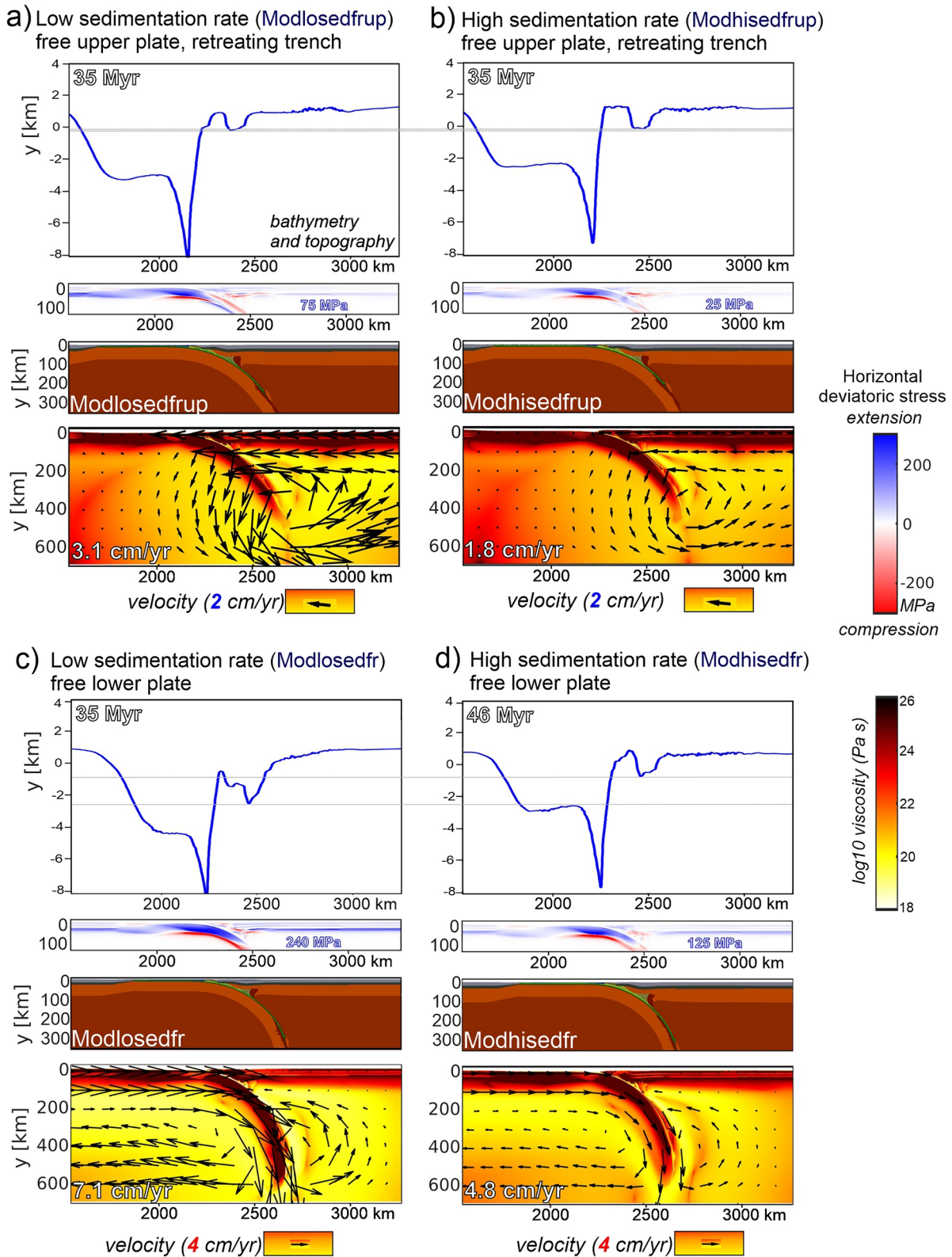
Figure 9. Parameter test on the influence of different erosion and sedimentation rates and convergence kinematics. No velocity boundary conditions are imposed after the slab reaches 380 km depth. (a) Free upper and fixed lower plate and lower sedimentation rate. (b) Free upper and fixed lower plate and higher sedimentation rate. (c) Fixed upper and free lower plate and lower sedimentation rate. (d) Fixed upper and free lower plate and higher sedimentation rate. Higher subduction velocity is reached in the experiment with lower sedimentation and erosion rates. Note the different scales of the velocity vectors.
