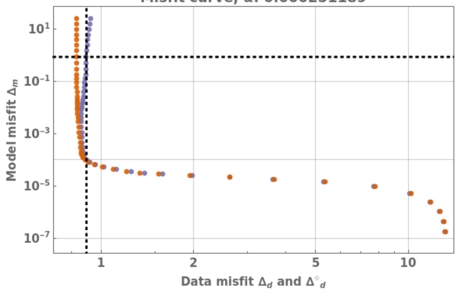
Misfit curve, \alpha: 0.000251189
