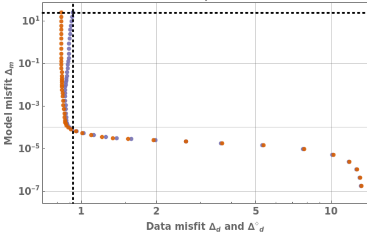
Misfit curve, \alpha: 0.00001
