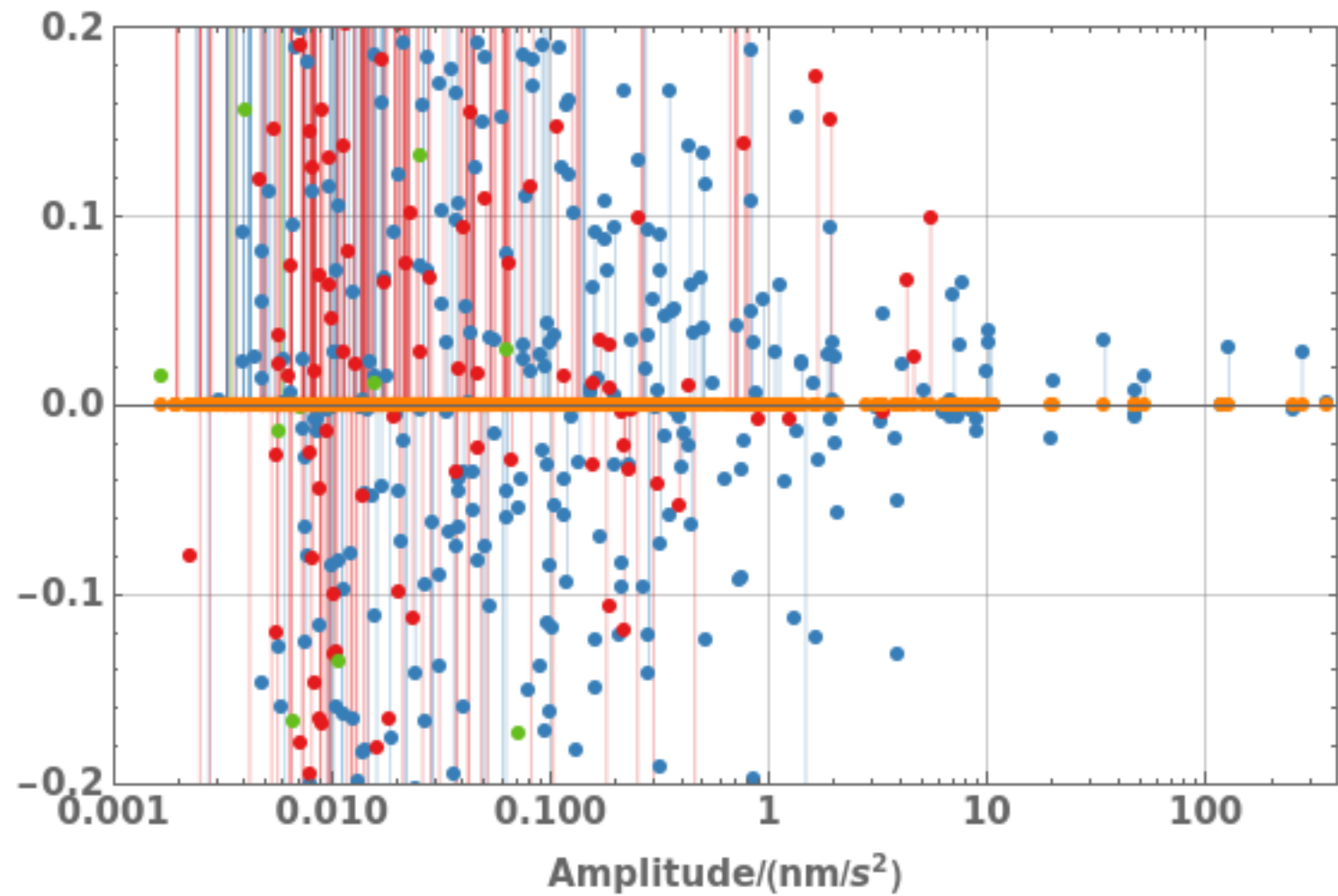
Gravimetric factor difference
