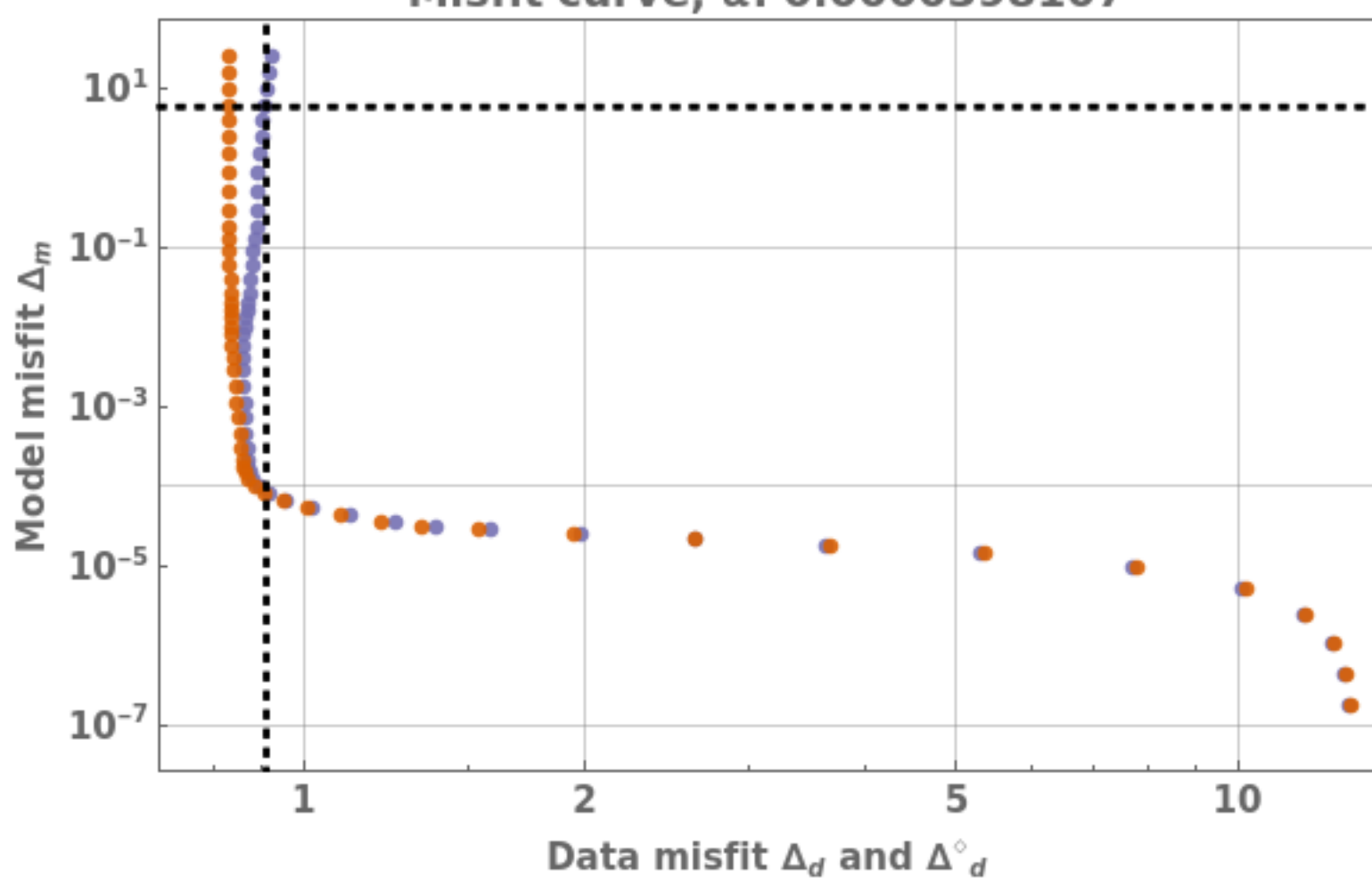
Misfit curve, \alpha: 0.0000398107
