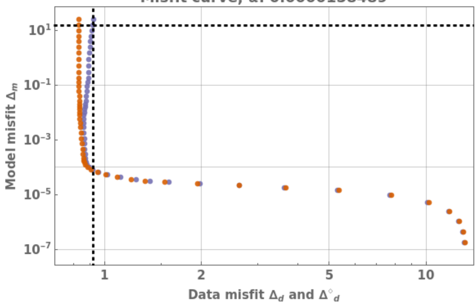
Misfit curve, \alpha : 0.0000158489
