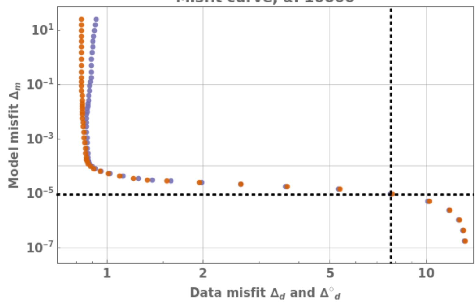
Misfit curve, \alpha: 10000
