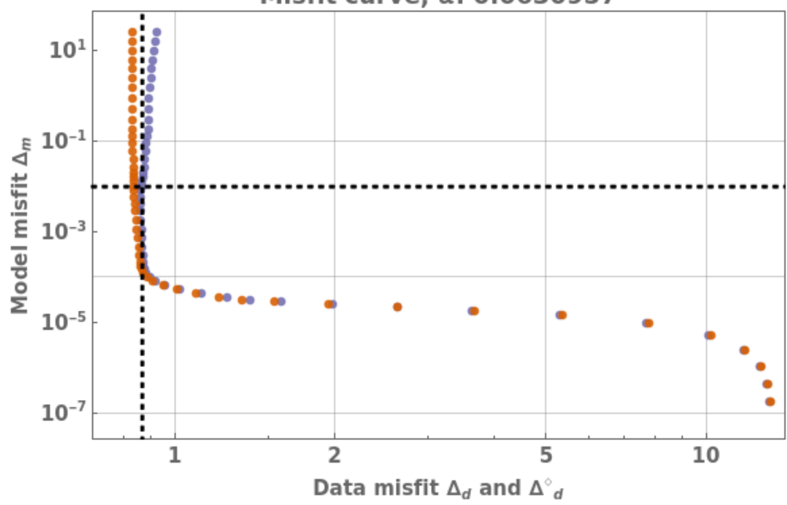
Misfit curve, \alpha: 0.0630957
