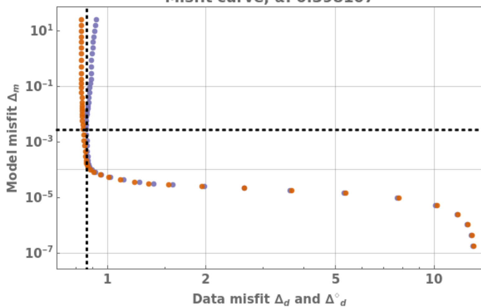
Misfit curve, \alpha: 0.398107
