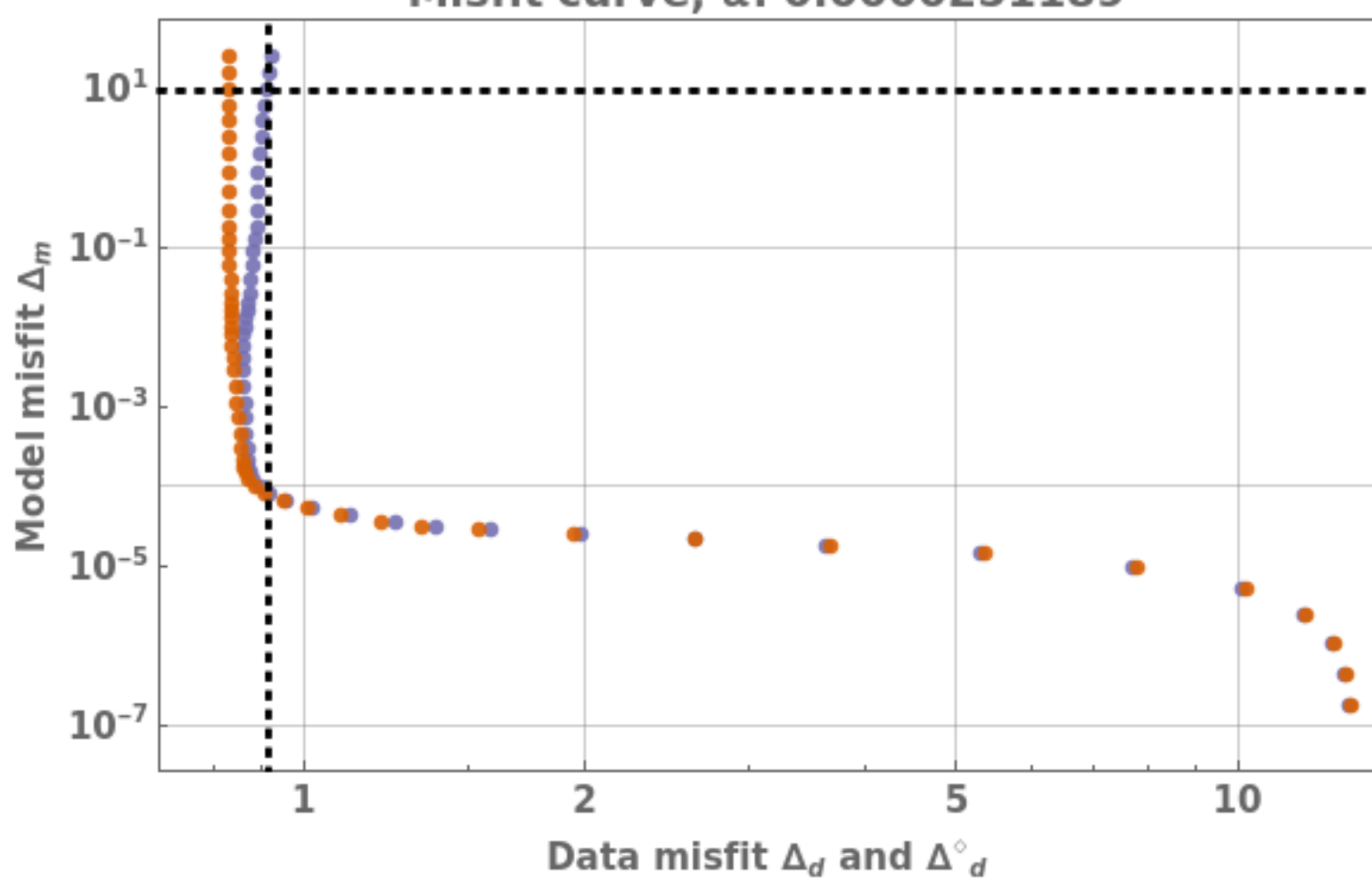
Misfit curve, \alpha: 0.0000251189
