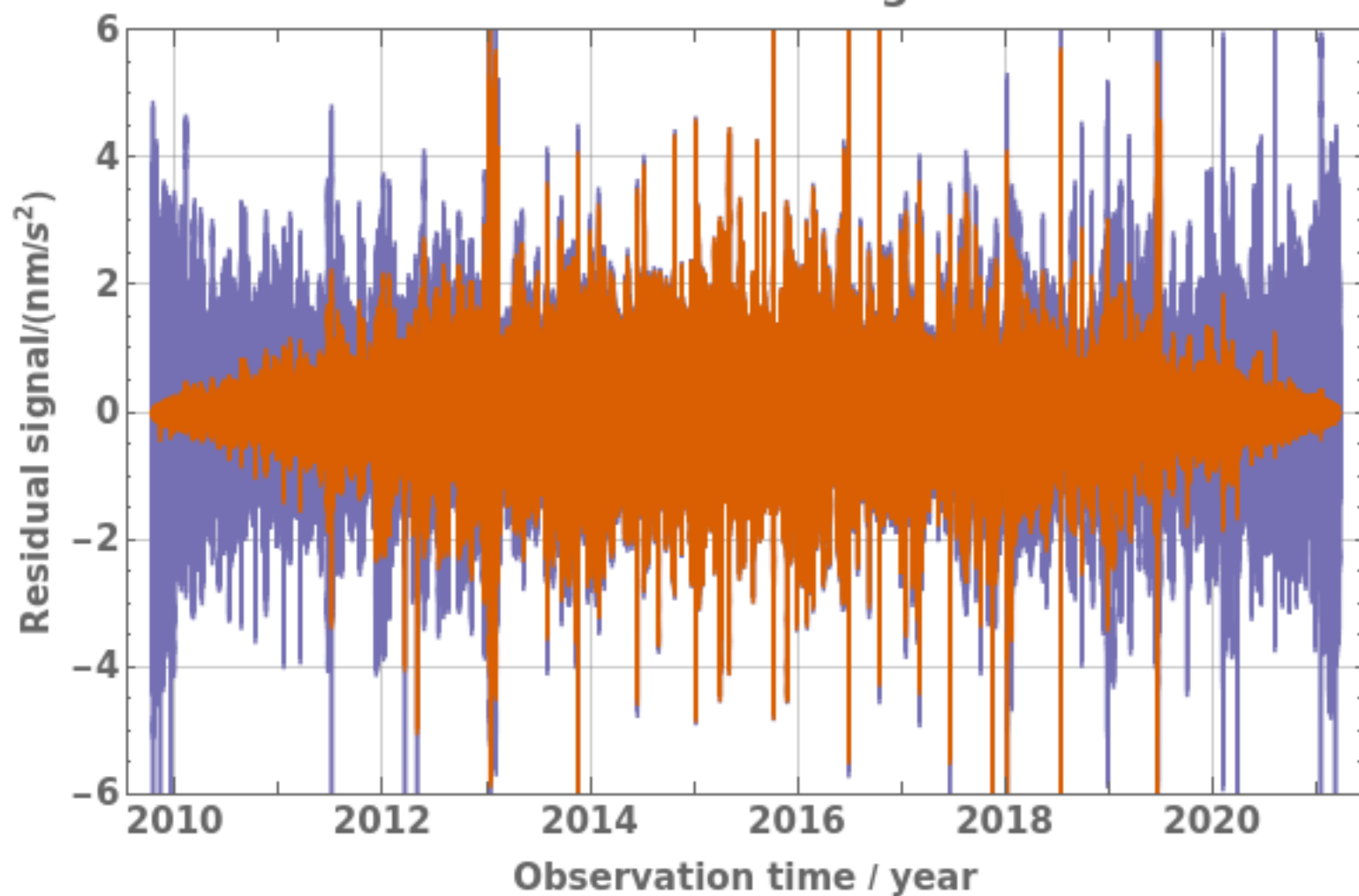
Data residual signal
