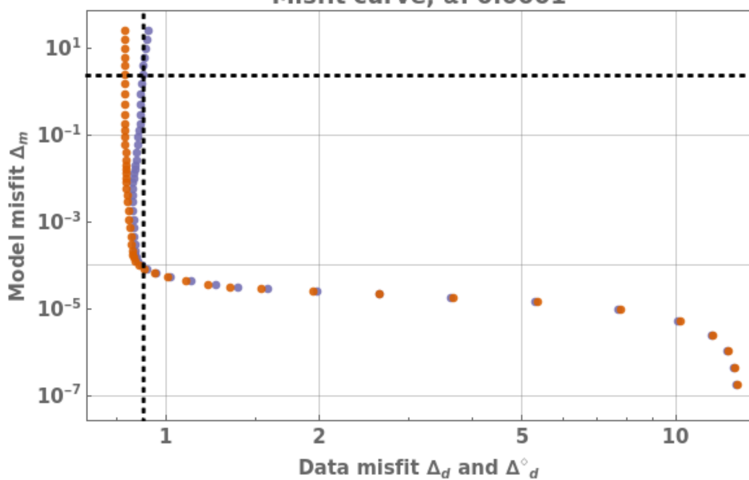
Misfit curve, \alpha: 0.0001
