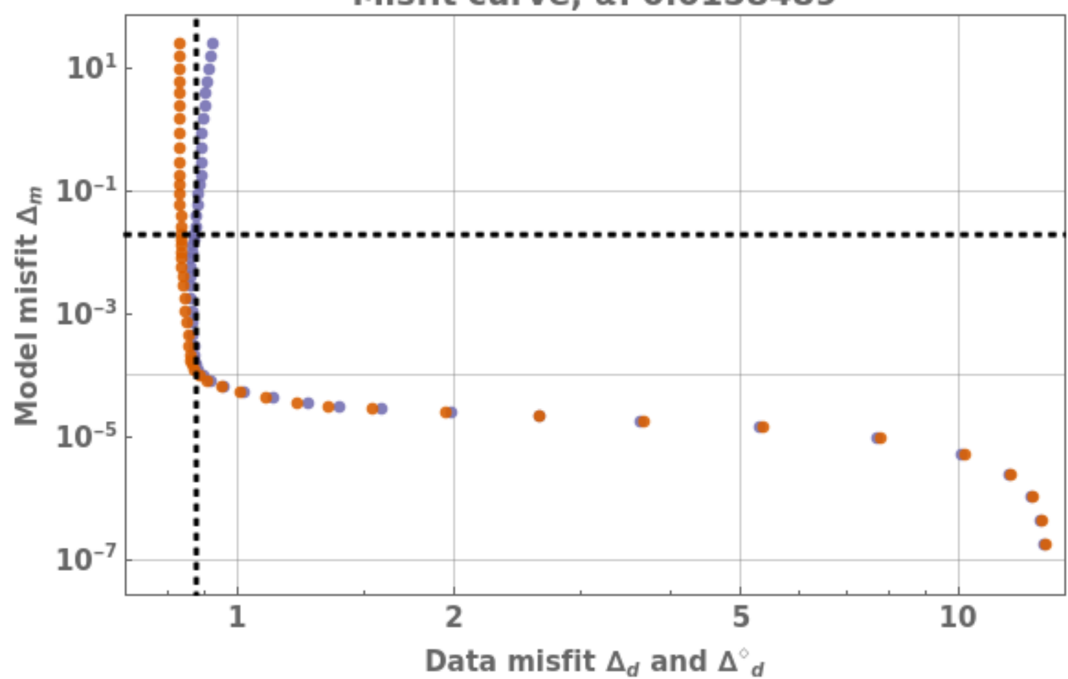
Misfit curve, \alpha : 0.0158489
