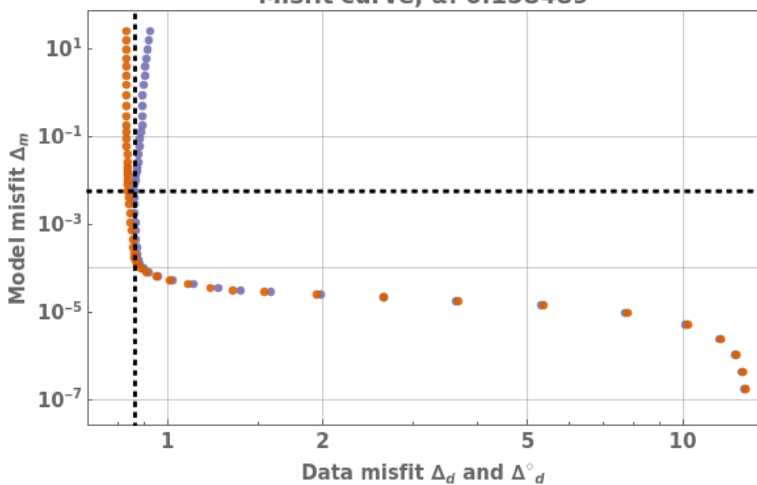
Misfit curve, \alpha: 0.158489
