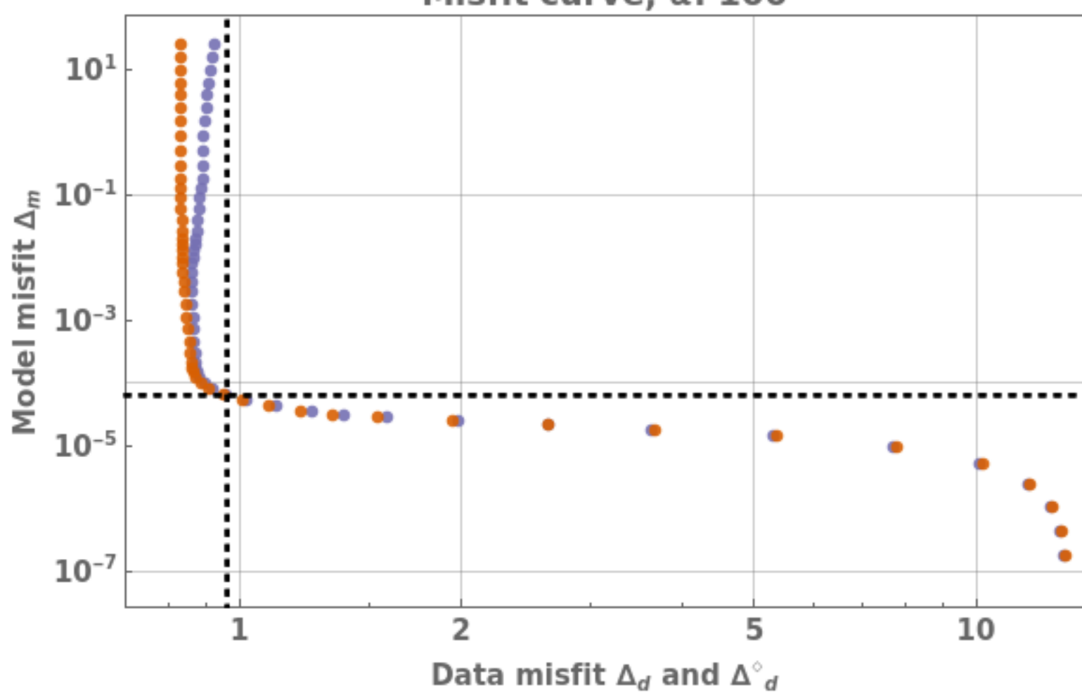
Misfit curve, \alpha: 100
