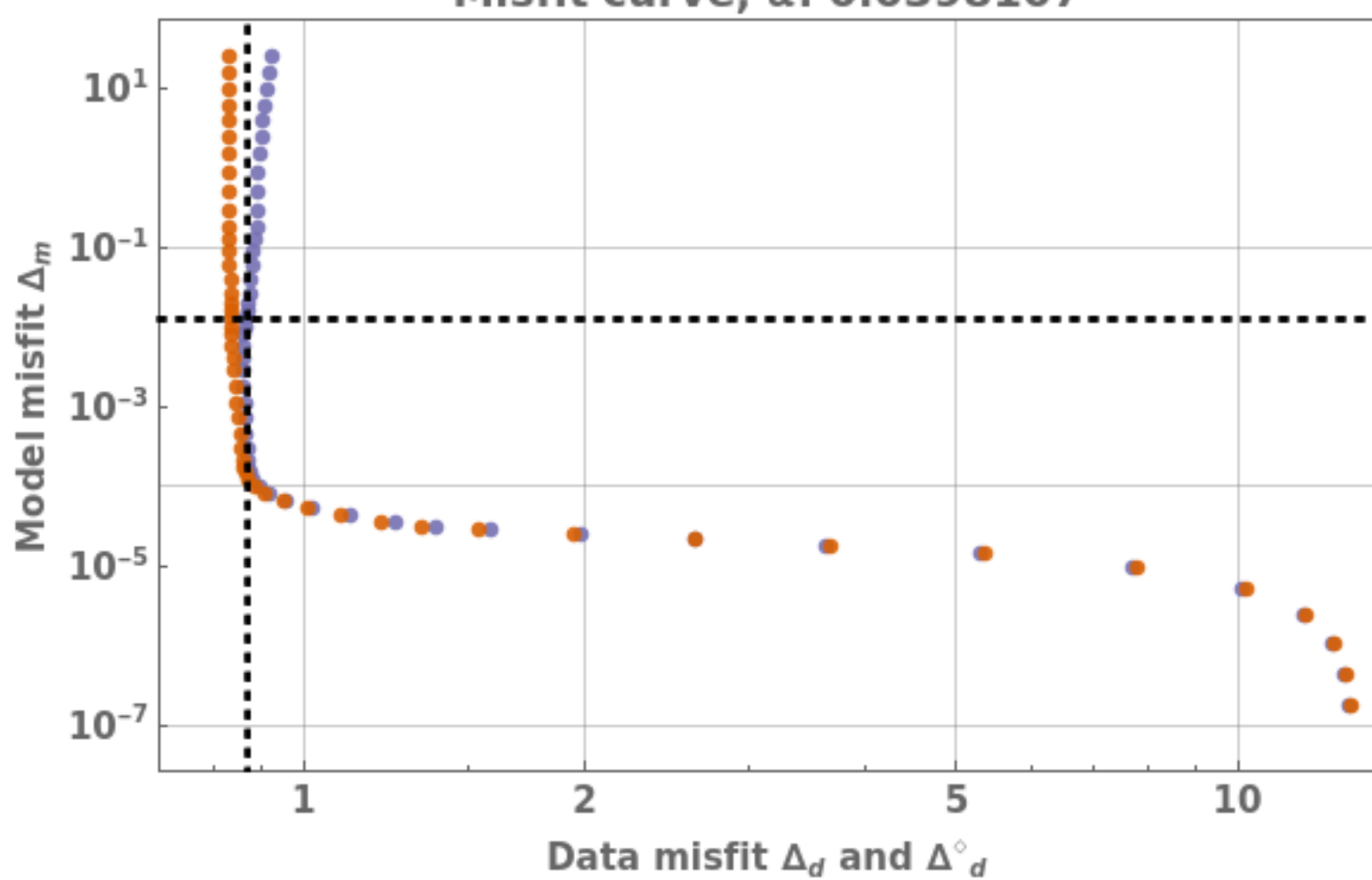
Misfit curve, \alpha : 0.0398107
