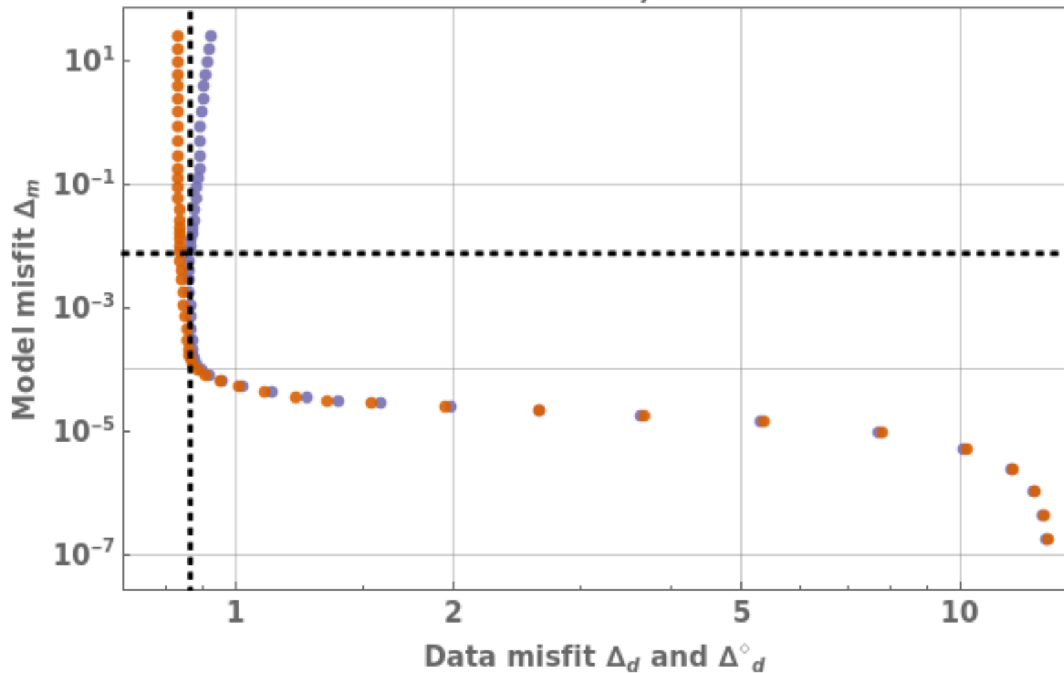
Misfit curve, \alpha: 0.1
