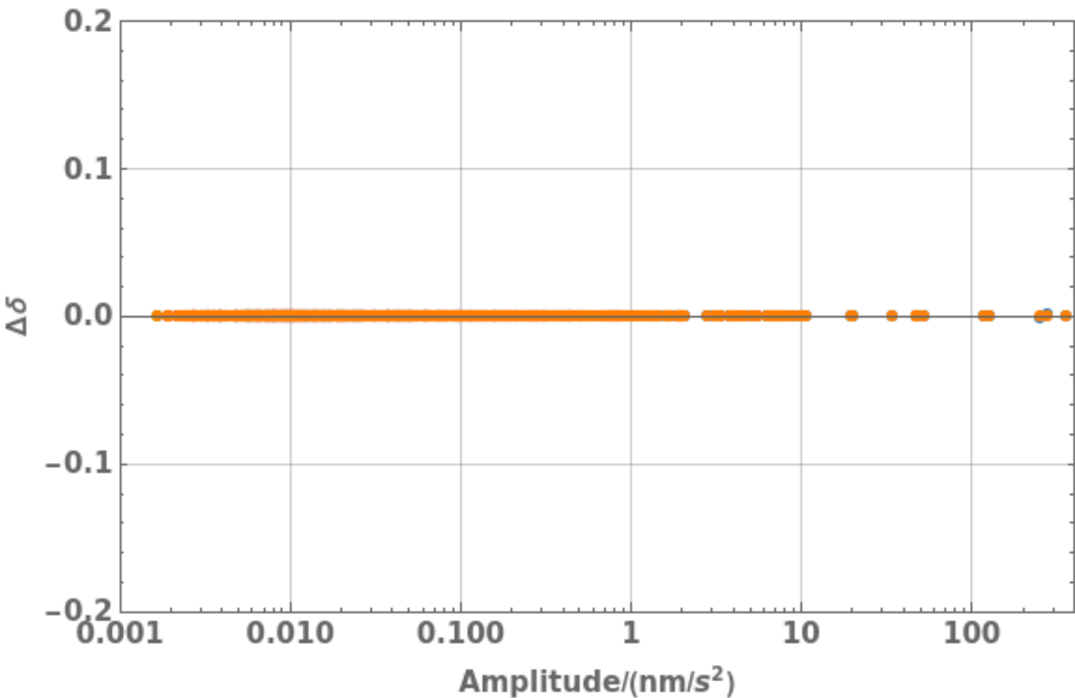
Gravimetric factor difference
