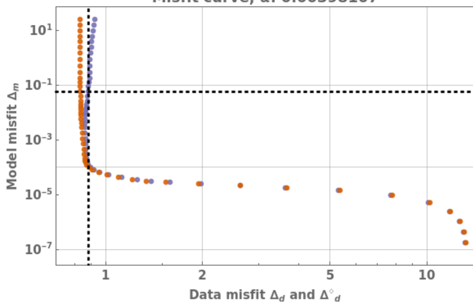
Misfit curve, \alpha: 0.00398107
