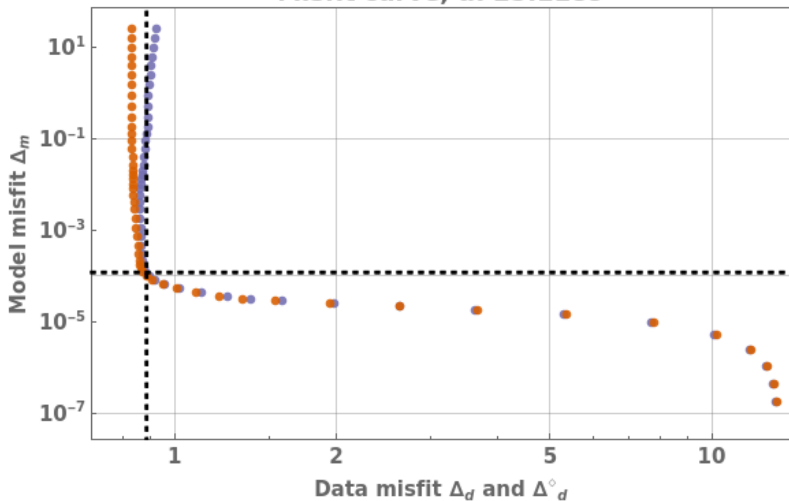
Misfit curve, \alpha : 25.1189
