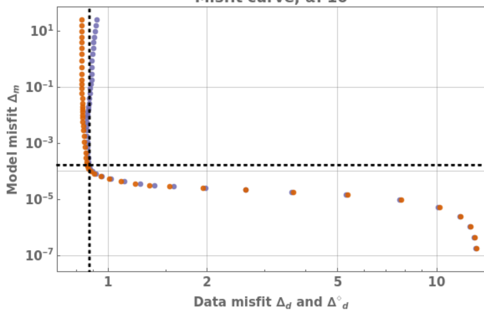
Misfit curve, \alpha: 10
