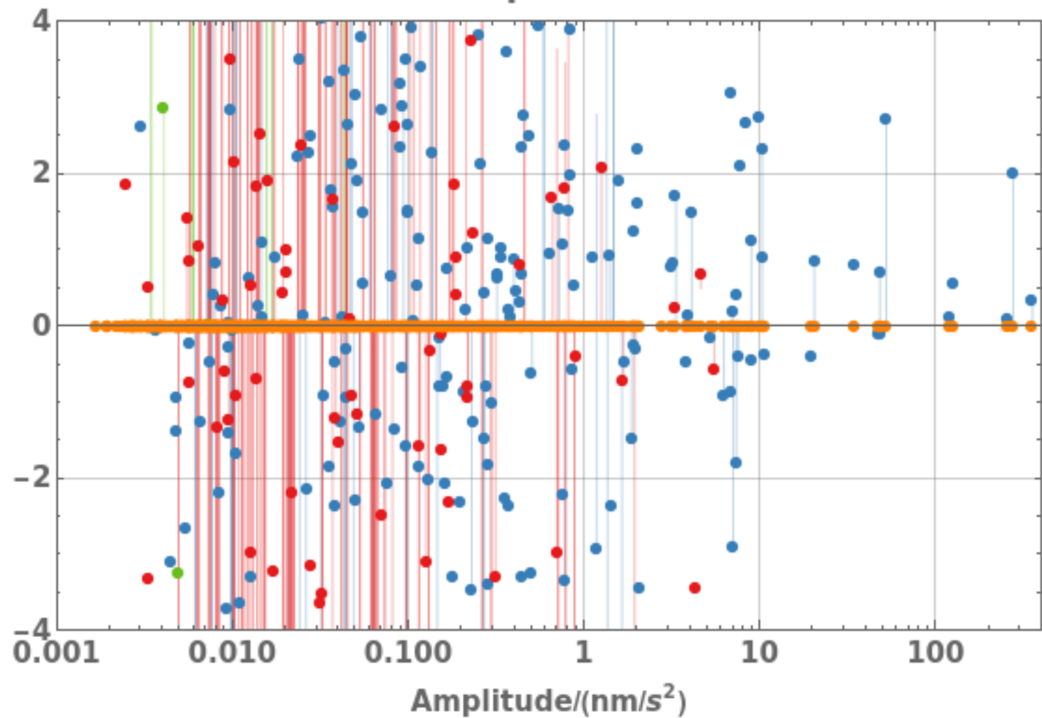
Gravimetric phase difference
