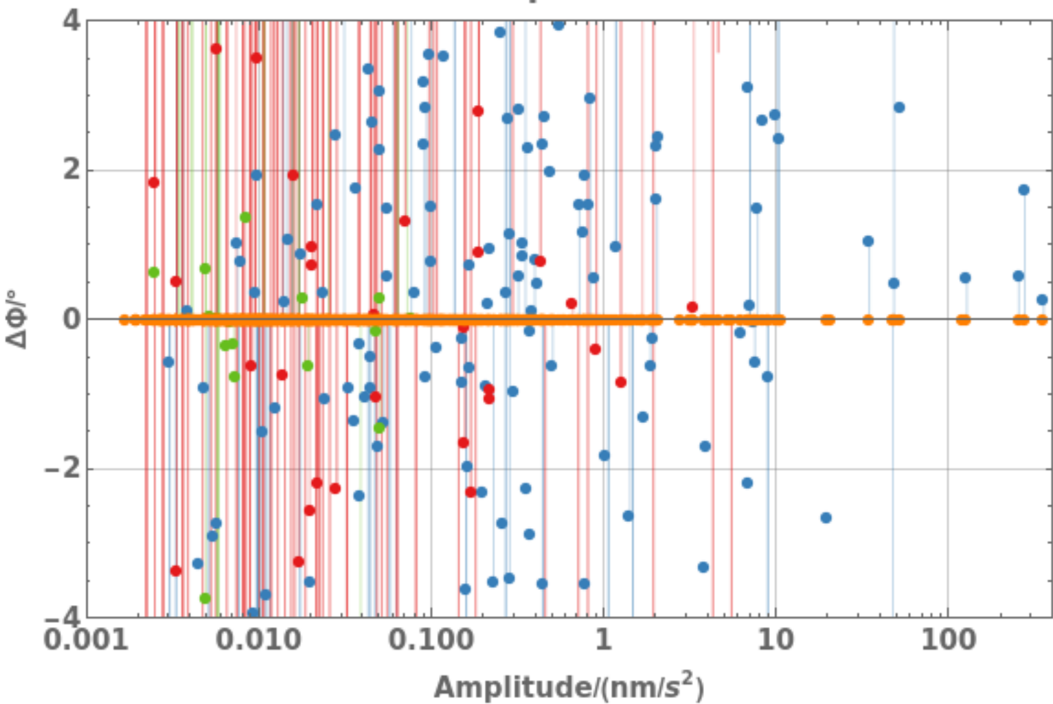
Gravimetric phase difference
