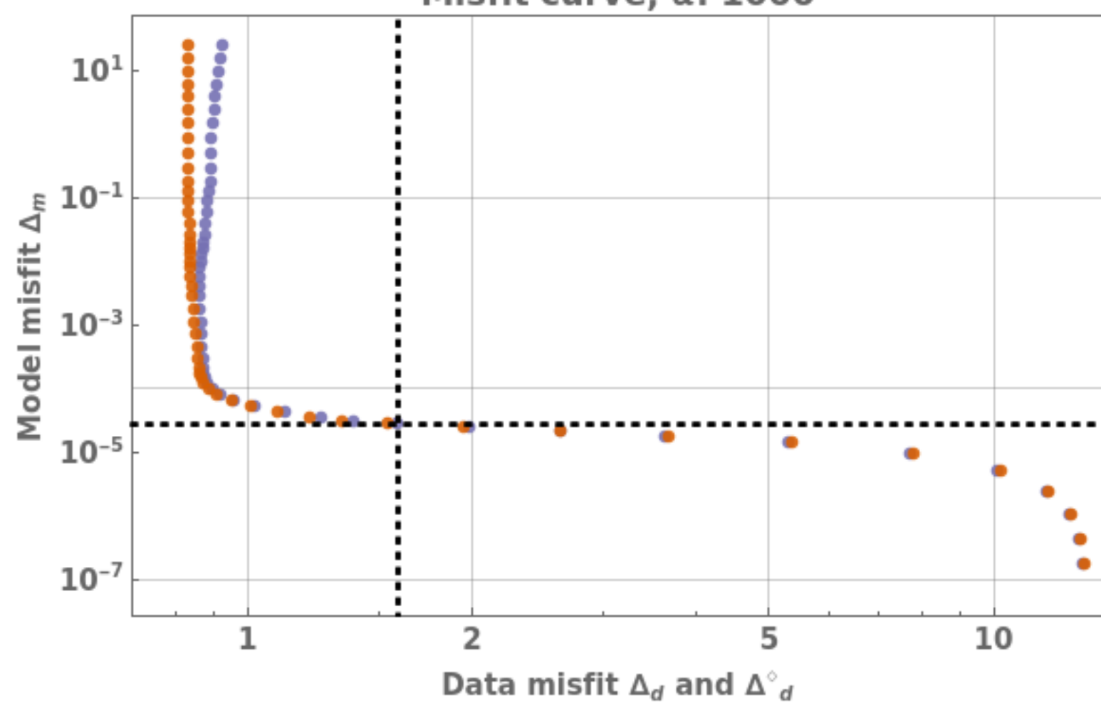
Misfit curve, \alpha: 1000
