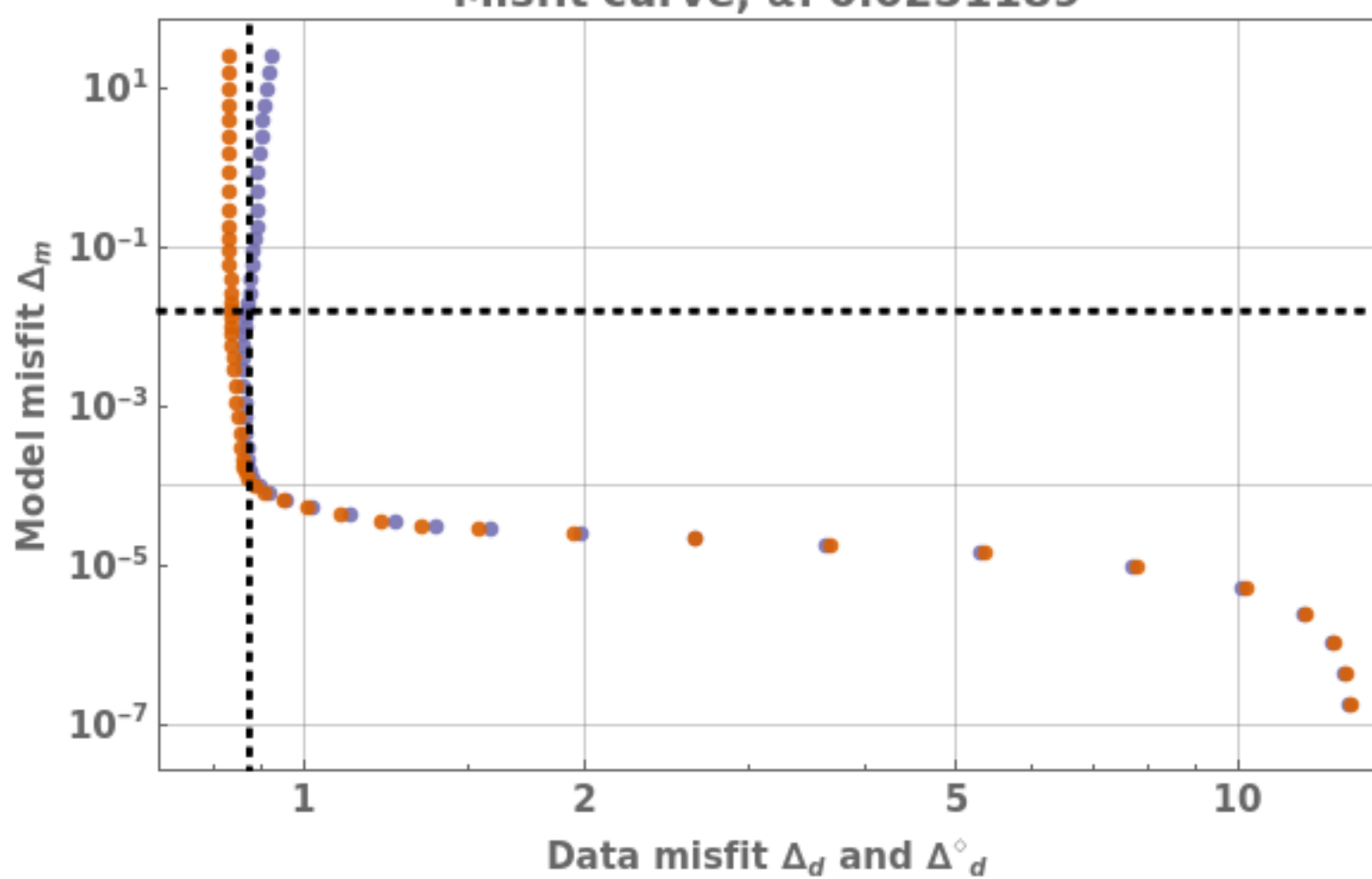
Misfit curve, \alpha : 0.0251189
