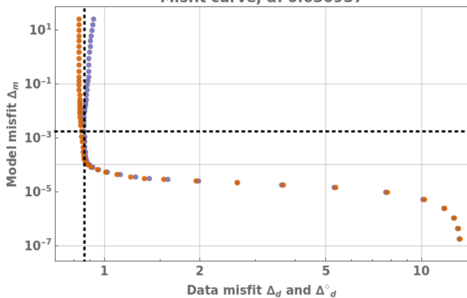
Misfit curve, \alpha: 0.630957
