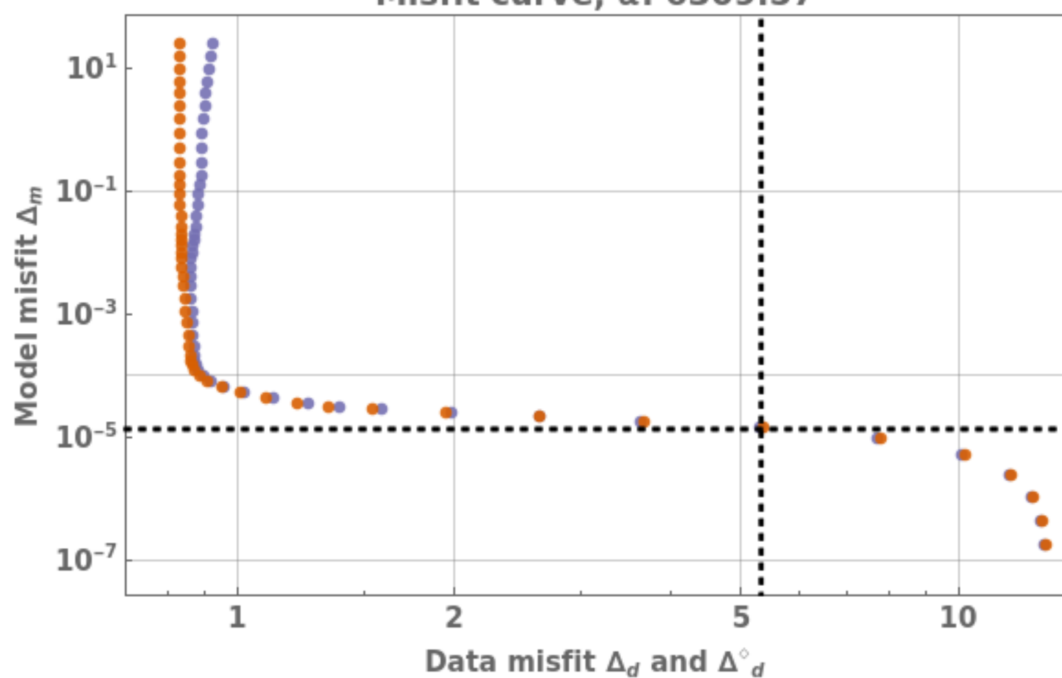
Misfit curve, \alpha : 6309.57
