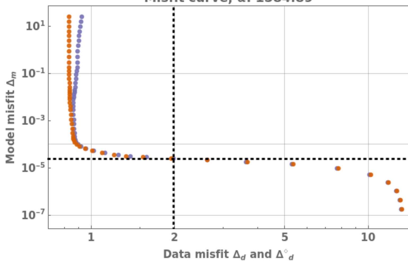
Misfit curve, \alpha : 1584.89
