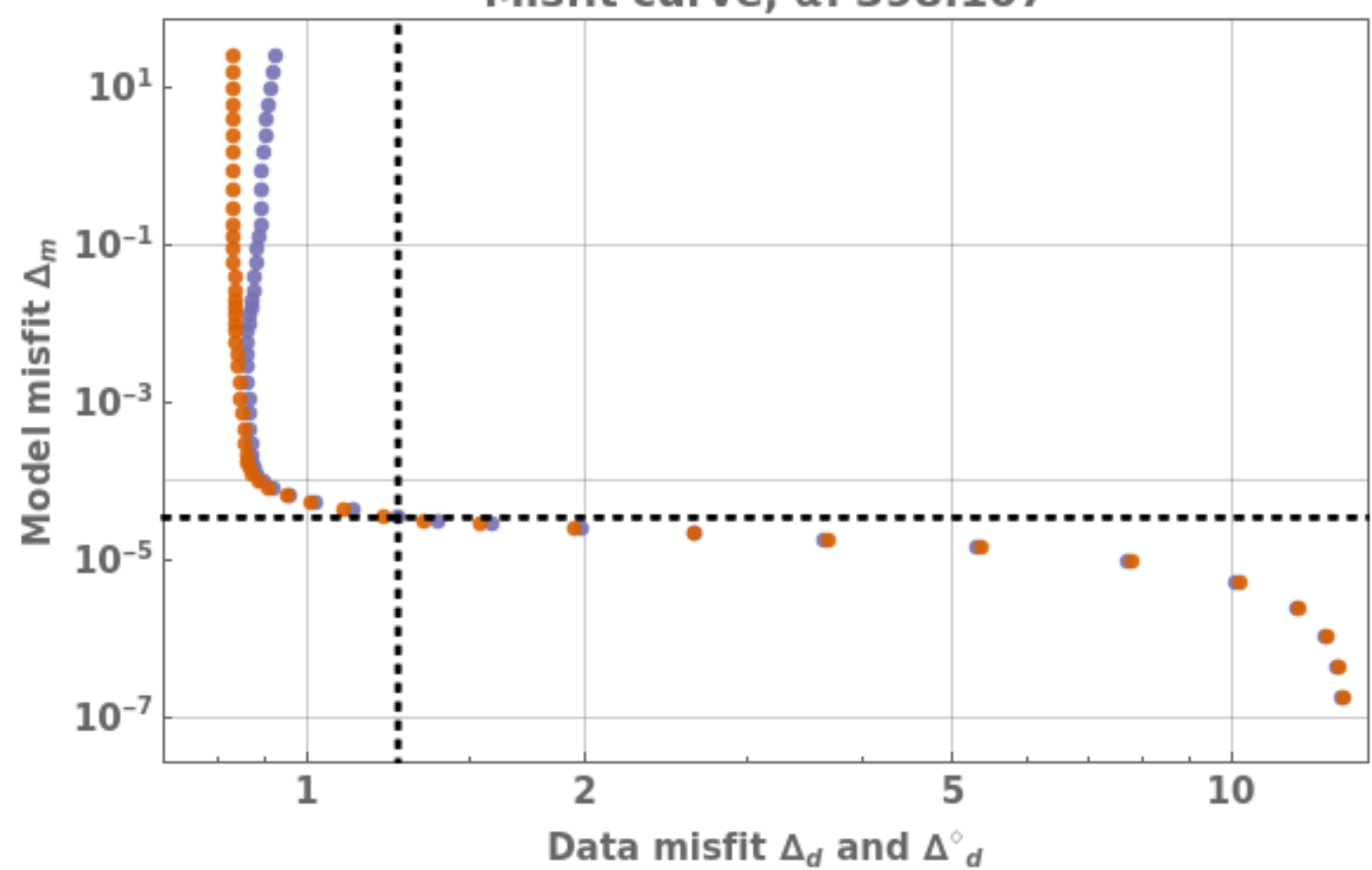
Misfit curve, \alpha : 398.107
