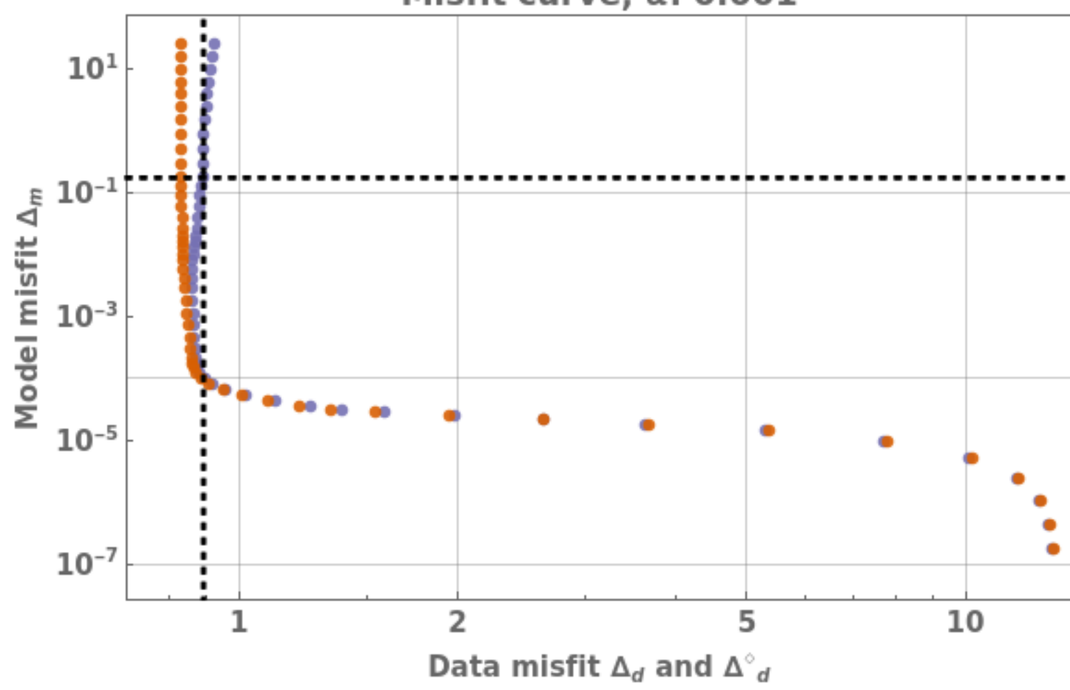
Misfit curve, \alpha: 0.001
