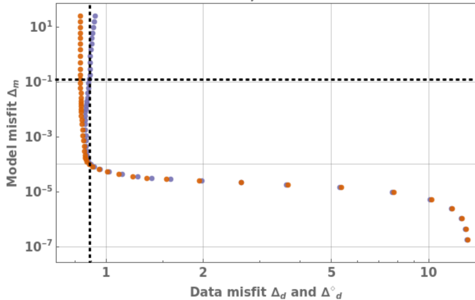
Misfit curve, \alpha: 0.00158489
