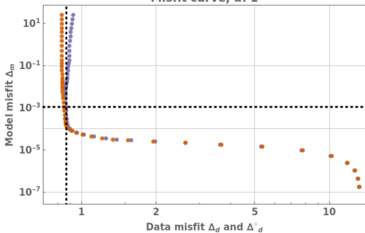
Misfit curve, \alpha: 1
