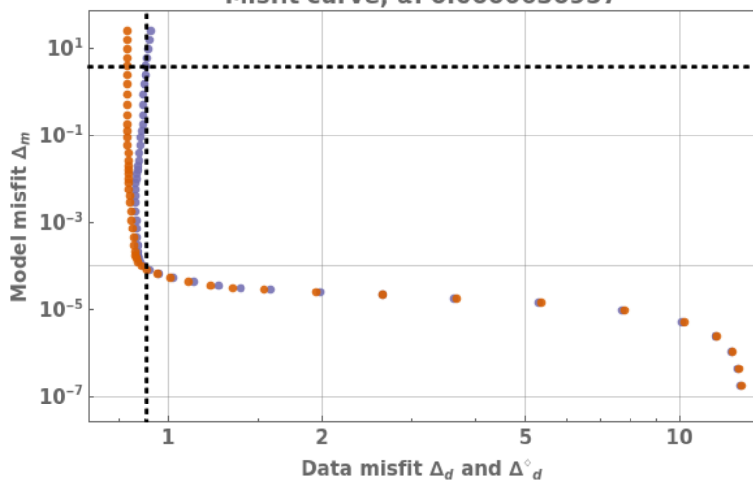
Misfit curve, \alpha: 0.0000630957
