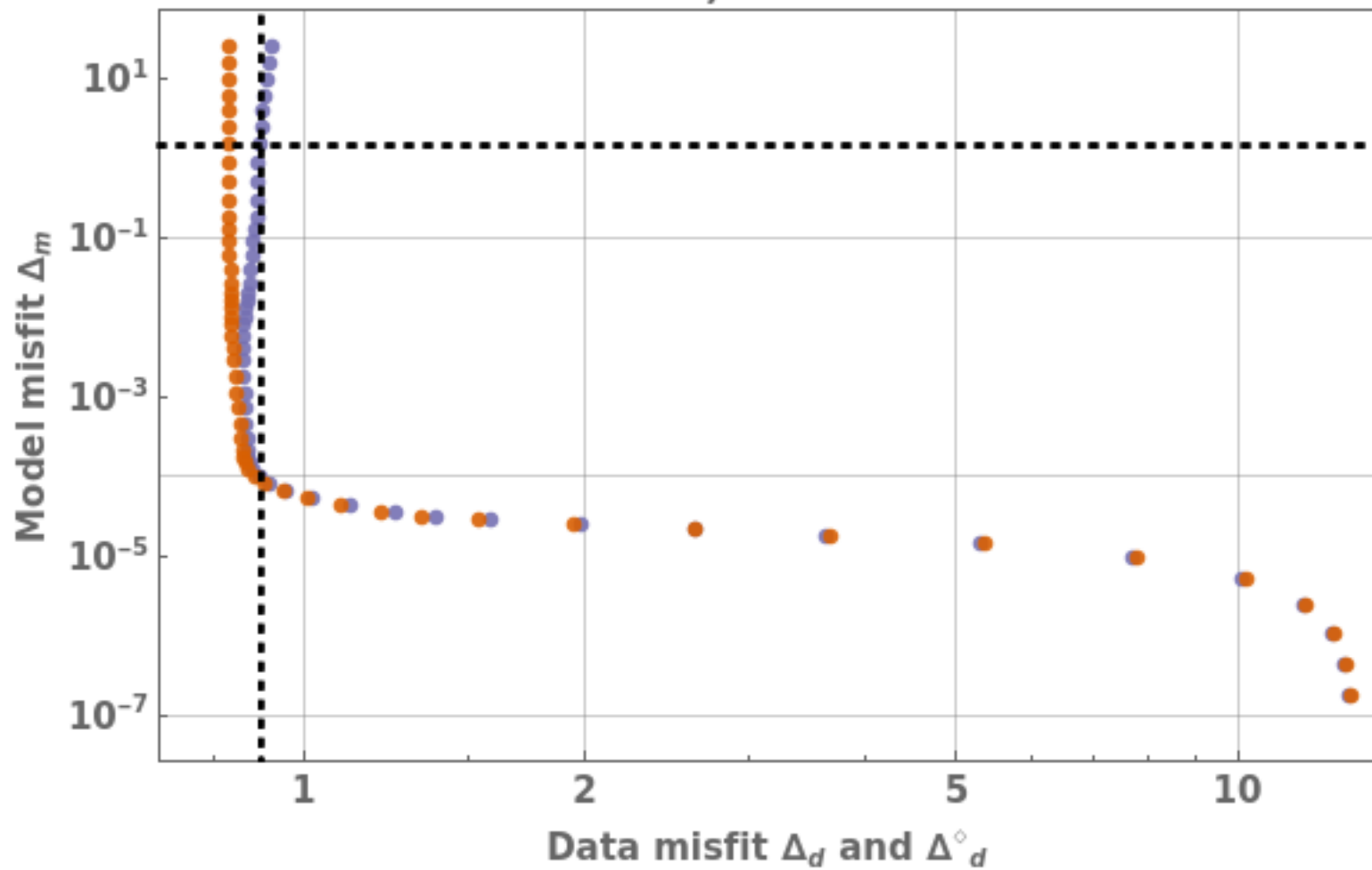
Misfit curve, \alpha : 0.000158489
