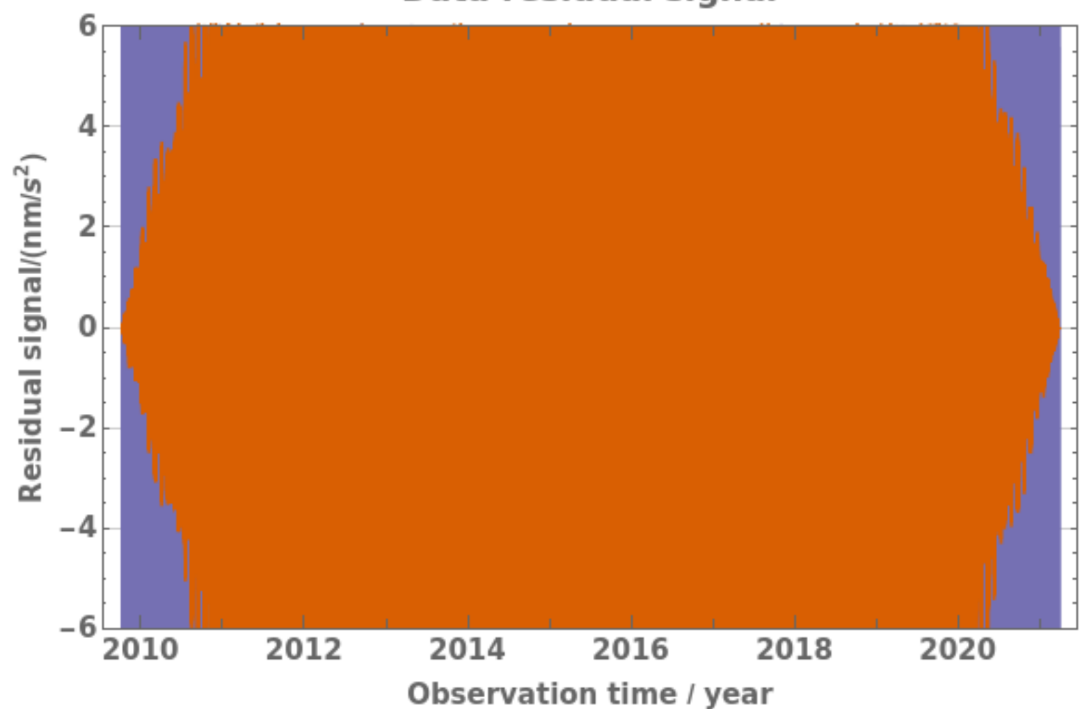
Data residual signal
