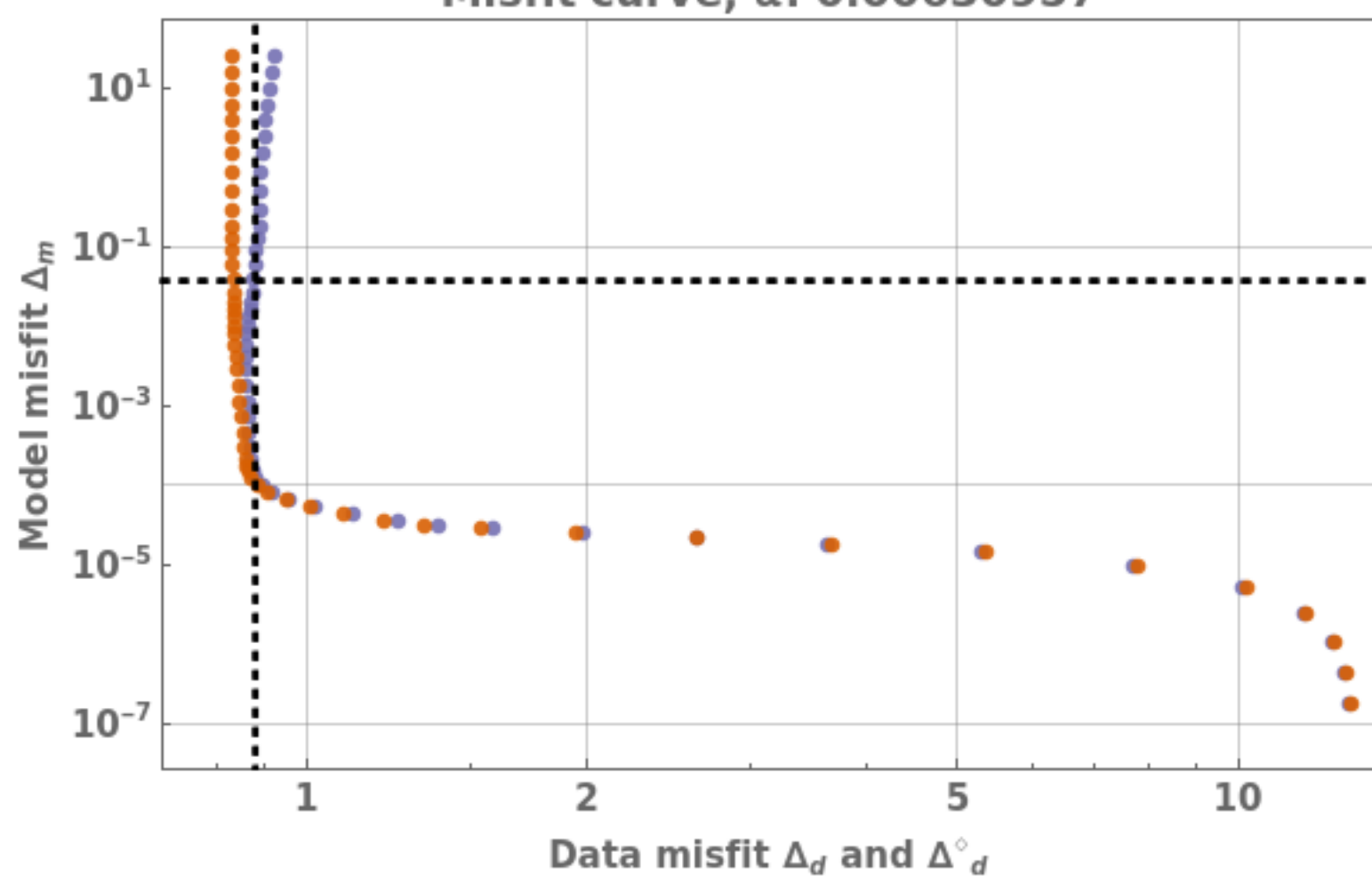
Misfit curve, \alpha: 0.00630957
