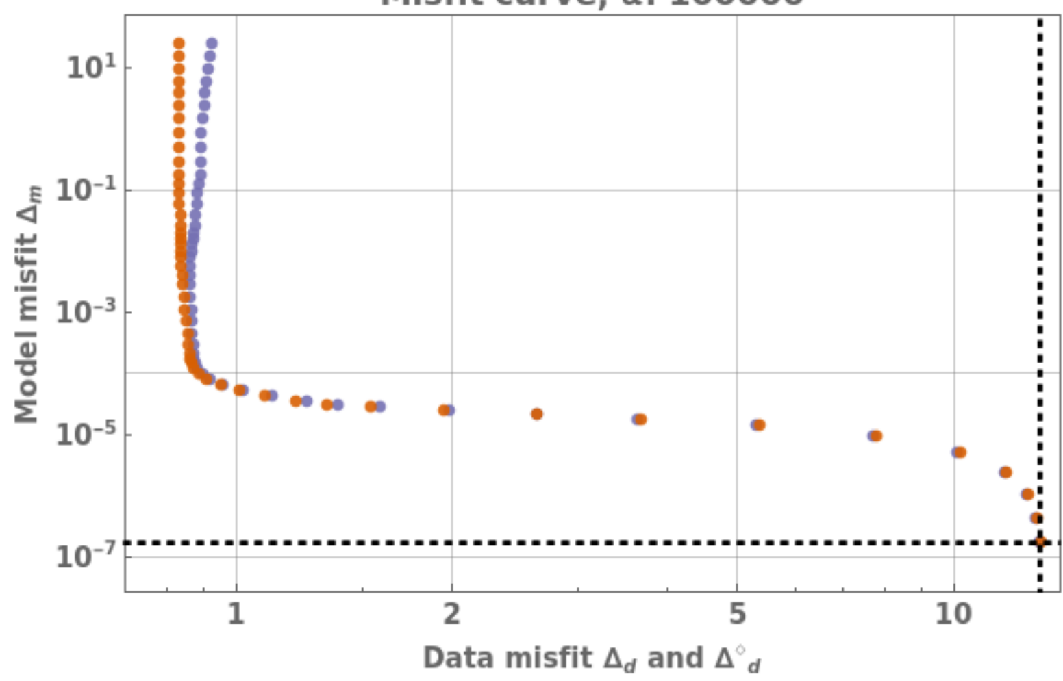
Misfit curve, \alpha: 100000
