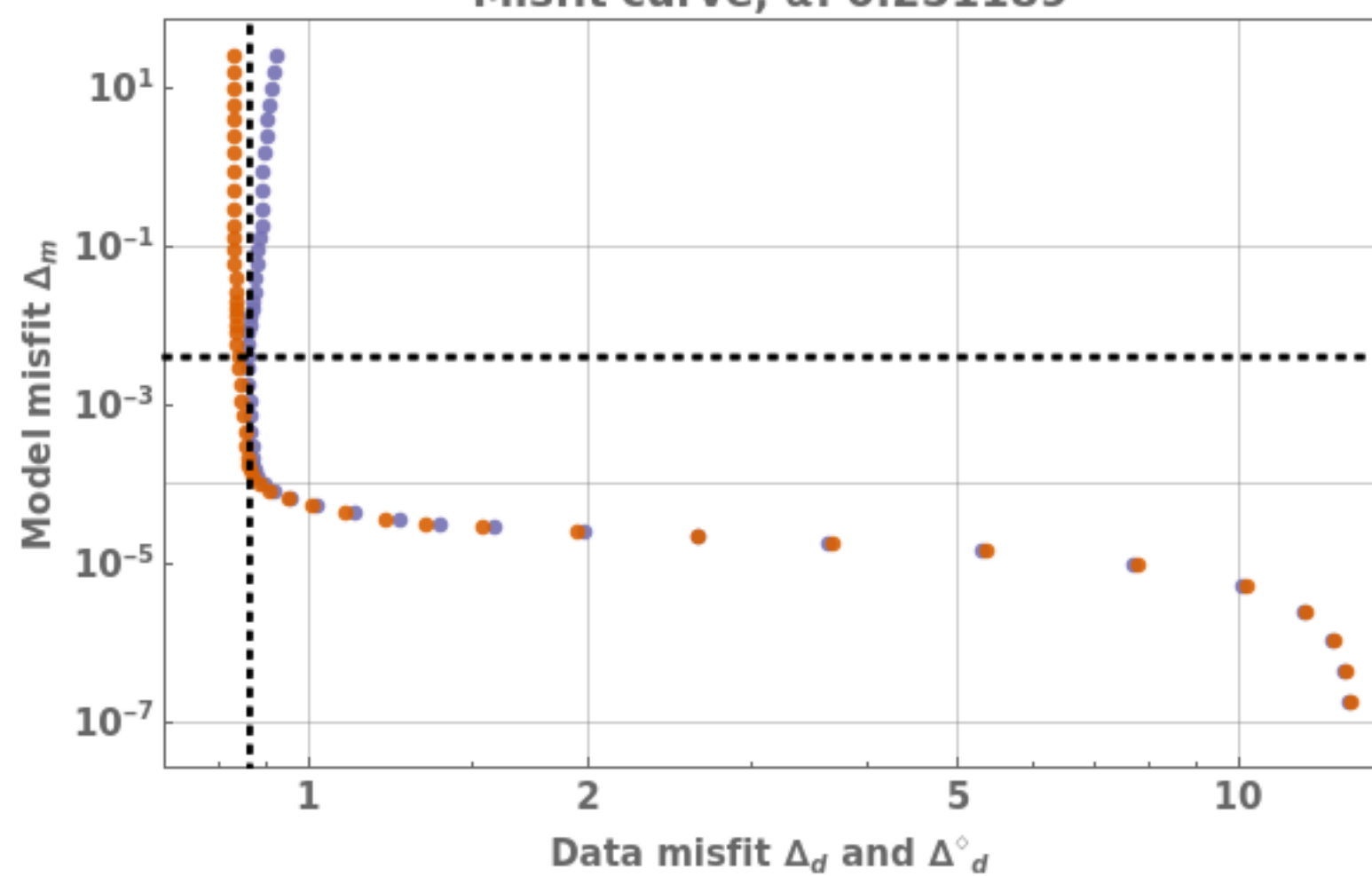
Misfit curve, \alpha: 0.251189
