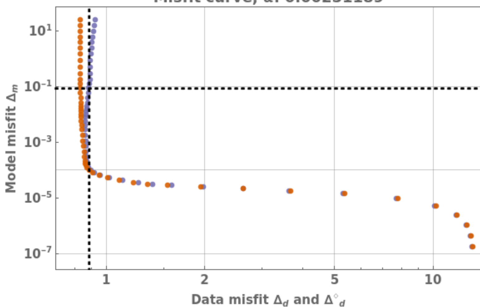
Misfit curve, \alpha: 0.00251189
