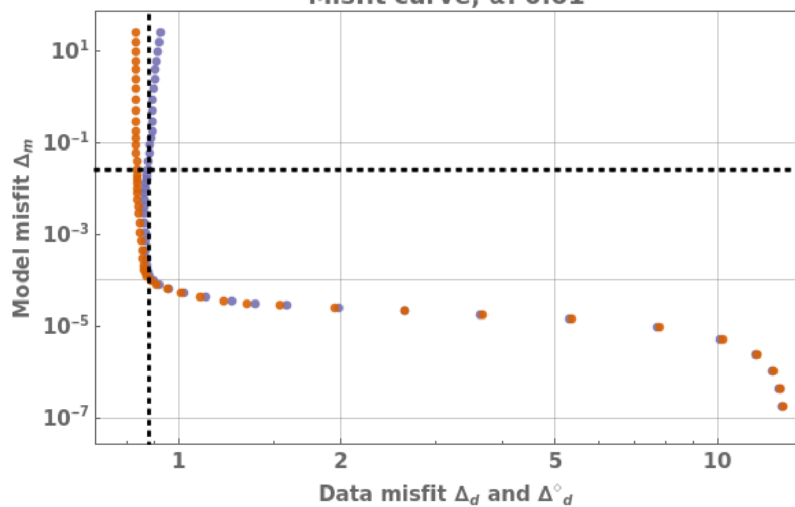
Misfit curve, \alpha: 0.01
