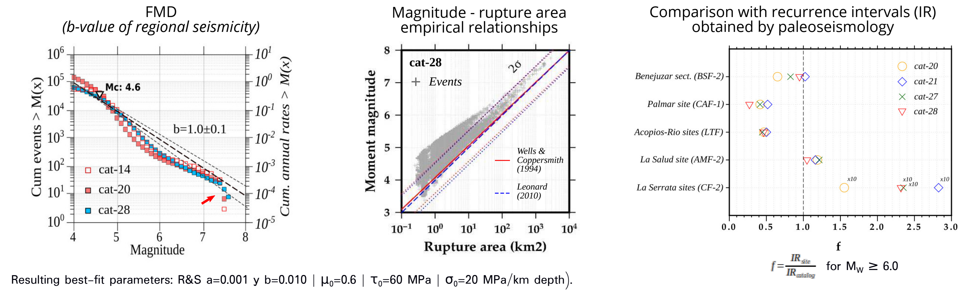
Resulting best-fit parameters: R&S a=0.001 y b=0.010 | \mu_0=0.6 | \tau_0=60 MPa | \sigma_0=20 MPa/km depth.
