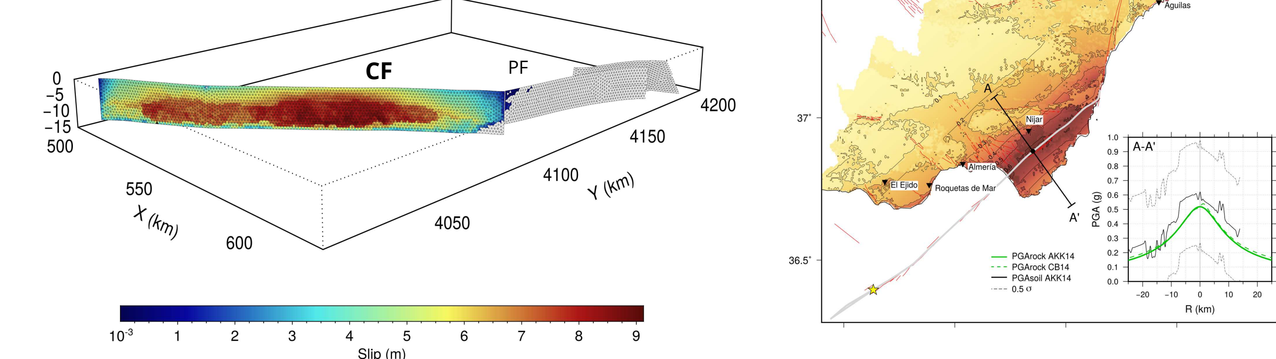
Example of maximum scenario M_w 7.6 on the Carboneras Fault (SW of the EBFS). Being a subvertical fault, the largest PGA are concentrated on both sides of the fault trace, exceeding 0.5 g in areas with soft clayey soils.
