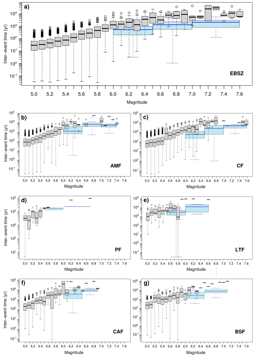
Figure 6. Interevent time distribution according to moderate-large moment magnitudes simulated on (a) the complete fault system and, (b) to (g), on each fault. The gray box lies between the upper and lower quartiles of the data, the black line inside the box indicate the median value, the dashed lines represent maximum and minimum values, and the isolated circles are the outliers. The blue boxes show interevent times for less frequent M \geq 6 earthquakes ( M \geq 5.5 for PF and LTF) considering a larger magnitude bin. Events with an intermediate time less than 10 days have been discarded to avoid a clustering effect.
