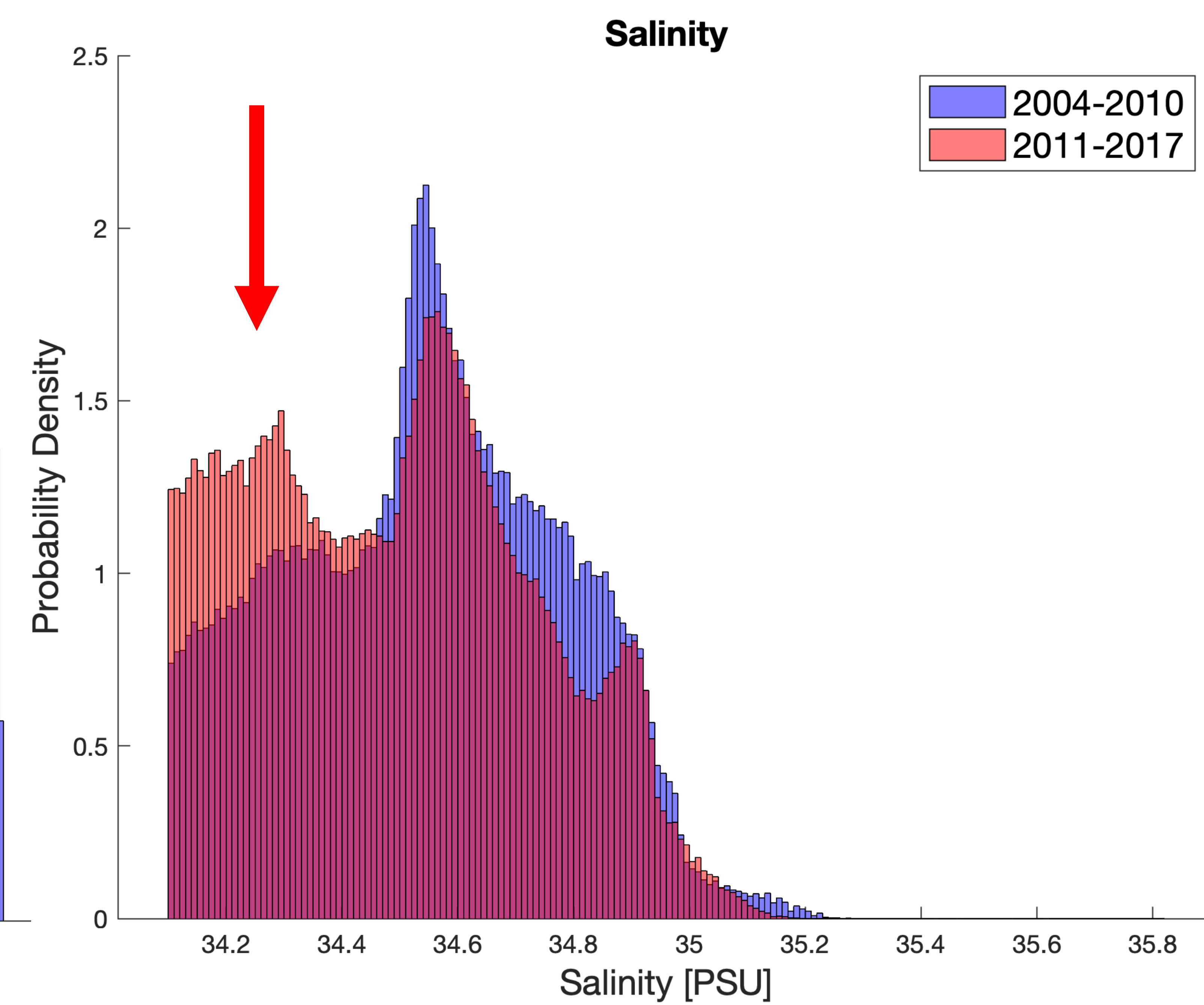
West Greenland Irminger (Atlantic) Water
