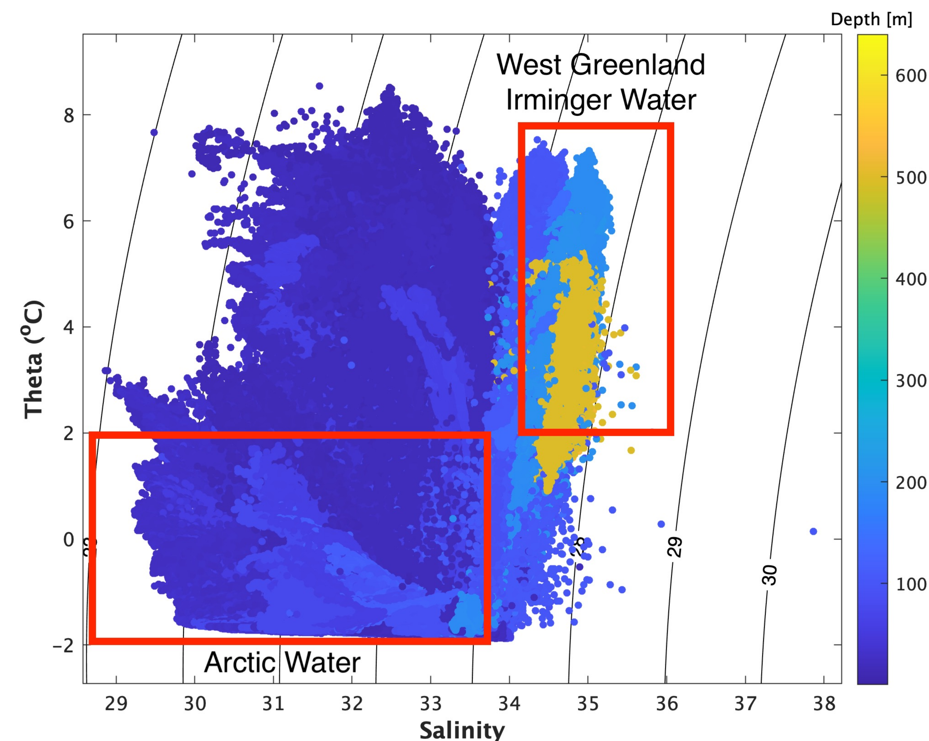
Key Davis Strait Water Masses
