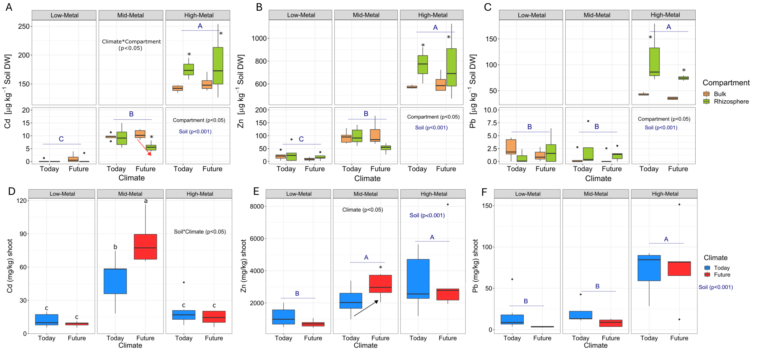
Figure S1. CaCl 2 extractable metal concentrations in soils (A-C); metal accumulation in shoots (D-F).
