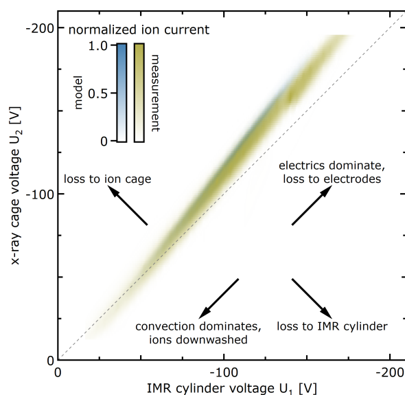
Figure 8. Sensitivity of pinhole \text{NO}_3^- current towards IMR cylinder voltage U_1 and ion cage voltage U_2 in Eisele type inlet. Ion transport to the IMR and pinhole is only significant for a narrow combination of voltages that cause substantial electrophoretic transport while minimising surface losses.
