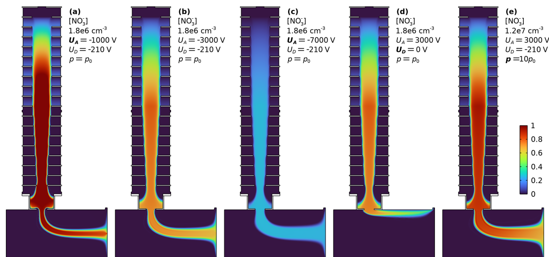
Figure 4. Sensitivities of \text{NO}_3^- concentrations in MION2 inlet to different acceleration voltages U_A (A–C), deflector voltage U_D = 0 for deactivation (D), and primary ion production rate (E). The colour scale ranges from 0 to the maximum described in each panel. Figures A–D use the same colour scale. The width of the ion beam increases for larger voltages, while the extracted concentrations slightly decrease. At concentrations of 10^7 \text{ cm}^{-3} space charge leads to a spreading of the ion beam, the concentration at the pinhole is lower than at the ionisation volume.
