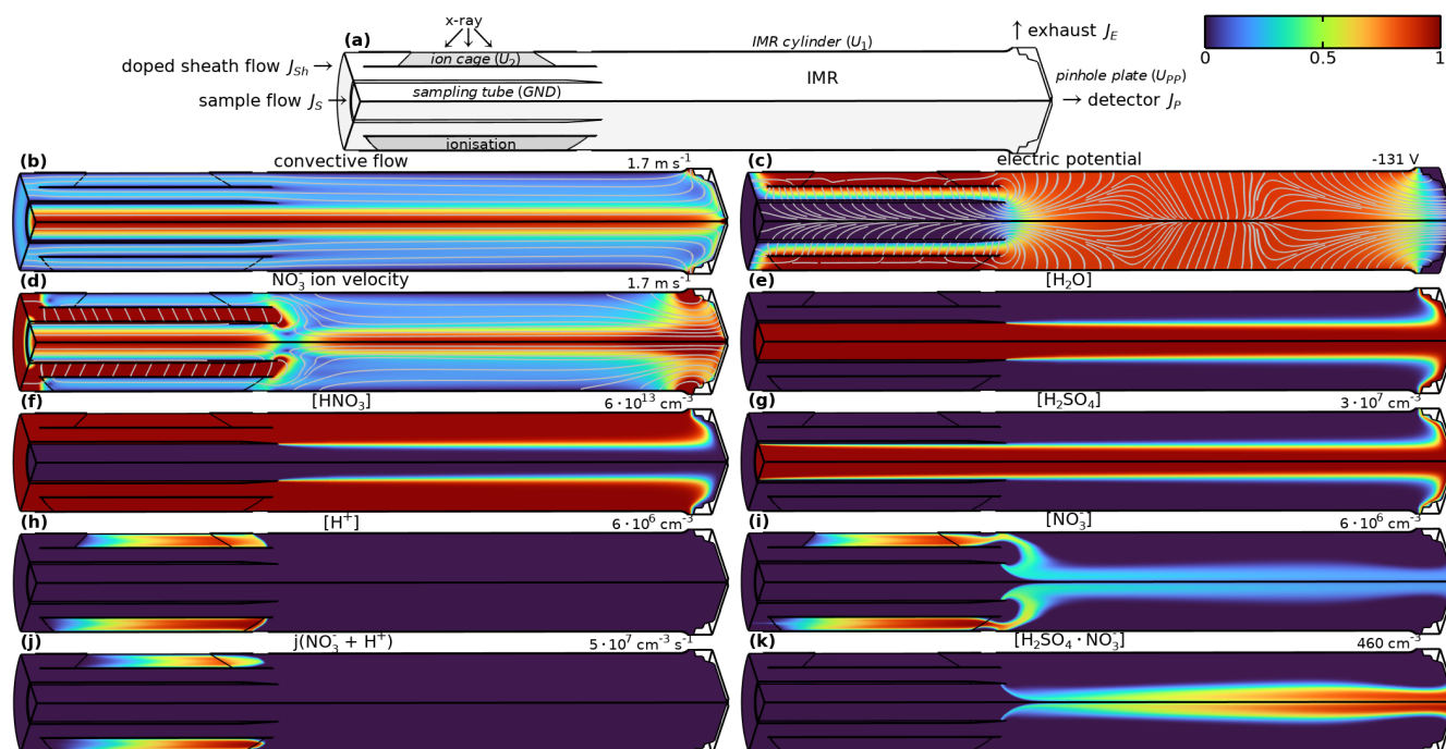
Figure 7. Physical quantities in Eisele type inlet. Only a quarter cut is shown. The colour scale ranges from 0 to the maximum described in each panel. Panel D shows the electro-advective velocity for anions with \mu = 2.4 \text{ cm}^2 \text{ V}^{-1} \text{ s}^{-1} . Used settings: U_1 = -110.7 \text{ V} , U_2 = -98.9 \text{ V} , U_{PP} = 0 \text{ V} , sheath flow 20 slpm, sample flow 10 slpm.
