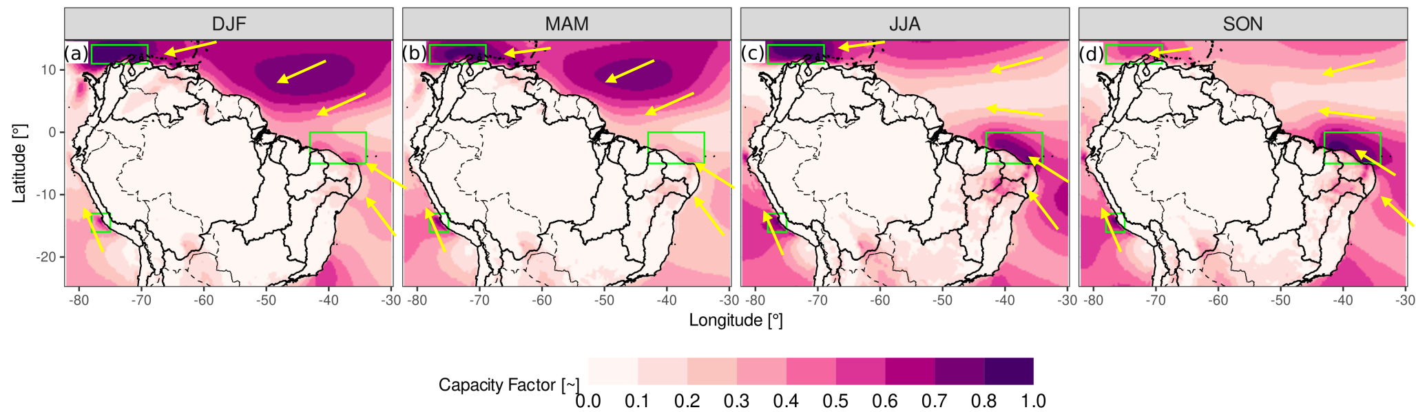
Mean seasonal Wind Capacity Factor - ERA5 (1980-2020)
