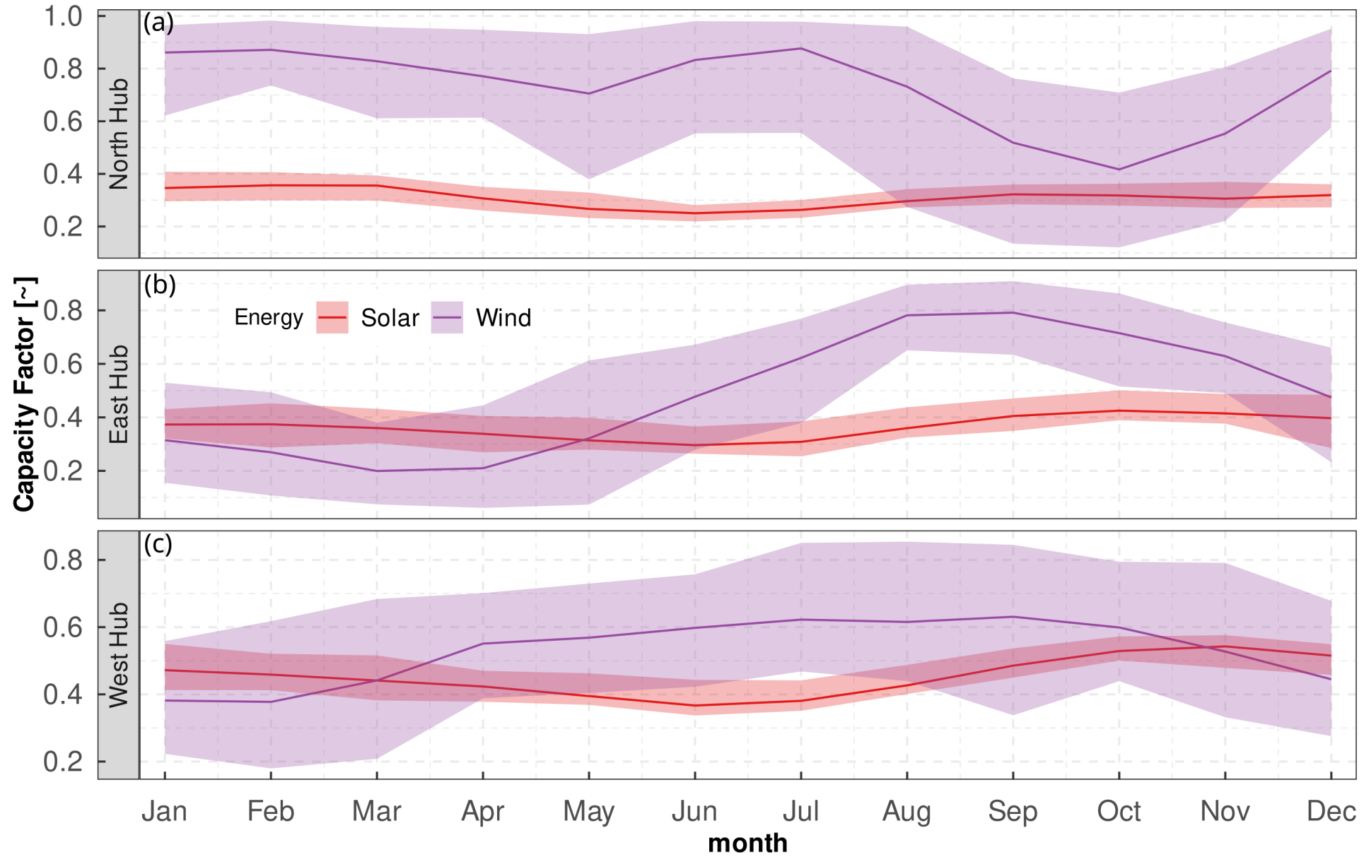
Multiannual Monthly Solar and Wind CF, maximum, mean and minimum
