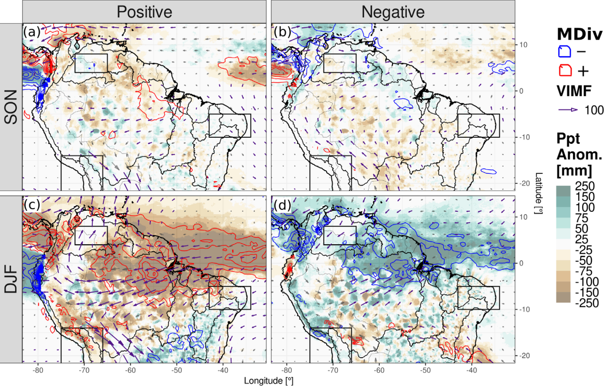
Anomaly Composite (1980-2020), |ELI| \geq 0.75 \cdot SD
