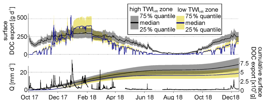
Figure 7. Absolute DOC surface export (25th, 50th and 75th percentiles) from high- \text{TWI}_{\text{HR}} ( \text{DOC}_I quality) and low- \text{TWI}_{\text{HR}} ( \text{DOC}_{II} quality) source zones. Underlying DOC concentration percentiles based on all riparian groundwater samples of each source zone. Cumulative positive DOC export (25th, 50th and 75th percentiles) from high- and low- \text{TWI}_{\text{HR}} zones are shown on the second y axis. Discharge rate ( Q ) (lower black line) is shown on the lower left vertical axis.
