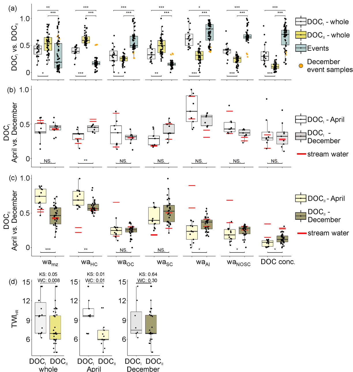
Figure 4. Comparison of FT-ICR-MS-derived weighted average (‘‘wa’’) molecular parameters wa_{mz} (mass to charge ratio), wa_{HC} (hydrogen to carbon ratio), wa_{OC} (oxygen to carbon ratio), wa_{SC} (sulfur to carbon ratio), wa_{AI} (aromaticity index) and wa_{NOSC} (nominal oxidation state of carbon) as well as DOC concentration (DOC conc.) and high-resolution TWI ( TWI_{HR} ) values of stream, DOC I and DOC II samples. (a) Boxplots of molecular parameters and DOC concentration of the DOC I and DOC II clusters. Orange dots indicate samples of one December event. (b) Boxplots of molecular parameters and DOC concentration of April and December DOC I samples and all event samples. (c) Boxplots of molecular parameters and DOC concentration of April and December DOC II samples and all event samples. Red horizontal lines in panels (b) and (c) indicate weighted averages of two April and two December stream water samples collected during the respective riparian groundwater sampling campaign. Data in panels (a–c) were min–max normalized to values between 0 and 1 for better illustration (see Table 1 for actual values). (d) Boxplots of TWI_{HR} values as affiliated to the respective wells of DOC I and DOC II samples. Wilcoxon rank sum (WC) and Kolmogorov–Smirnov (KS) test results are depicted above the squared brackets. Squared brackets above and below boxplots in (a–c) indicate the application of a KS test between two partitions. Asterisks indicate p values of the KS test (***: < 0.001; **: < 0.01; *: < 0.05; NS: not significant).
