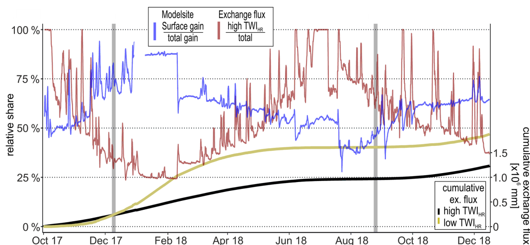
Figure 6. Share of surface runoff on total runoff generation (blue line) and of high- \text{TWI}_{\text{HR}} zone water exchange flux on total exchange flux in the model site (red). Data were smoothed to daily values for better visualization. The gap in the blue line in January 2018 is due to an ungauged flood event. Cumulative positive water exchange flux of high- \text{TWI}_{\text{HR}} (black) and low- \text{TWI}_{\text{HR}} (yellow) source zones are shown on the second vertical axis. Grey bars indicate modeling dates for a wet situation on 13 December 2017, right after an event and at dry conditions, and on 29 August 2018, amidst a longer dry period in summer (Fig. S8, Table S6).
