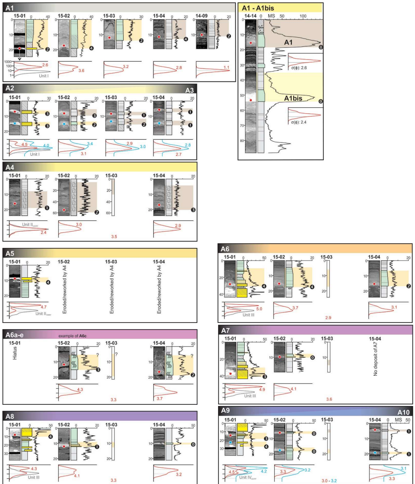
Supplementary Figure: Overview of all allochthonous deposits in piston cores 15-01, 15-02, 15-03 and 15-04, and also in gravity cores 14-09 and 14-14 for layer A1. Each individual graph shows (above, from left to right) sediment structure and thickness (CT-scan and log; in cm), magnetic susceptibility (same units and scale as in Fig. 5A), degree of basal erosion (ranging between 0 and 4; white numbers on black background), and (below) basal grain size and sorting (sample location indicated by red or blue dot; sorting in \sigma(\phi) in red or blue numbers) compared to background.
