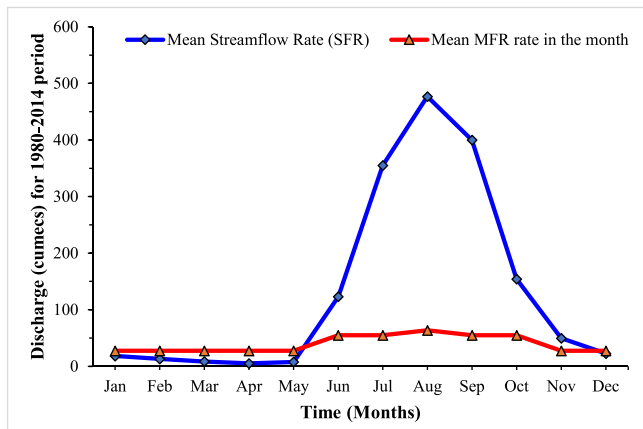
Fig. 5. Demonstration of observed monthly variation of Streamflow Rate (SFR) against Minimum in-stream Flow Requirement (MFR) for Jaraikela catchment using Tennant's method [Note: Here, each month is representative of the mean discharge over the period 1980–2014 (35 years)].
