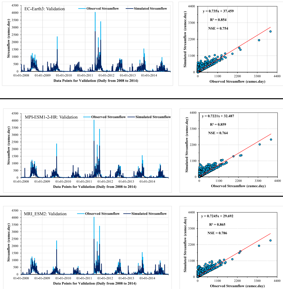
Fig. 4. Comparison between observed and simulated daily streamflow (obtained using the HCCS model) for the Jaraikela catchment during the validation period (2008–2014) for the three General Circulation Models (GCMs viz., EC-Earth3, MPI-ESM1-2-HR, and MRI-ESM2) output ensembles using time series plots (left-side) and scatter plots (right-side) [In the scatter plots, the solid black line shows the 45° line (1:1; line of perfect simulation), and the other line shows the best-fit line for the scatter plots].
