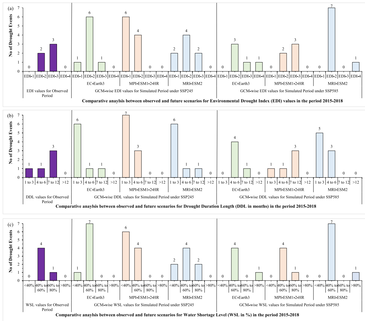
Fig. 10. Comparative analysis for the numbers of environmental drought events with different EDI values [as shown in (a)] and for different lengths of the drought (DDL) period [as shown in (b)] and for different levels of water shortage (WSL) [as shown in (c)] between the observed datasets and the three General Circulation Models (GCMs viz., EC-Earth3, MPI ESM1-2-HR, and MRI-ESM2) under the two future scenarios [SSP245 (left-side) and SSP585 (right-side)] for the period 2015–2018 at Jaraikela catchment [Note: The observed data for Jaraikela catchment is available only for the period 1980–2018 in the public domain; thus, the present study does not compare the observed findings with the entire first future period (i.e., 2015–2022) but is limited to comparing it with 2015–2018 period].
