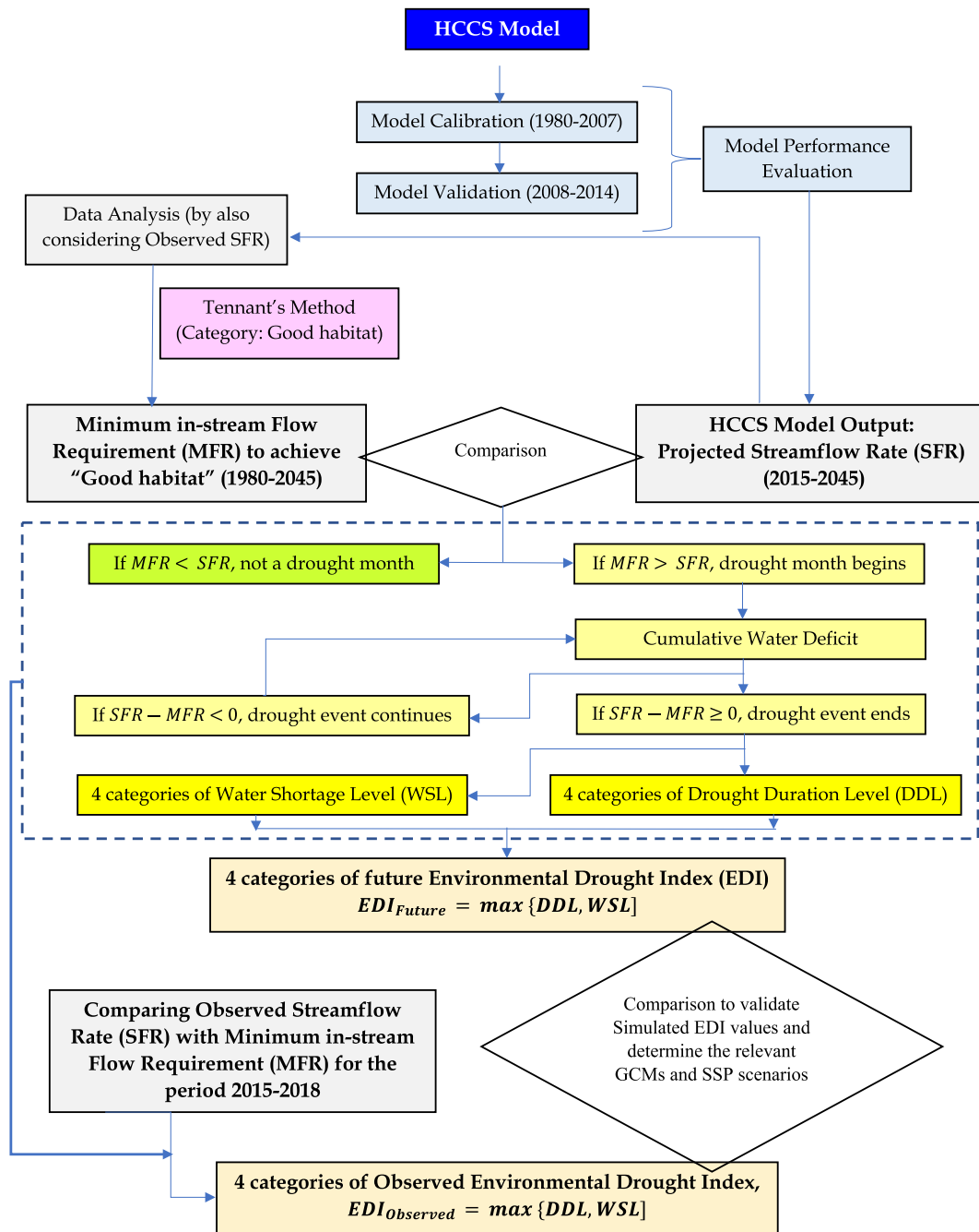
Fig. 1. Methodological flowchart for the development of the heuristic method and the Environmental Drought Index (EDI).
