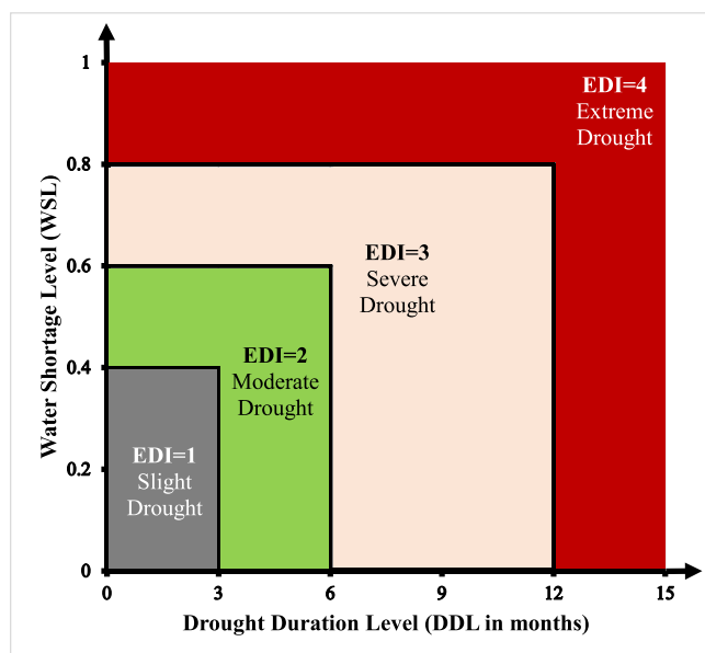
Fig. 2. Categorization of various EDI values based on different levels of drought duration (DDL) and water shortage (WSL), outlining their respective definitions and ranges [developed after Shi et al. (2018)].
