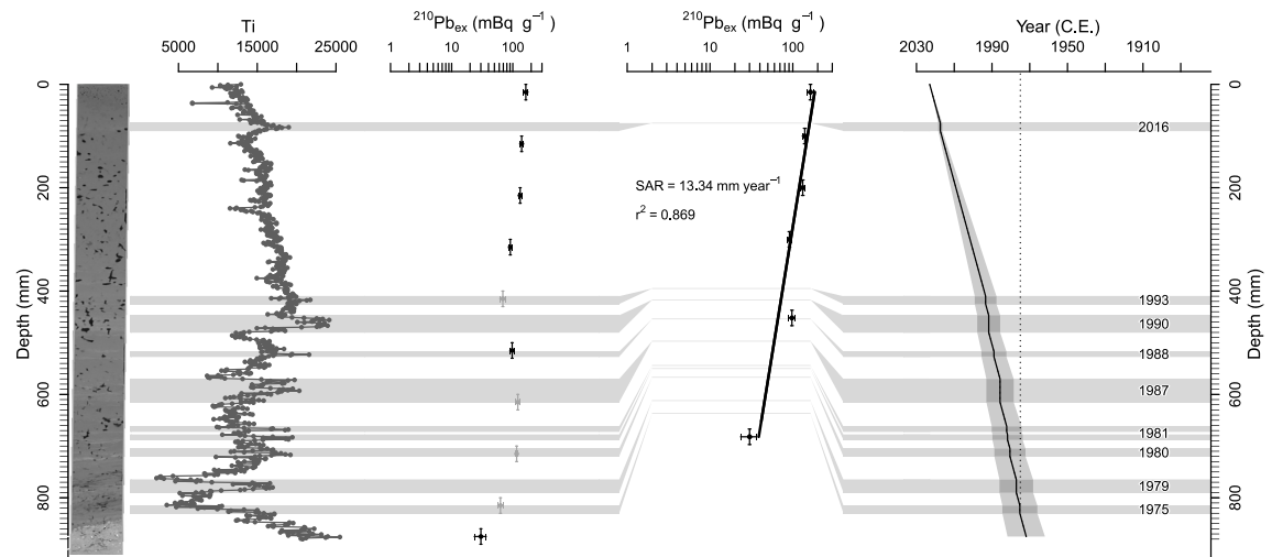
Fig. S4. Age-depth model for the DUC03 core.
