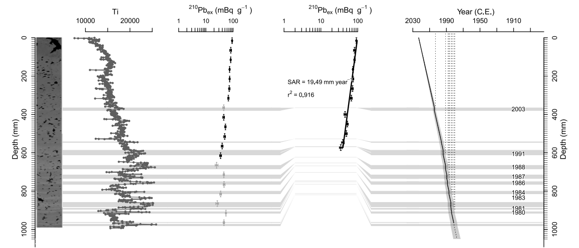
Fig. S5. Age-depth model for the DUC04 core.
