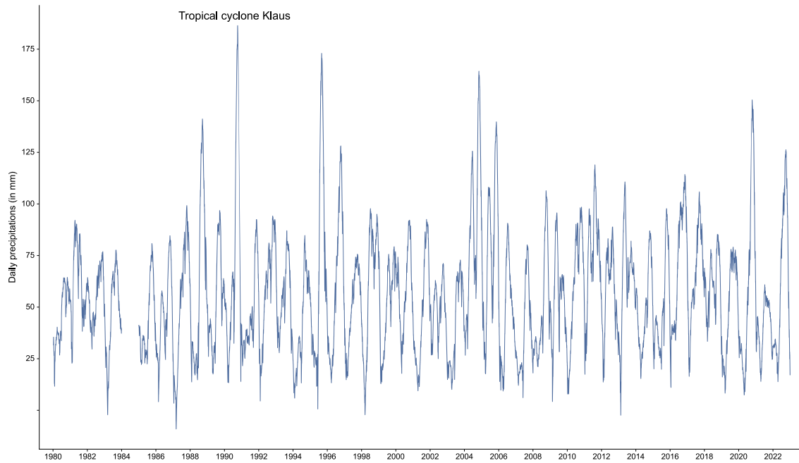
Fig. S1. Daily precipitations at the Saint-Espirit station (source: MétéoFrance) between 1980 and 2022.
