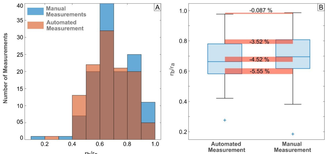
Figure 2. Manual vs Automated Measurement from Photograph from River 4. (A) Histogram. (B) Box-whisker plots.
