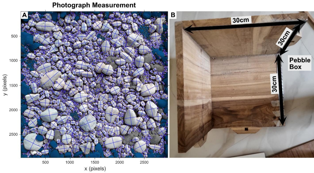
Figure 1. Gravel Axes Measurements. (A) Photograph measurement using BASEGRAIN (Detertand Weitbrecht, 2013). (B) Manual Measurement using Pebble Box (Ibbeken and Denzer, 1988; Bunte and Apt, 2001).
